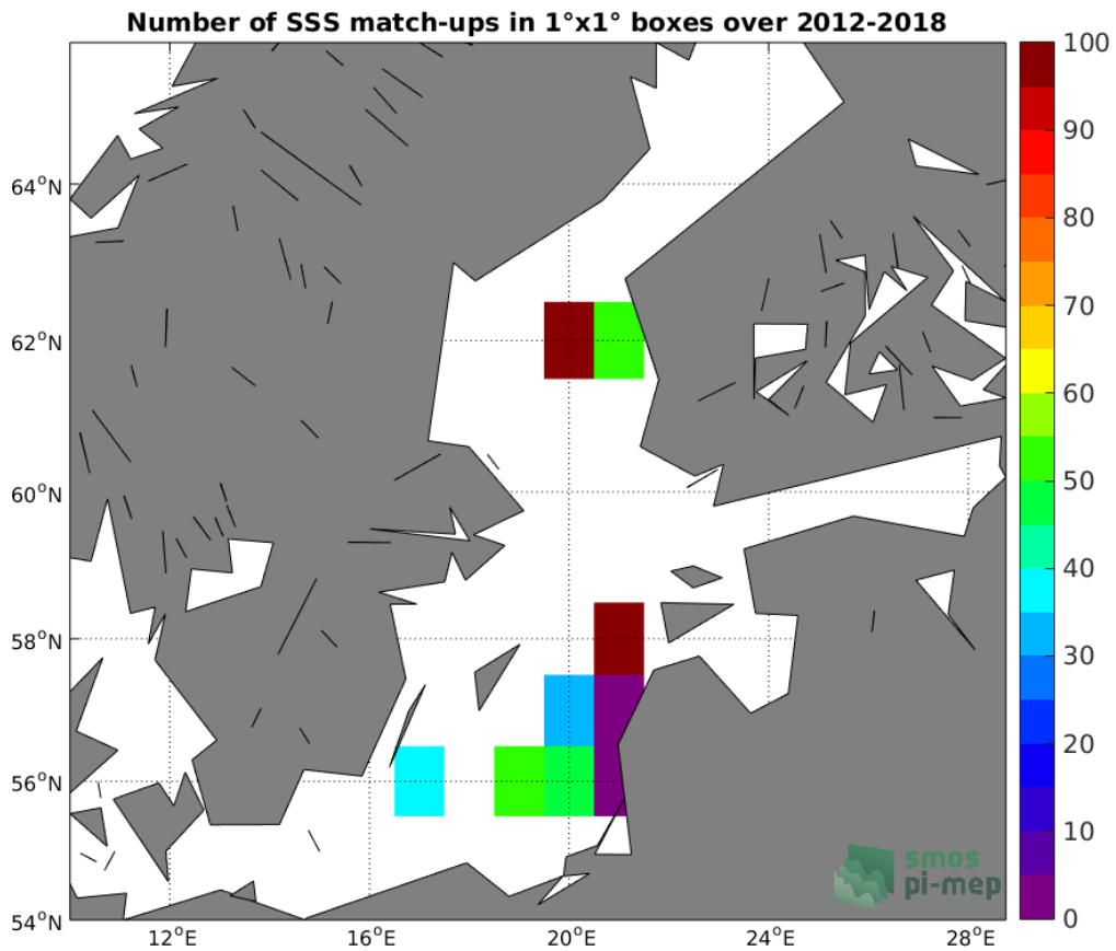
Figure 4: Number of SSS match-ups between Argo SSS and the CCI L4 Merged-OI v1.8 - 30-day running (ESA) SSS product for the Baltic Sea Pi-MEP region over 1°x1° boxes and for the full satellite product period.
