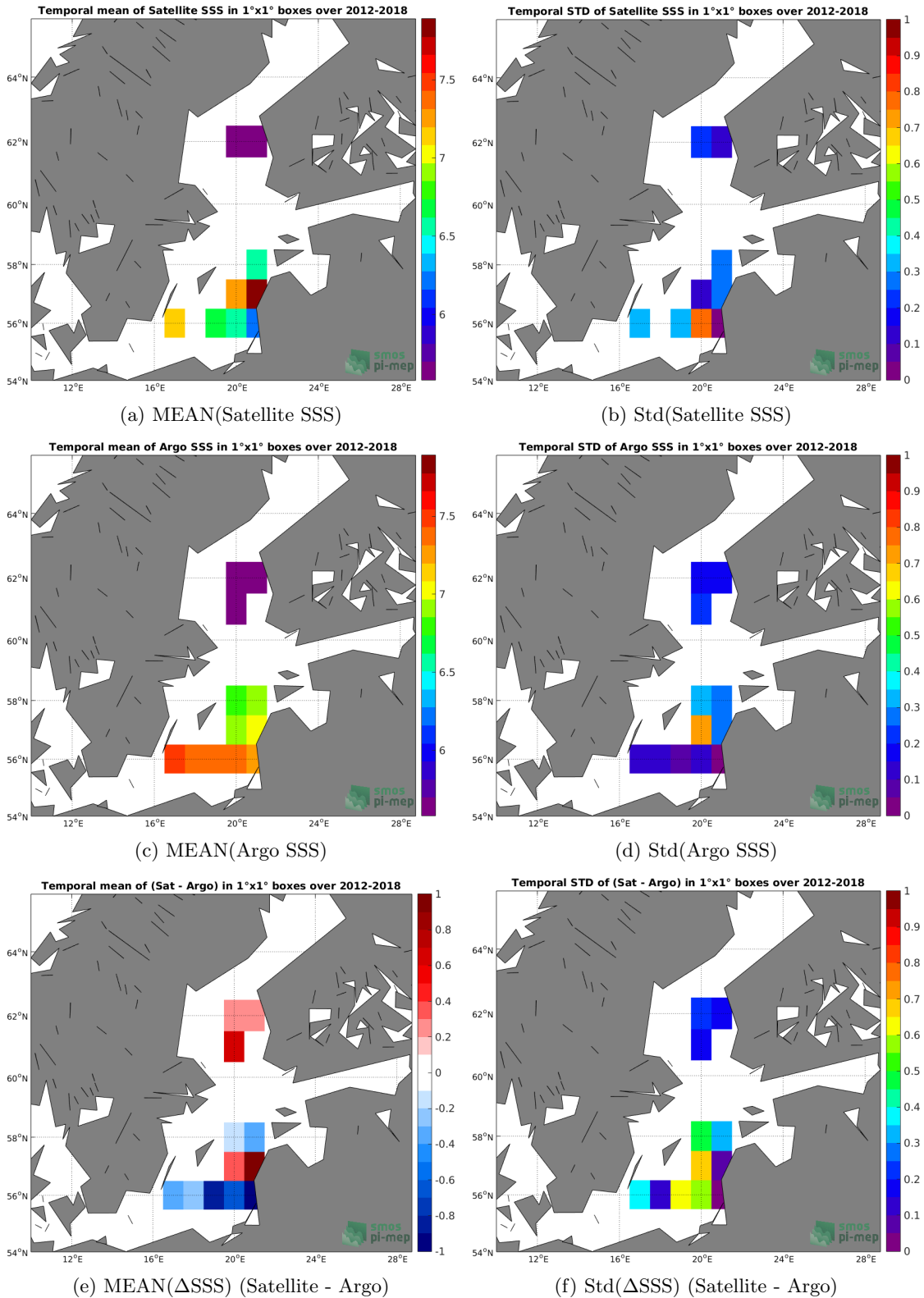
Figure 6: Temporal mean (left) and Std (right) of SSS from CCI L4 Merged-OI v1.8 - 30-day running (ESA) (top), Argo (middle), and of \Delta SSS (Satellite - Argo). Only match-up pairs are used to generate these maps.
