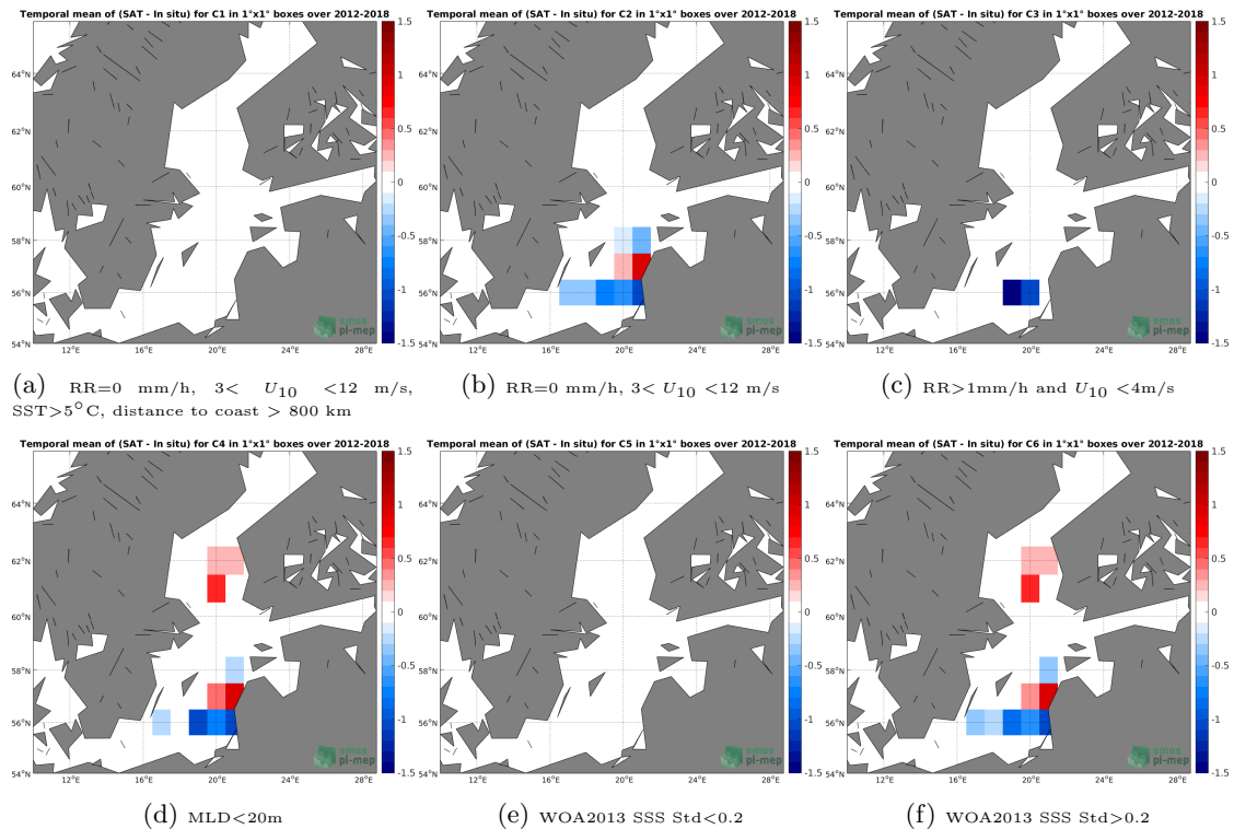
Figure 12: Temporal mean gridded over spatial boxes of size 1^{\circ}\times 1^{\circ} of \Delta\text{SSS} (CCI L4 Merged-OI v1.8 - 30-day running (ESA) - Argo) for 6 different subdatasets corresponding to:RR=0 mm/h, 3 < U_{10} < 12 m/s, SST >5^{\circ}\text{C} , distance to coast > 800 km (a), RR=0 mm/h, 3 < U_{10} < 12 m/s (b), RR >1\text{mm/h} and U_{10} < 4\text{m/s} (c),MLD <20\text{m} (d),WOA2013 SSS Std <0.2 (e),WOA2013 SSS Std >0.2 (f).
