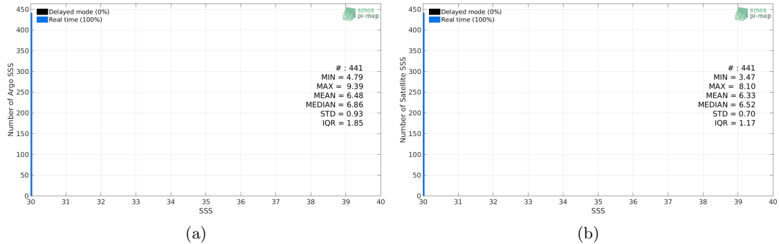
Figure 2: Histograms of SSS from Argo (a) and CCI L4 Merged-OI v1.8 - 30-day running (ESA) (b) considering all match-up pairs per bins of 0.1 over the Baltic Sea Pi-MEP region and for the full satellite product period.
