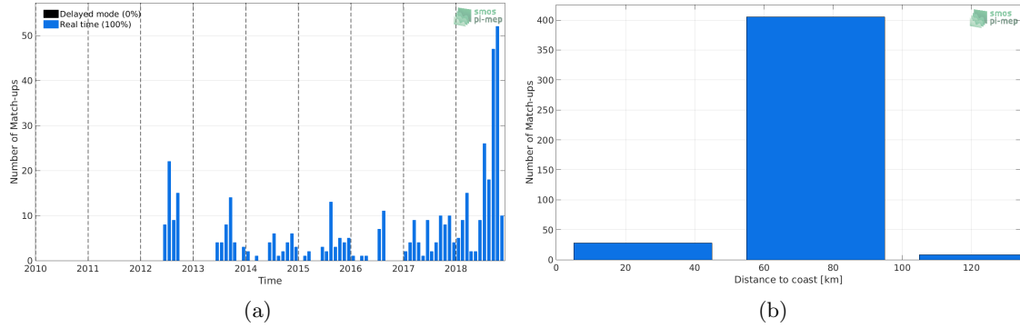
Figure 1: Number of match-ups between Argo and CCI L4 Merged-OI v1.8 - 30-day running (ESA) SSS as a function of time (a) and as function of the distance to coast (b) over the Baltic Sea Pi-MEP region and for the full satellite product period.
