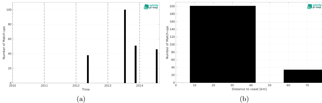
Figure 2: Number of match-ups between TSG (LEGOS-DM) and Aquarius SSS L3 OR v5 - 7-Day running (NASA-GSFC) SSS as a function of time (a) and as function of the distance to coast (b) over the Baltic Sea Pi-MEP region and for the full satellite product period.
