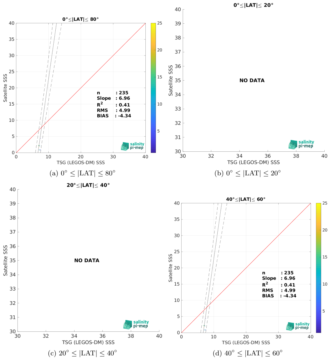
Figure 10: Contour maps of the concentration of Aquarius SSS L3 OR v5 - 7-Day running (NASA-GSFC) SSS (y-axis) versus TSG (LEGOS-DM) SSS (x-axis) at match-up pairs for different latitude bands. For each plot, the red line shows x=y . The black thin and dashed lines indicate a linear fit through the data cloud and the \pm 95\% confidence levels, respectively. The number match-up pairs n , the slope and R^2 coefficient of the linear fit, the root mean square (RMS) and the mean bias between satellite and in situ data are indicated for each latitude band in each plots.
