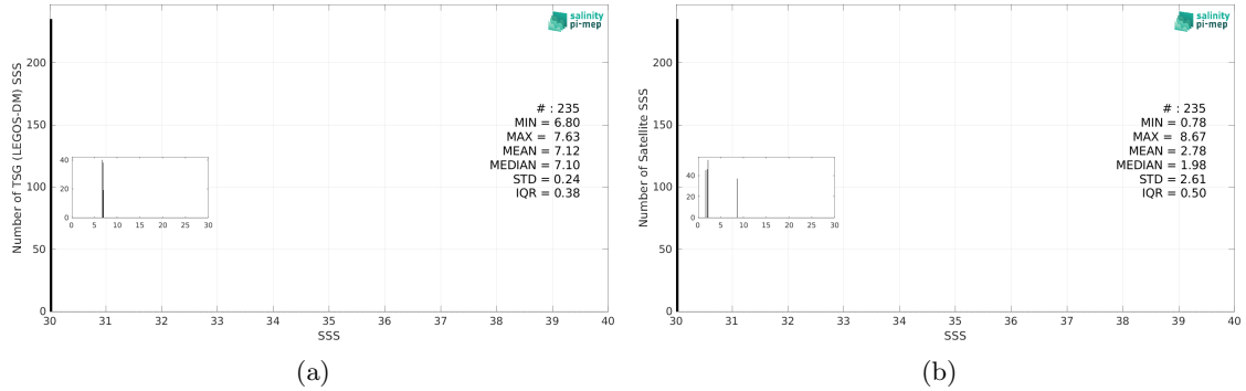
Figure 3: Histograms of SSS from TSG (LEGOS-DM) (a) and Aquarius SSS L3 OR v5 - 7-Day running (NASA-GSFC) (b) considering all match-up pairs per bins of 0.1 over the Baltic Sea Pi-MEP region and for the full satellite product period.
