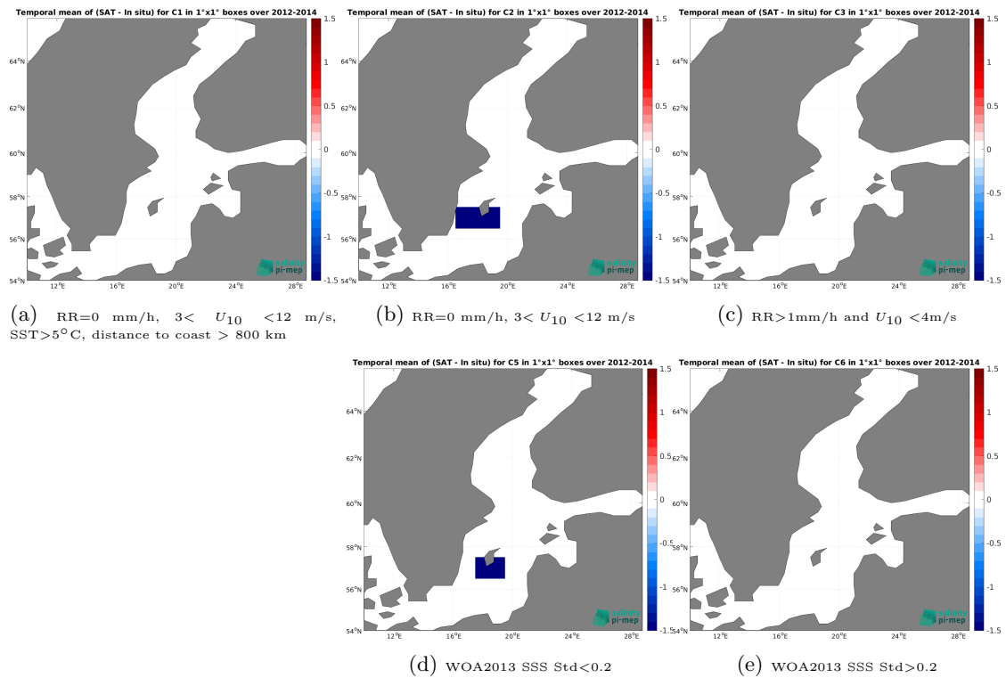
Figure 14: Temporal mean gridded over spatial boxes of size 1^\circ \times 1^\circ of \Delta SSS (Aquarius SSS L3 OR v5 - 7-Day running (NASA-GSFC) - TSG (LEGOS-DM)) for 5 different subdatasets corresponding to:RR=0 mm/h, 3 < U_{10} < 12 m/s, SST >5^\circ\text{C} , distance to coast > 800 km (a), RR=0 mm/h, 3 < U_{10} < 12 m/s (b), RR >1 mm/h and U_{10} < 4 m/s (c), WOA2013 SSS Std <0.2 (d), WOA2013 SSS Std >0.2 (e).
