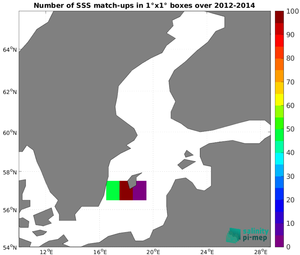
Figure 5: Number of SSS match-ups between TSG (LEGOS-DM) SSS and the Aquarius SSS L3 OR v5 - 7-Day running (NASA-GSFC) SSS product for the Baltic Sea Pi-MEP region over 1^\circ \times 1^\circ boxes and for the full satellite product period.
