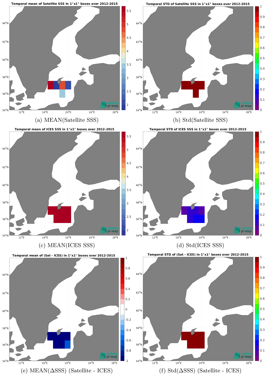
Figure 7: Temporal mean (left) and Std (right) of SSS from Aquarius SSS L3 OR v5 - 7-Day running (NASA-GSFC) (top), ICES (middle), and of \Delta SSS (Satellite - ICES). Only match-up pairs are used to generate these maps.
