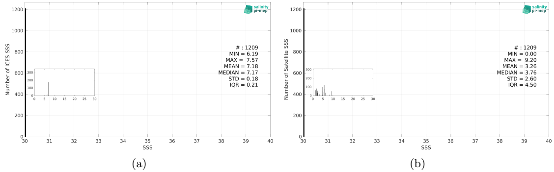
Figure 3: Histograms of SSS from ICES (a) and Aquarius SSS L3 OR v5 - 7-Day running (NASA-GSFC) (b) considering all match-up pairs per bins of 0.1 over the Baltic Sea Pi-MEP region and for the full satellite product period.
