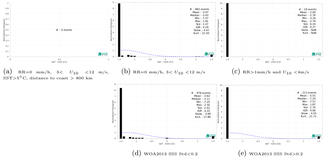
Figure 15: Normalized histogram of \Delta SSS (Aquarius SSS L3 OR v5 - 7-Day running (NASA-GSFC) - ICES) for 5 different subdatasets corresponding to: RR=0 mm/h, 3 < U_{10} < 12 m/s, SST >5^{\circ} C, distance to coast > 800 km (a), RR=0 mm/h, 3 < U_{10} < 12 m/s (b), RR >1 mm/h and U_{10} < 4 m/s (c), WOA2013 SSS Std <0.2 (d), WOA2013 SSS Std >0.2 (e).
