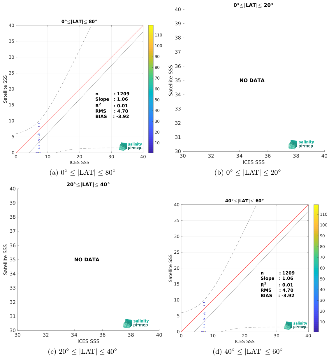
Figure 10: Contour maps of the concentration of Aquarius SSS L3 OR v5 - 7-Day running (NASA-GSFC) SSS (y-axis) versus ICES SSS (x-axis) at match-up pairs for different latitude bands. For each plot, the red line shows x=y . The black thin and dashed lines indicate a linear fit through the data cloud and the \pm 95\% confidence levels, respectively. The number match-up pairs n , the slope and R^2 coefficient of the linear fit, the root mean square (RMS) and the mean bias between satellite and in situ data are indicated for each latitude band in each plots.
