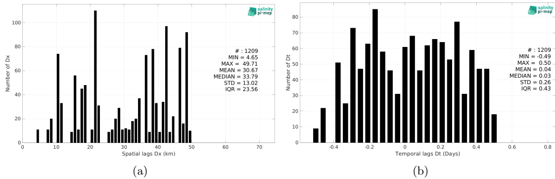
Figure 6: Histograms of the spatial (a) and temporal (b) lags between the location/time of the ICES measurement and the date of the corresponding Aquarius SSS L3 OR v5 - 7-Day running (NASA-GSFC) SSS pixel.
