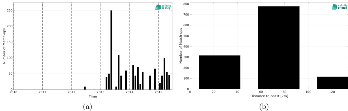
Figure 2: Number of match-ups between ICES and Aquarius SSS L3 OR v5 - 7-Day running (NASA-GSFC) SSS as a function of time (a) and as function of the distance to coast (b) over the Baltic Sea Pi-MEP region and for the full satellite product period.
