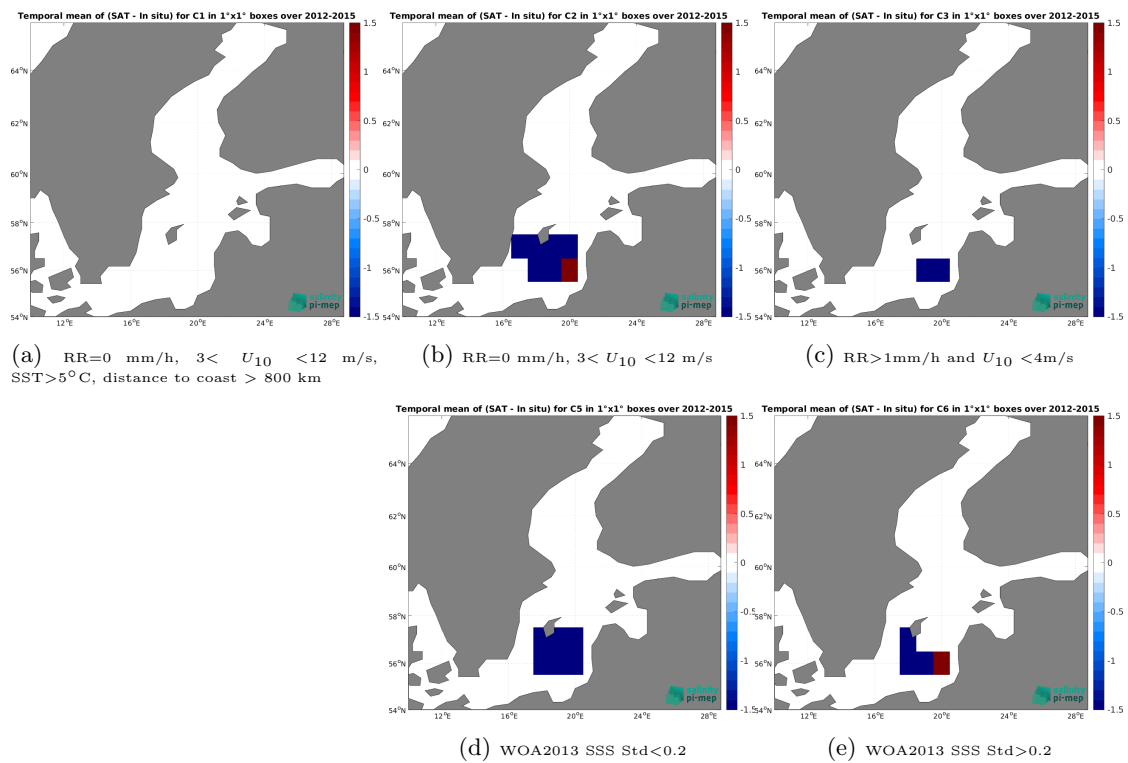
Figure 14: Temporal mean gridded over spatial boxes of size 1^\circ \times 1^\circ of \Delta SSS (Aquarius SSS L3 OR v5 - 7-Day running (NASA-GSFC) - ICES) for 5 different subdatasets corresponding to: RR=0 mm/h, 3 < U_{10} < 12 m/s, SST > 5^\circ\text{C} , distance to coast > 800 km (a), RR=0 mm/h, 3 < U_{10} < 12 m/s (b), RR > 1 mm/h and U_{10} < 4 m/s (c), WOA2013 SSS Std < 0.2 (d), WOA2013 SSS Std > 0.2 (e).
