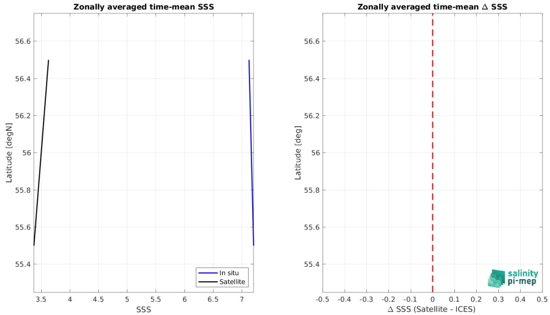
Figure 9: Left panel: Zonal mean SSS from Aquarius SSS L3 OR v5 - 7-Day running (NASA-GSFC) satellite product (black) and from ICES (blue). Right panel: Zonal mean of \Delta SSS (Satellite - ICES) for all the collected Pi-MEP match-up pairs estimated over the full satellite product period.
