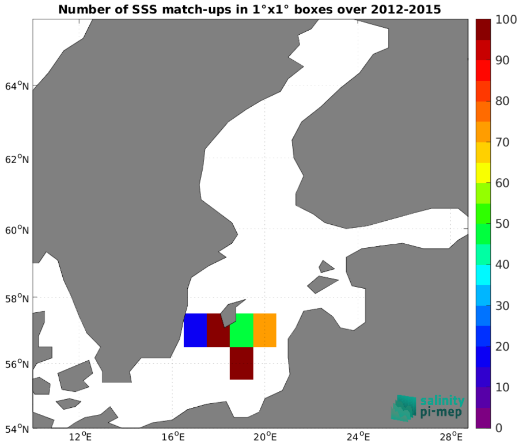
Figure 5: Number of SSS match-ups between ICES SSS and the Aquarius SSS L3 OR v5 - 7-Day running (NASA-GSFC) SSS product for the Baltic Sea Pi-MEP region over 1^\circ \times 1^\circ boxes and for the full satellite product period.
