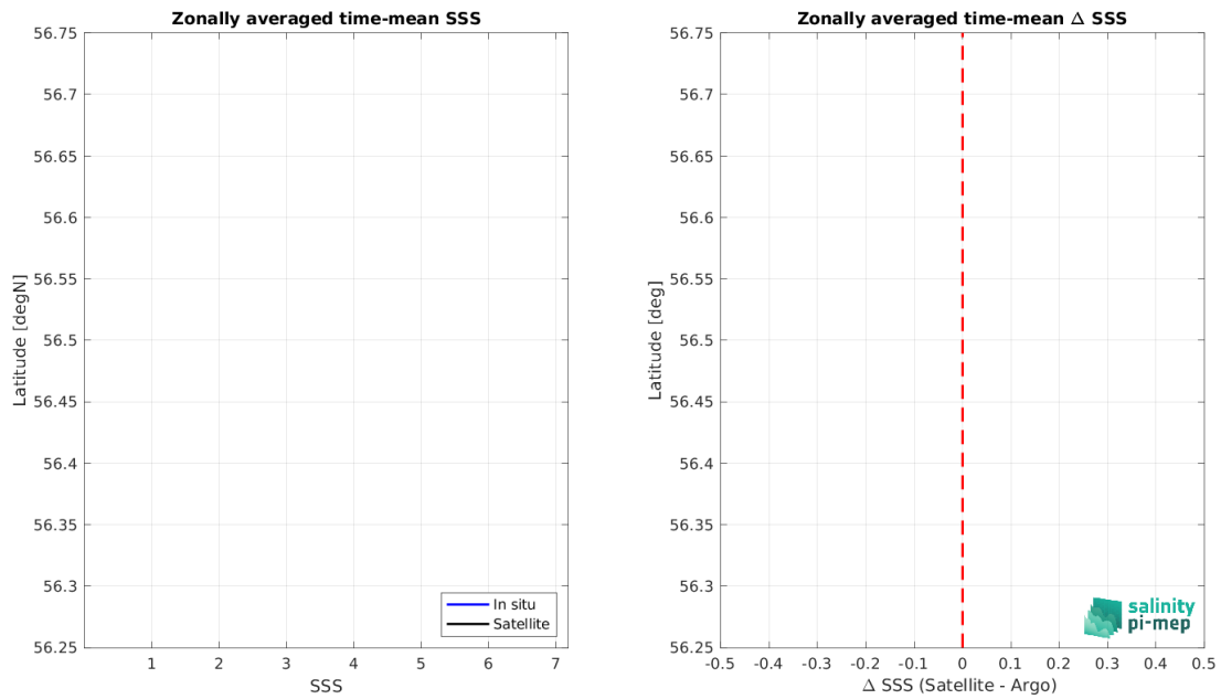
Figure 7: Left panel: Zonal mean SSS from Aquarius SSS L3 OR v5 - 7-Day running (NASA-GSFC) satellite product (black) and from Argo (blue). Right panel: Zonal mean of \Delta SSS (Satellite - Argo) for all the collected Pi-MEP match-up pairs estimated over the full satellite product period.
