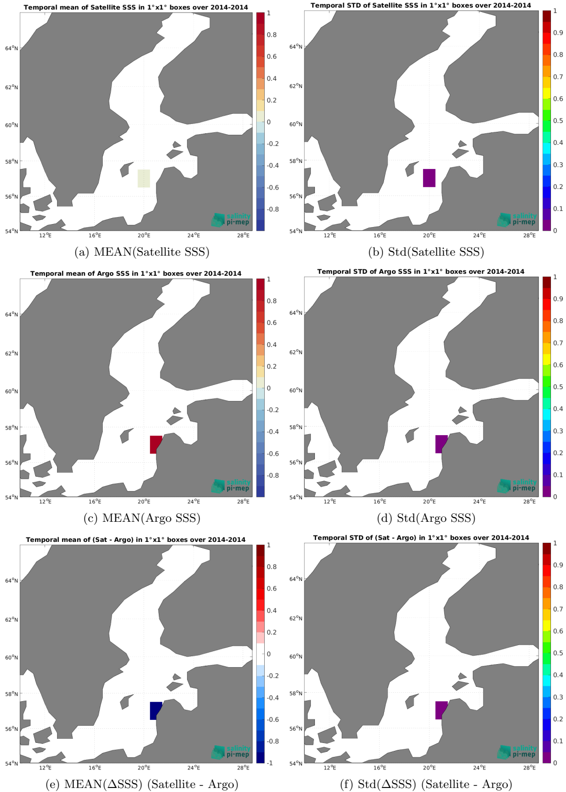
Figure 5: Temporal mean (left) and Std (right) of SSS from Aquarius SSS L3 OR v5 - 7-Day running (NASA-GSFC) (top), Argo (middle), and of \Delta SSS (Satellite - Argo). Only match-up pairs are used to generate these maps.
