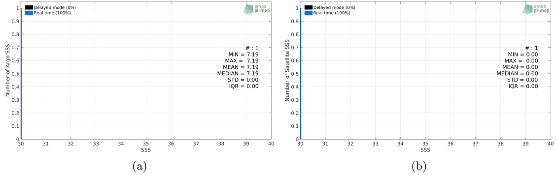
Figure 2: Histograms of SSS from Argo (a) and Aquarius SSS L3 OR v5 - 7-Day running (NASA-GSFC) (b) considering all match-up pairs per bins of 0.1 over the Baltic Sea Pi-MEP region and for the full satellite product period.
