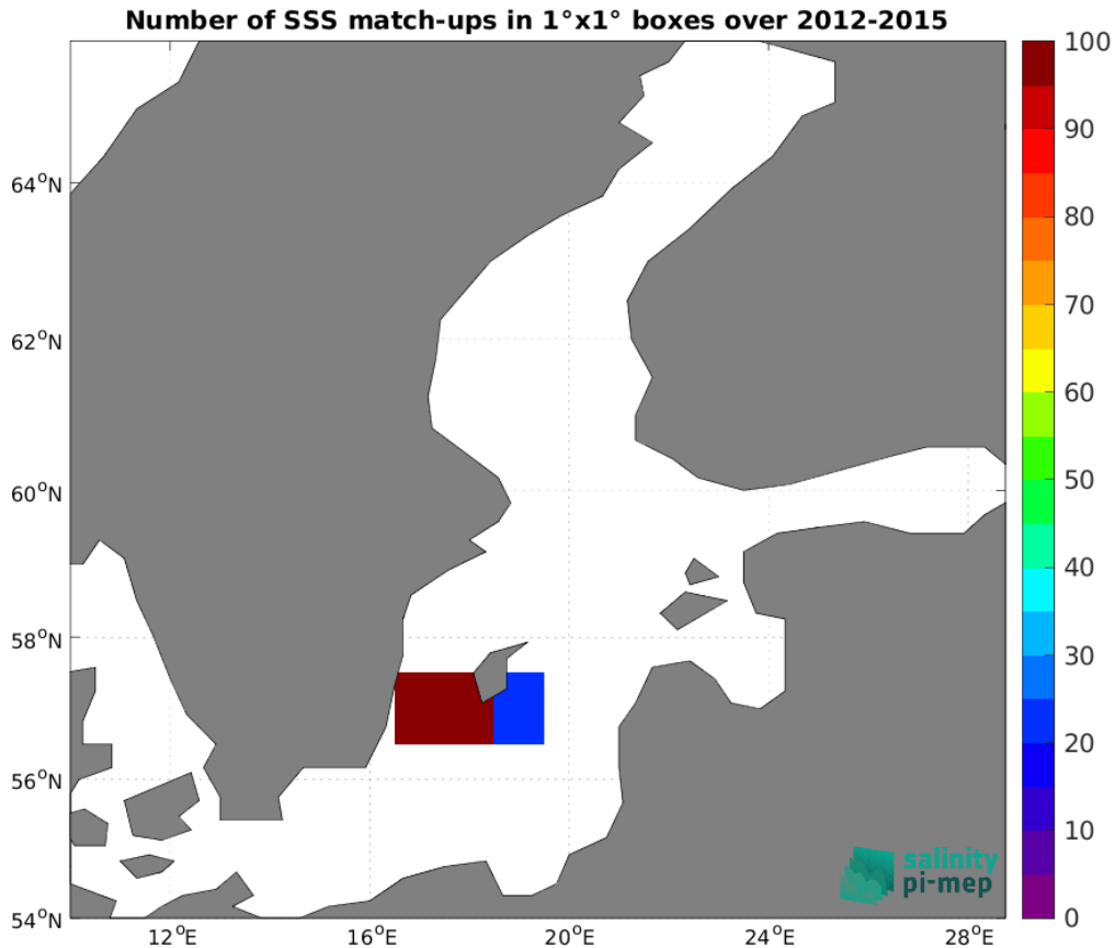
Figure 5: Number of SSS match-ups between TSG (LEGOS-DM) SSS and the Aquarius SSS L3 OR v5 - 7-Day running - Rain mask (NASA-GSFC) SSS product for the Baltic Sea Pi-MEP region over 1^\circ \times 1^\circ boxes and for the full satellite product period.
