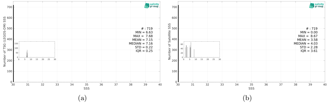
Figure 3: Histograms of SSS from TSG (LEGOS-DM) (a) and Aquarius SSS L3 OR v5 - 7-Day running - Rain mask (NASA-GSFC) (b) considering all match-up pairs per bins of 0.1 over the Baltic Sea Pi-MEP region and for the full satellite product period.
