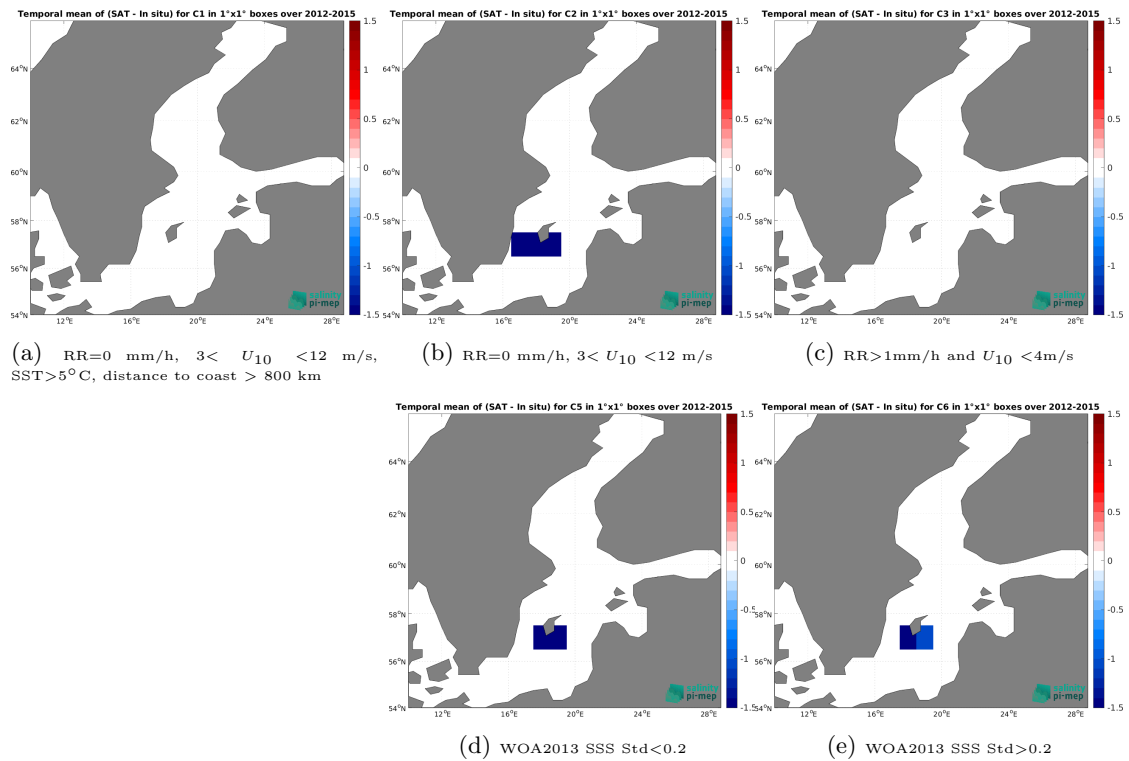
Figure 14: Temporal mean gridded over spatial boxes of size 1^\circ \times 1^\circ of \Delta SSS (Aquarius SSS L3 OR v5 - 7-Day running - Rain mask (NASA-GSFC) - TSG (LEGOS-DM)) for 5 different subdatasets corresponding to:RR=0 mm/h, 3 < U_{10} < 12 m/s, SST >5^\circ\text{C} , distance to coast > 800 km (a), RR=0 mm/h, 3 < U_{10} < 12 m/s (b), RR >1 mm/h and U_{10} < 4 m/s (c), WOA2013 SSS Std <0.2 (d), WOA2013 SSS Std >0.2 (e).
