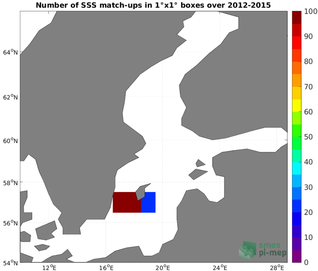
Figure 4: Number of SSS match-ups between TSG (LEGOS-DM) SSS and the Aquarius SSS L3 OR v5 - 7-Day running - Rain mask (NASA-GSFC) SSS product for the Baltic Sea Pi-MEP region over 1^\circ \times 1^\circ boxes and for the full satellite product period.
