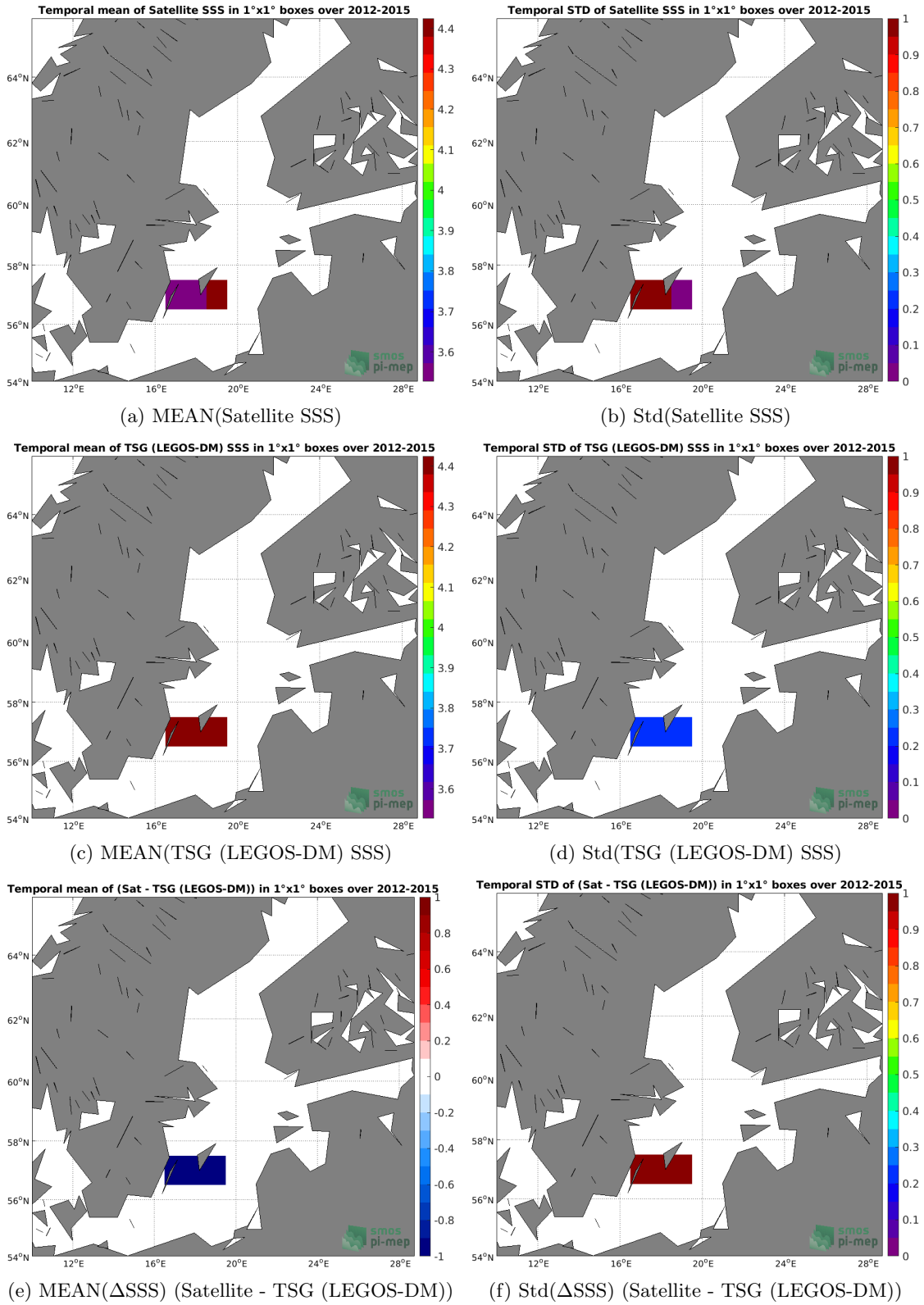
Figure 6: Temporal mean (left) and Std (right) of SSS from Aquarius SSS L3 OR v5 - 7-Day running - Rain mask (NASA-GSFC) (top), TSG 2 (LEGOS-DM) (middle), and of \Delta SSS (Satellite - TSG (LEGOS-DM)). Only match-up pairs are used to generate these maps.
