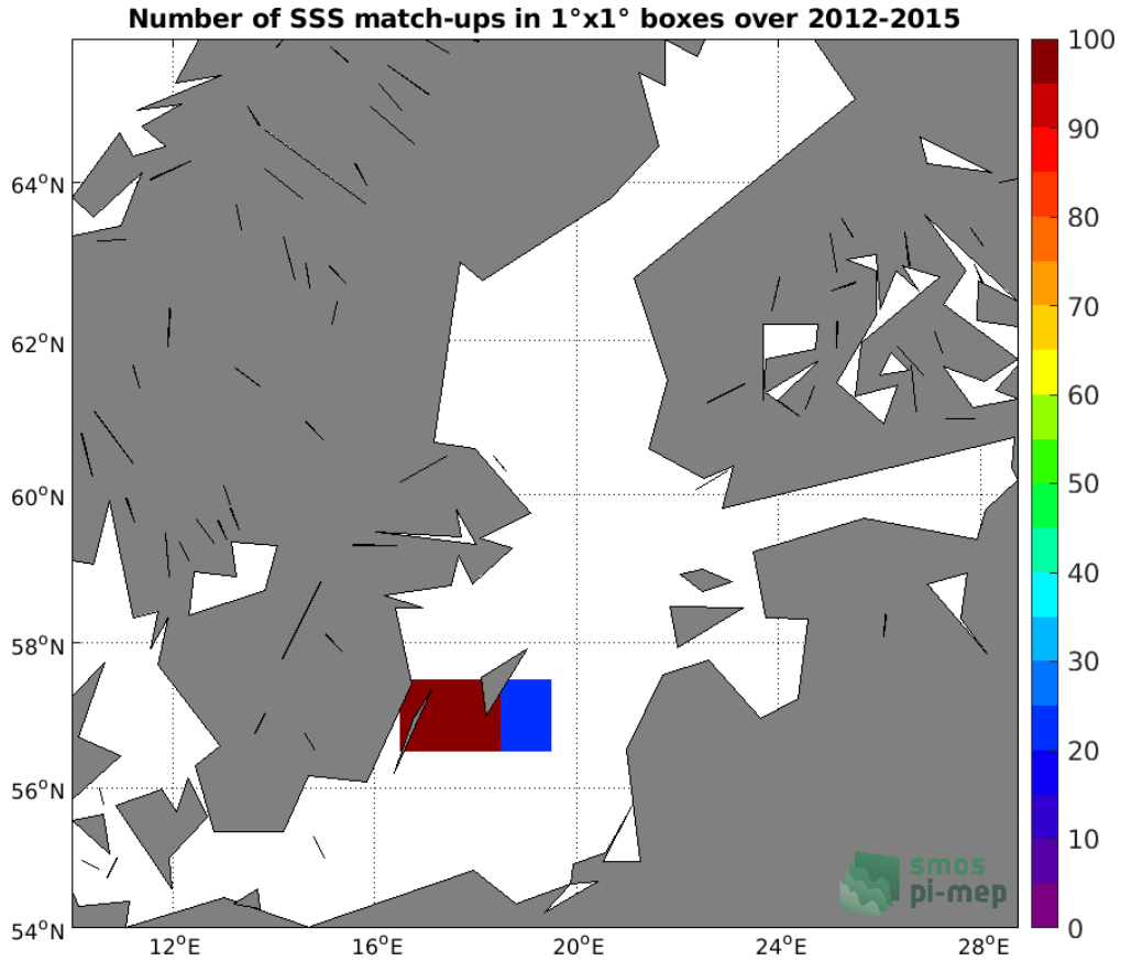
Figure 4: Number of SSS match-ups between TSG (LEGOS-DM) SSS and the Aquarius SSS L3 OR v5 - 7-Day running - Rain mask (NASA-GSFC) SSS product for the Baltic Sea Pi-MEP region over 1°×1° boxes and for the full satellite product period.
