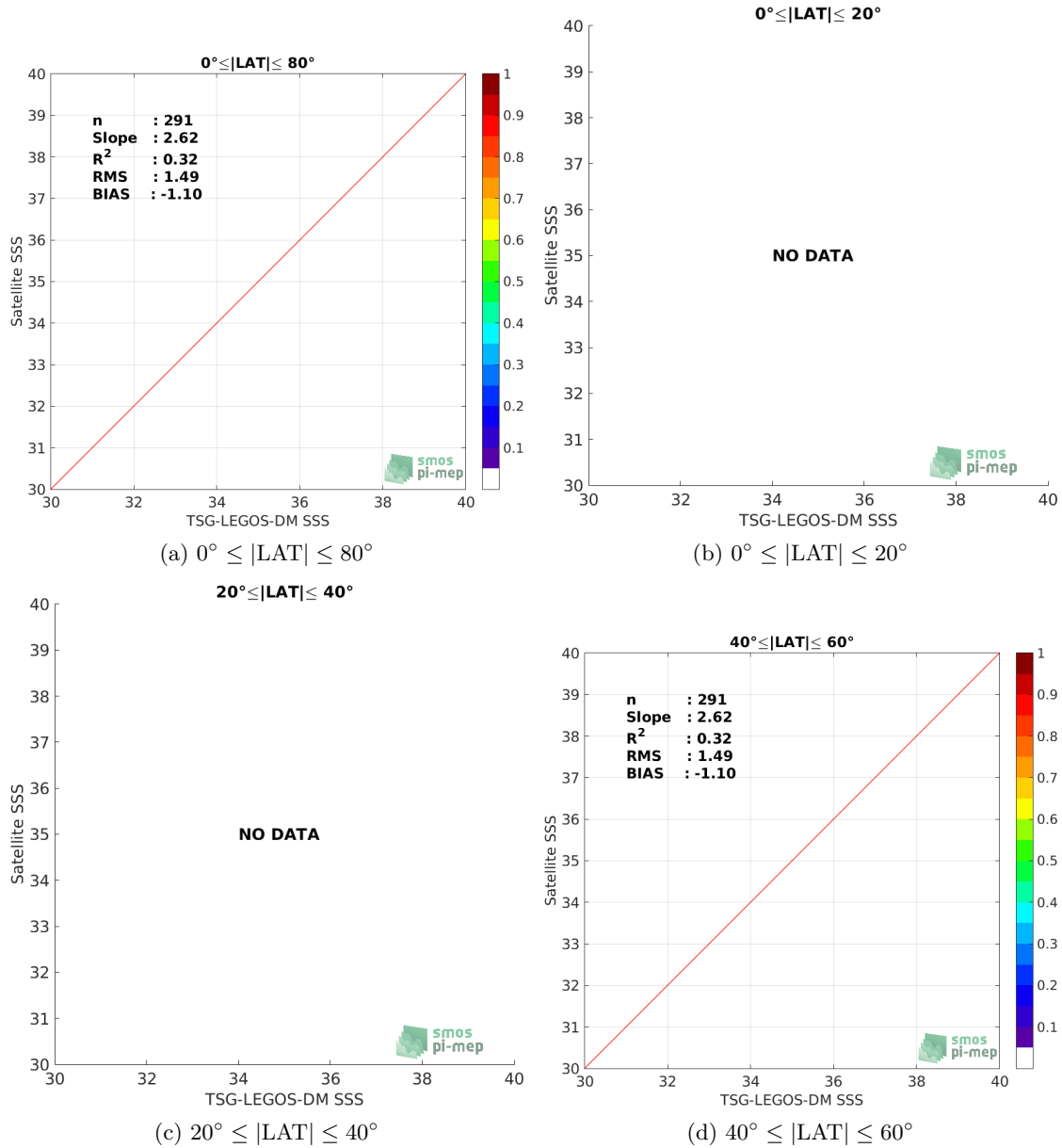
Figure 9: Contour maps of the concentration of Aquarius-L3-OR-V5-7DAY-RUNNING-RAIN-MASK-1DEG SSS ( y -axis) versus TSG-LEGOS-DM SSS ( x -axis) at match-up pairs for different latitude bands. For each plot, the red line shows x=y . The black thin and dashed lines indicate a linear fit through the data cloud and the \pm 95\% confidence levels, respectively. The number match-up pairs n , the slope and R^2 coefficient of the linear fit, the root mean square (RMS) and the mean bias between satellite and in situ data are indicated for each latitude band in each plots.
