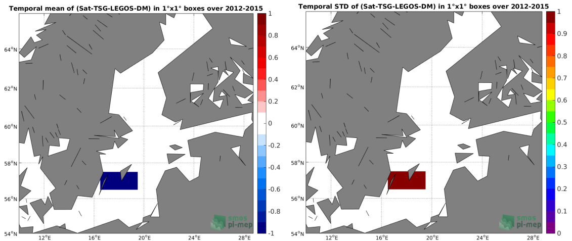
(e) MEAN( \Delta SSS) (Satellite - TSG-LEGOS-DM)
