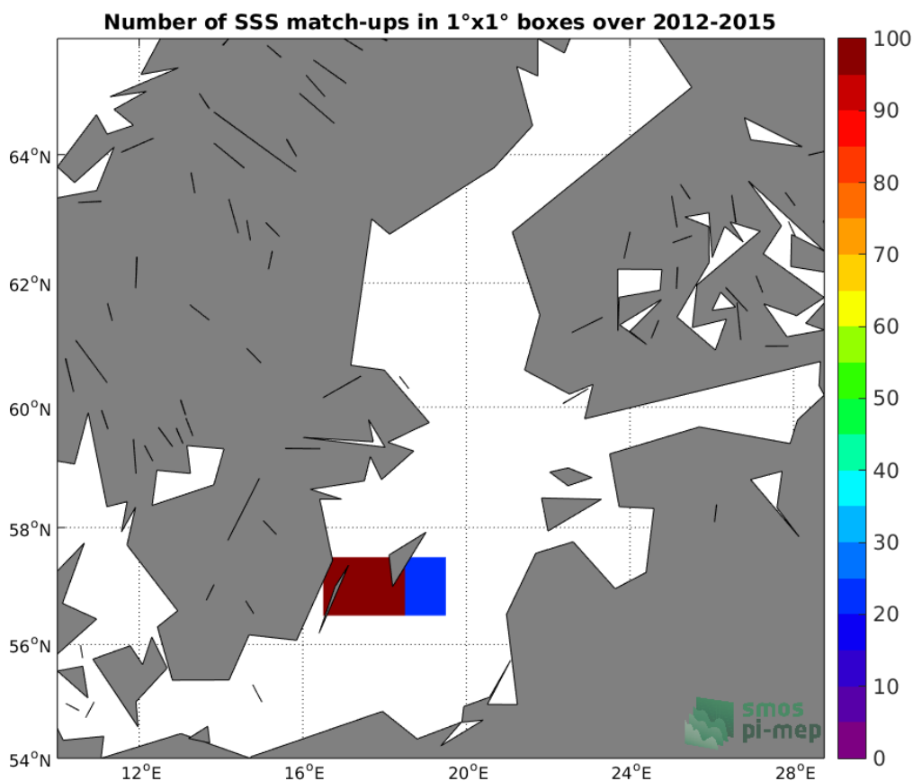
Figure 4: Number of SSS match-ups between TSG-LEGOS-DM SSS and the Aquarius-L3-OR-V5-7DAY-RUNNING-RAIN-MASK-1DEG SSS product for the Baltic Sea Pi-MEP region over 1°x1° boxes and for the full satellite product period.
