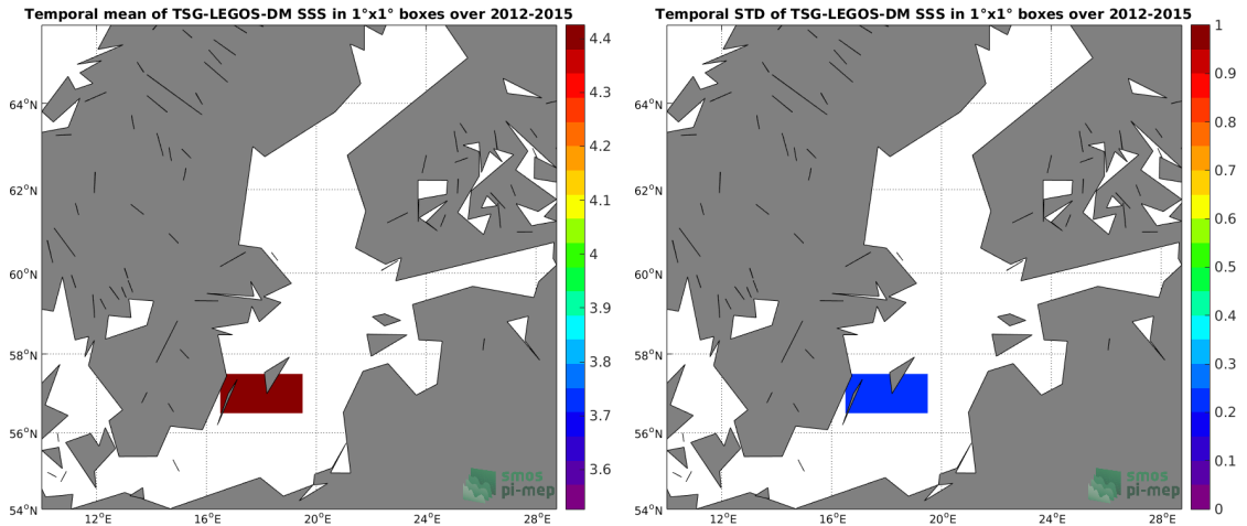
(c) MEAN(TSG-LEGOS-DM SSS)
