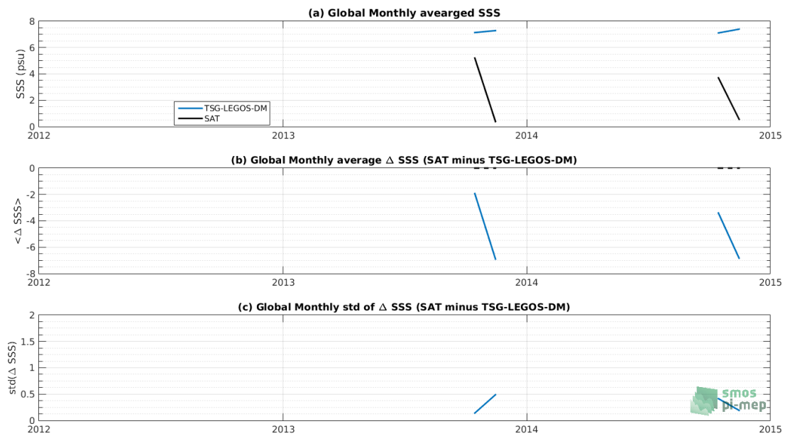
Figure 7: Time series of the monthly averaged mean SSS (top), mean \Delta SSS (Satellite - TSG-LEGOS-DM) and Std of \Delta SSS (Satellite - TSG-LEGOS-DM) over the Baltic Sea Pi-MEP region considering all match-ups collected by the Pi-MEP platform.
