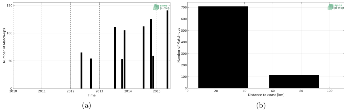
Figure 1: Number of match-ups between TSG-LEGOS-DM and Aquarius-L3-OR-V5-7DAY-RUNNING-RAIN-MASK-1DEG SSS as a function of time (a) and as function of the distance to coast (b) over the Baltic Sea Pi-MEP region and for the full satellite product period.
