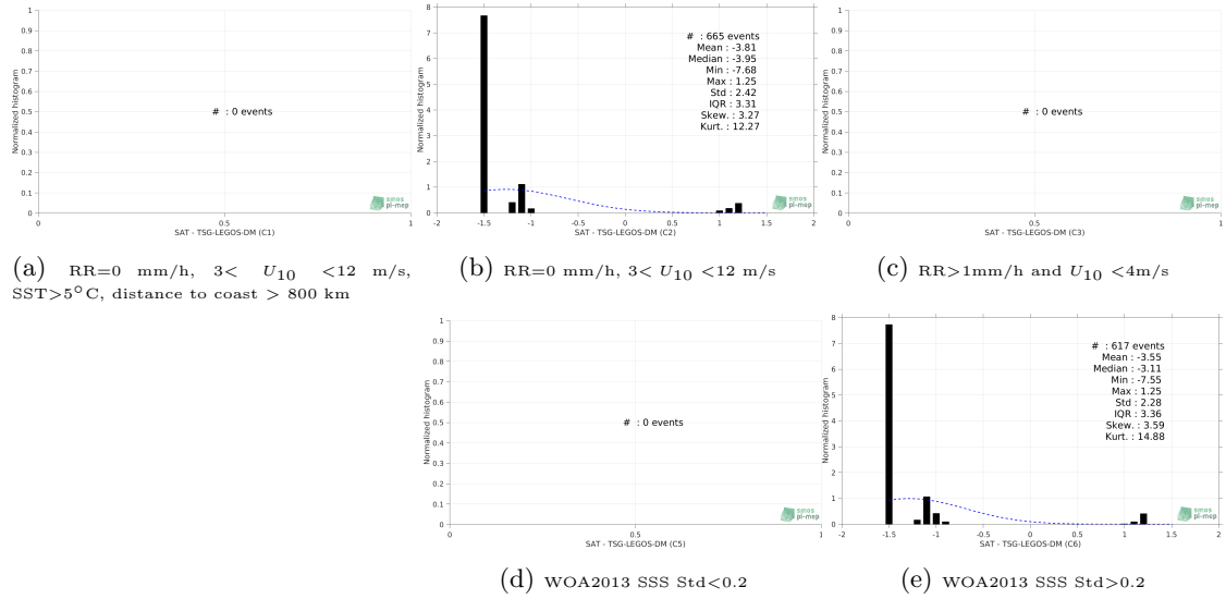
Figure 13: Normalized histogram of \Delta SSS (Aquarius-L3-OR-V5-7DAY-RUNNING-RAIN-MASK-1DEG - TSG-LEGOS-DM) for 5 different subdatasets corresponding to: RR=0 mm/h, 3 < U_{10} < 12 m/s, SST>5°C, distance to coast > 800 km (a), RR=0 mm/h, 3 < U_{10} < 12 m/s (b), RR>1mm/h and U_{10} < 4 m/s (c), WOA2013 SSS Std<0.2 (d), WOA2013 SSS Std>0.2 (e).
