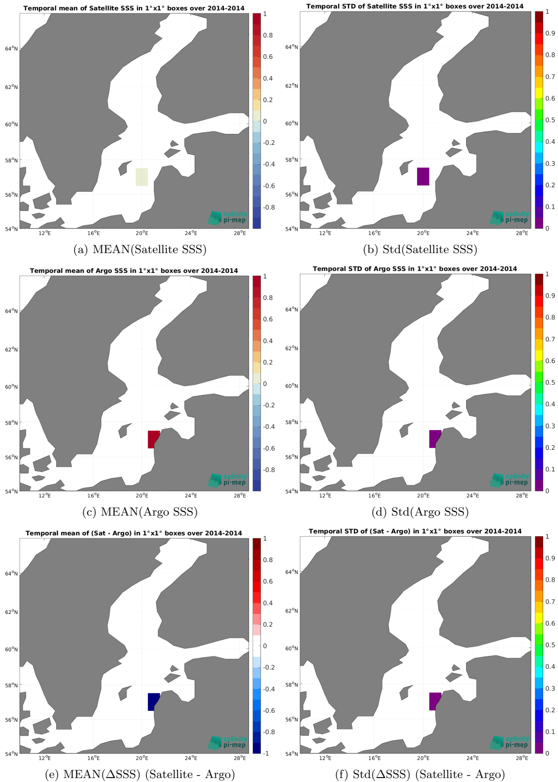
Figure 5: Temporal mean (left) and Std (right) of SSS from Aquarius SSS L3 OR v5 - 7-Day running - Rain mask (NASA-GSFC) (top), Argo 16 (middle), and of \Delta SSS (Satellite - Argo). Only match-up pairs are used to generate these maps.
