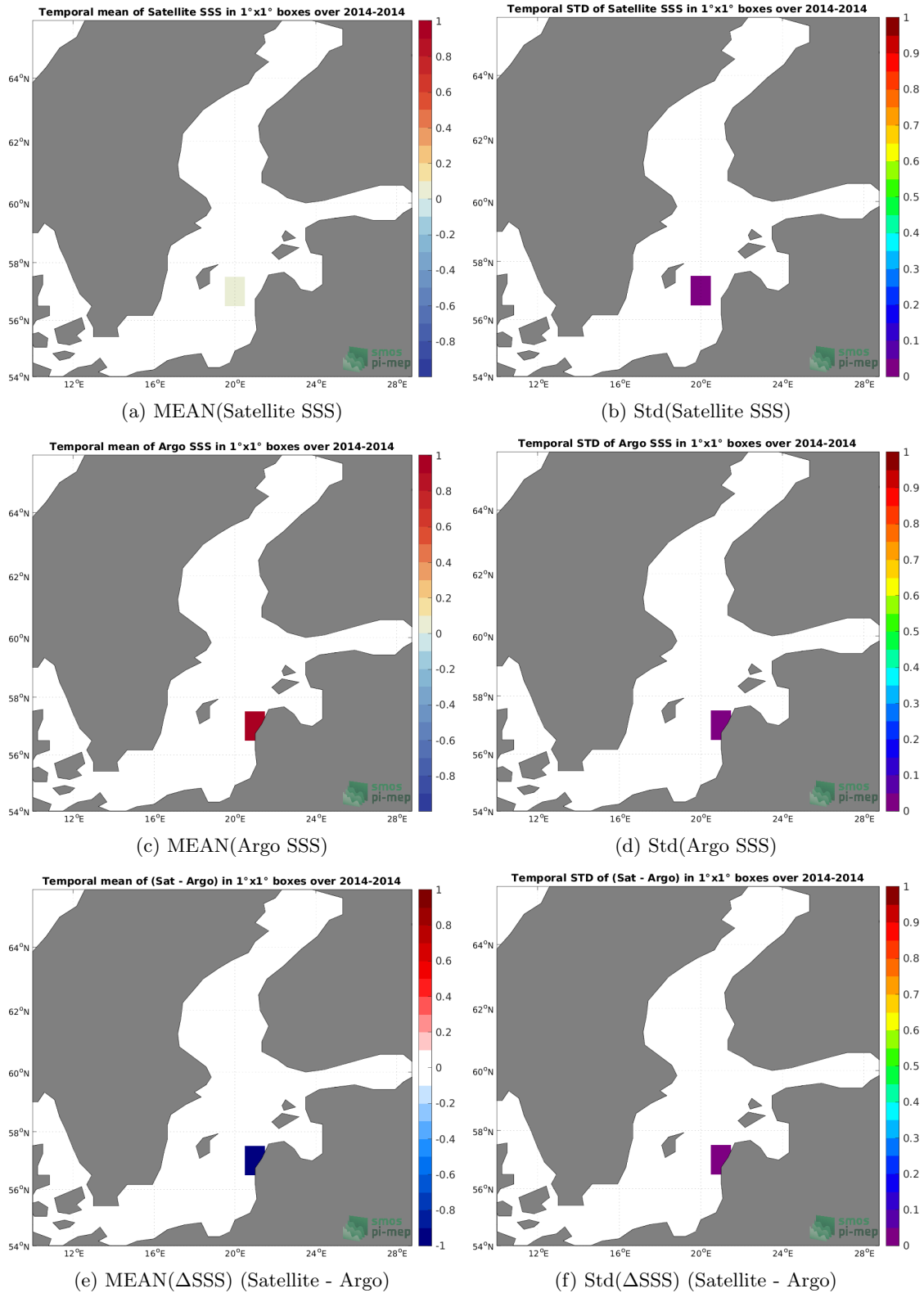
Figure 6: Temporal mean (left) and Std (right) of SSS from Aquarius SSS L3 OR v5 - 7-Day running - Rain mask (NASA-GSFC) (top), Argo 7 (middle), and of \Delta\text{SSS} (Satellite - Argo). Only match-up pairs are used to generate these maps.
