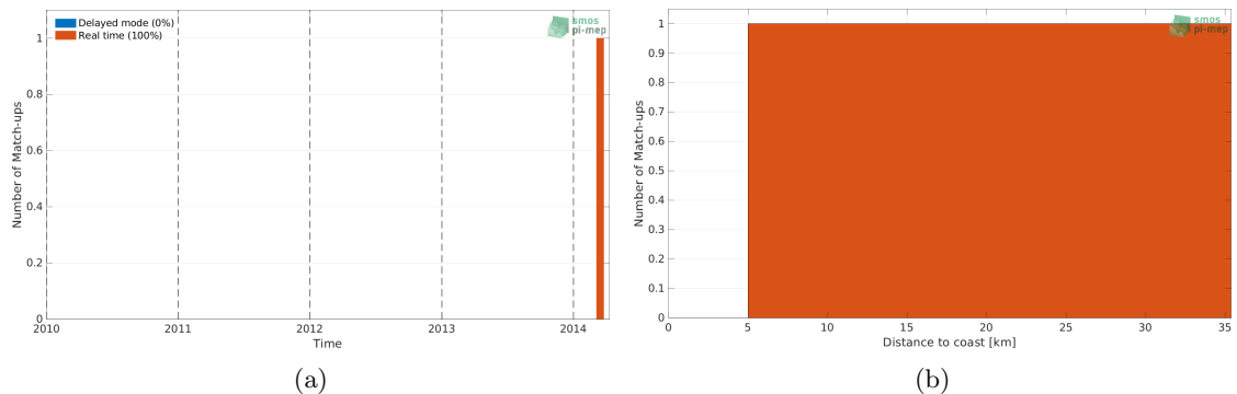
Figure 1: Number of match-ups between Argo and Aquarius SSS L3 OR v5 - 7-Day running - Rain mask (NASA-GSFC) SSS as a function of time (a) and as function of the distance to coast (b) over the Baltic Sea Pi-MEP region and for the full satellite product period.
