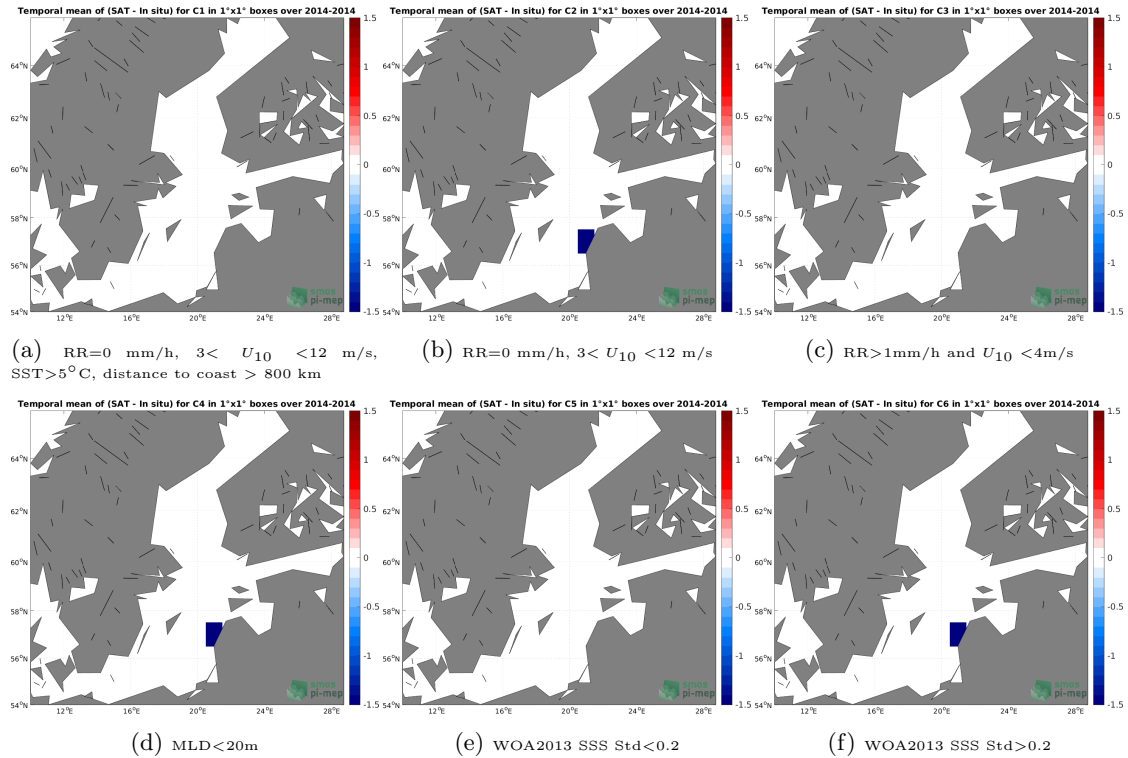
Figure 12: Temporal mean gridded over spatial boxes of size 1^{\circ}\times 1^{\circ} of \Delta\text{SSS} (Aquarius SSS L3 OR v5 - 7-Day running - Rain mask (NASA-GSFC) - Argo) for 6 different subdatasets corresponding to:RR=0 mm/h, 3 < U_{10} < 12 m/s, SST >5^{\circ}\text{C} , distance to coast > 800 km (a), RR=0 mm/h, 3 < U_{10} < 12 m/s (b), RR >1 mm/h and U_{10} < 4 m/s (c),MLD <20 m (d),WOA2013 SSS Std <0.2 (e),WOA2013 SSS Std >0.2 (f).
