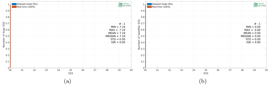
Figure 2: Histograms of SSS from Argo (a) and Aquarius SSS L3 OR v5 - 7-Day running - Rain mask (NASA-GSFC) (b) considering all match-up pairs per bins of 0.1 over the Baltic Sea Pi-MEP region and for the full satellite product period.
