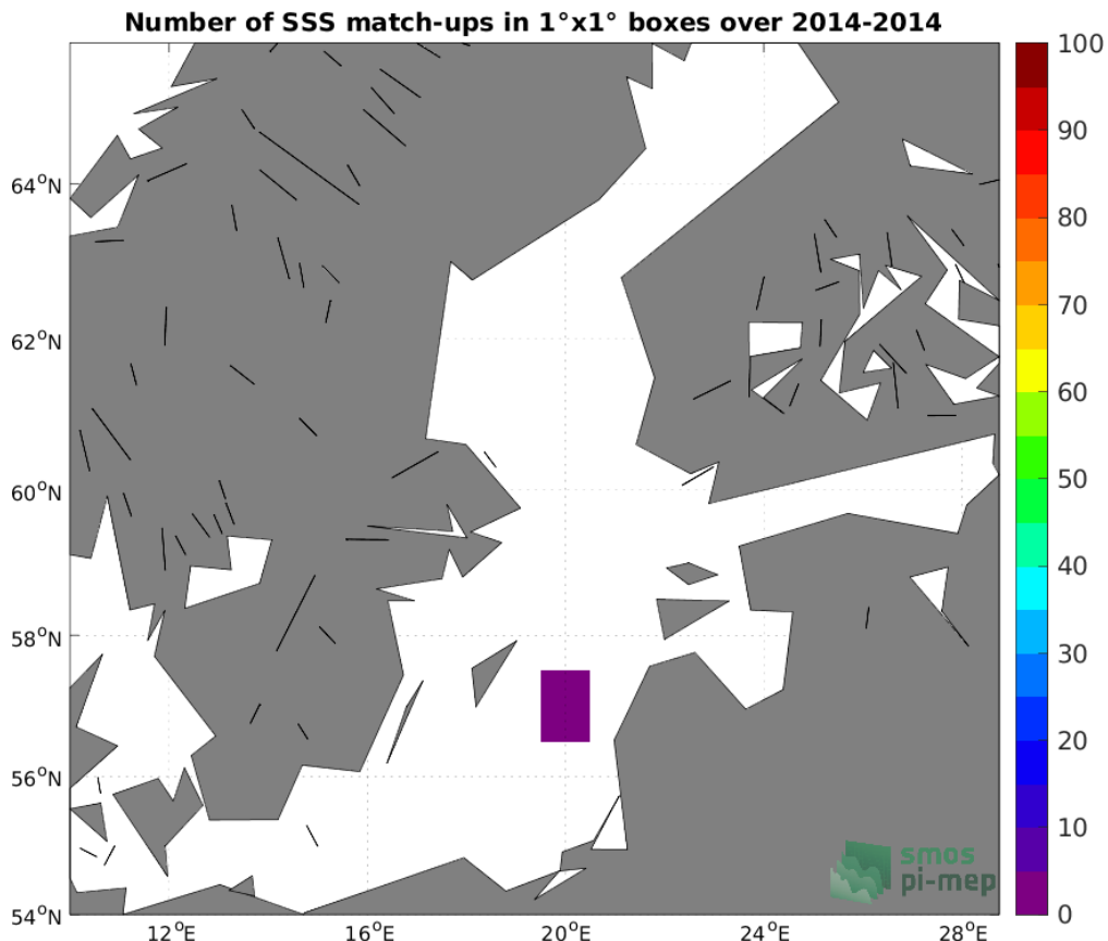
Figure 4: Number of SSS match-ups between Argo SSS and the Aquarius SSS L3 OR v5 - 7-Day running - Rain mask (NASA-GSFC) SSS product for the Baltic Sea Pi-MEP region over 1°×1° boxes and for the full satellite product period.
