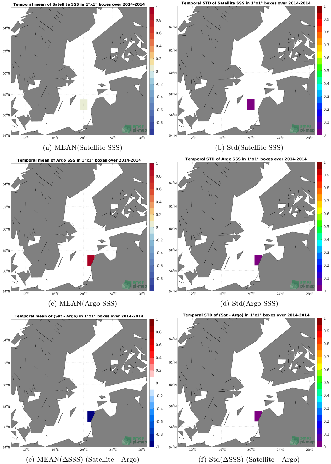
Figure 6: Temporal mean (left) and Std (right) of SSS from Aquarius SSS L3 OR v5 - 7-Day running - Rain mask (NASA-GSFC) (top), Argo 23 (middle), and of \Delta SSS (Satellite - Argo). Only match-up pairs are used to generate these maps.
