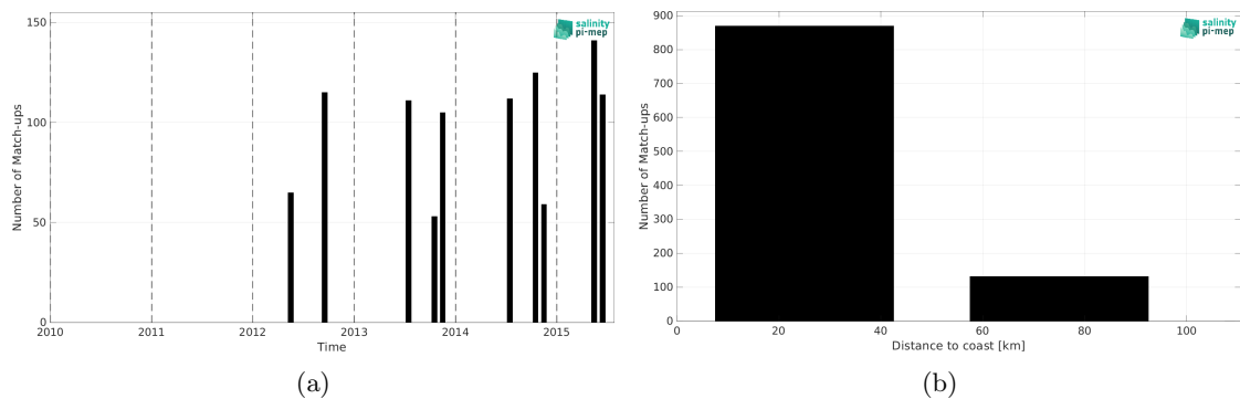
Figure 1: Number of match-ups between TSG (LEGOS-DM) and Aquarius SSS L3 OR v5 - Monthly (NASA-GSFC) SSS as a function of time (a) and as function of the distance to coast (b) over the Baltic Sea Pi-MEP region and for the full satellite product period.
