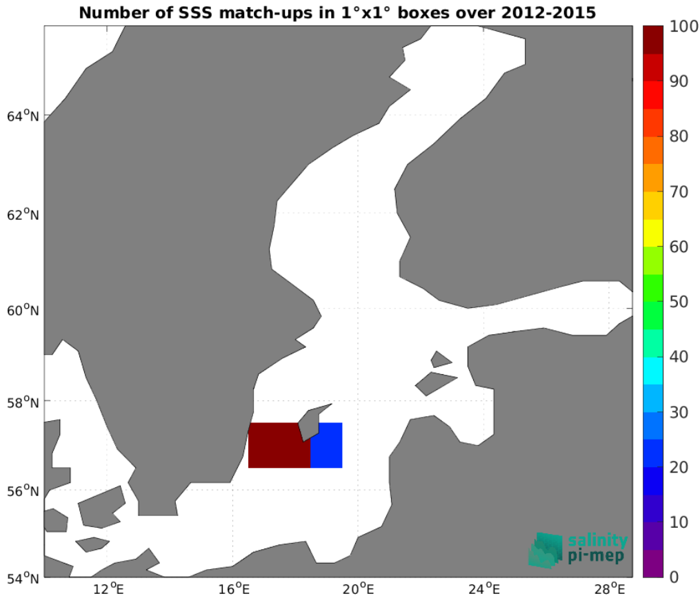
Figure 4: Number of SSS match-ups between TSG (LEGOS-DM) SSS and the Aquarius SSS L3 OR v5 - Monthly (NASA-GSFC) SSS product for the Baltic Sea Pi-MEP region over 1^\circ \times 1^\circ boxes and for the full satellite product period.
