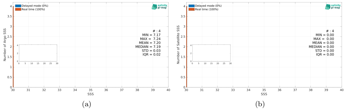
Figure 3: Histograms of SSS from Argo (a) and Aquarius SSS L3 OR v5 - Monthly (NASA-GSFC) (b) considering all match-up pairs per bins of 0.1 over the Baltic Sea Pi-MEP region and for the full satellite product period.
