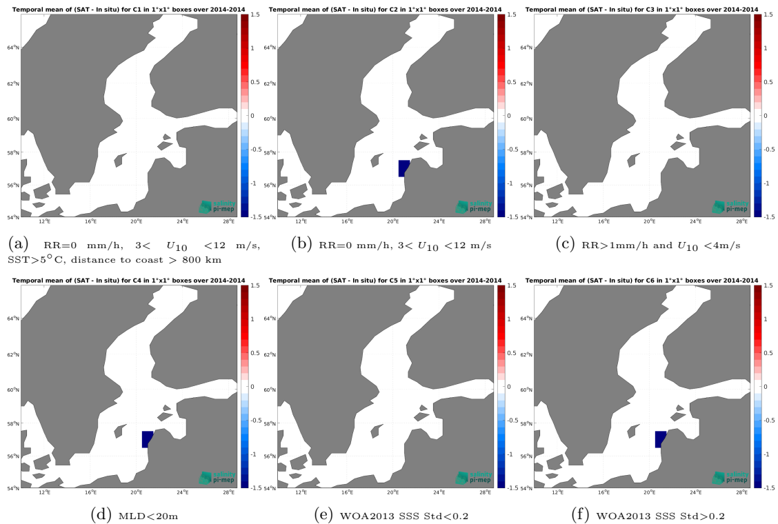
Figure 14: Temporal mean gridded over spatial boxes of size 1^\circ \times 1^\circ of \Delta SSS (Aquarius SSS L3 OR v5 - Monthly (NASA-GSFC) - Argo) for 6 different subdatasets corresponding to:RR=0 mm/h, 3 < U_{10} < 12 m/s, SST >5^\circ\text{C} , distance to coast > 800 km (a), RR=0 mm/h, 3 < U_{10} < 12 m/s (b), RR >1 mm/h and U_{10} < 4 m/s (c),MLD <20 m (d),WOA2013 SSS Std <0.2 (e),WOA2013 SSS Std >0.2 (f).
