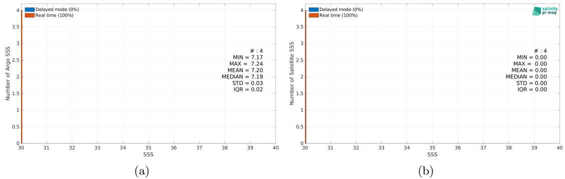
Figure 2: Histograms of SSS from Argo (a) and Aquarius SSS L3 OR v5 - Monthly (NASA-GSFC) (b) considering all match-up pairs per bins of 0.1 over the Baltic Sea Pi-MEP region and for the full satellite product period.
