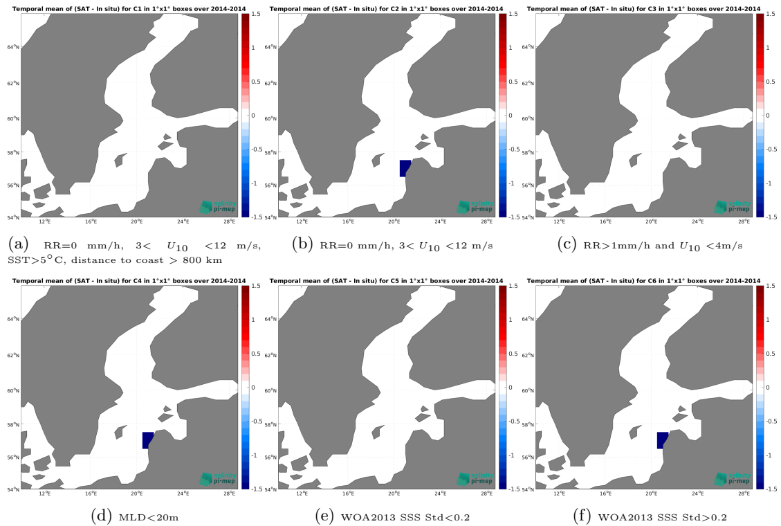
Figure 12: Temporal mean gridded over spatial boxes of size 1^{\circ}\times 1^{\circ} of \Delta\text{SSS} (Aquarius SSS L3 OR v5 - Monthly (NASA-GSFC) - Argo) for 6 different subdatasets corresponding to:RR=0 mm/h, 3 < U_{10} < 12 m/s, SST >5^{\circ}\text{C} , distance to coast > 800 km (a), RR=0 mm/h, 3 < U_{10} < 12 m/s (b), RR >1 mm/h and U_{10} < 4 m/s (c),MLD <20 m (d),WOA2013 SSS Std <0.2 (e),WOA2013 SSS Std >0.2 (f).
