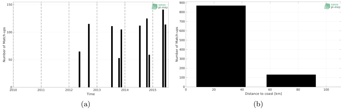
Figure 1: Number of match-ups between TSG (LEGOS-DM) and Aquarius SSS L3 OR v5 - Monthly - Rain mask (NASA-GSFC) SSS as a function of time (a) and as function of the distance to coast (b) over the Baltic Sea Pi-MEP region and for the full satellite product period.
