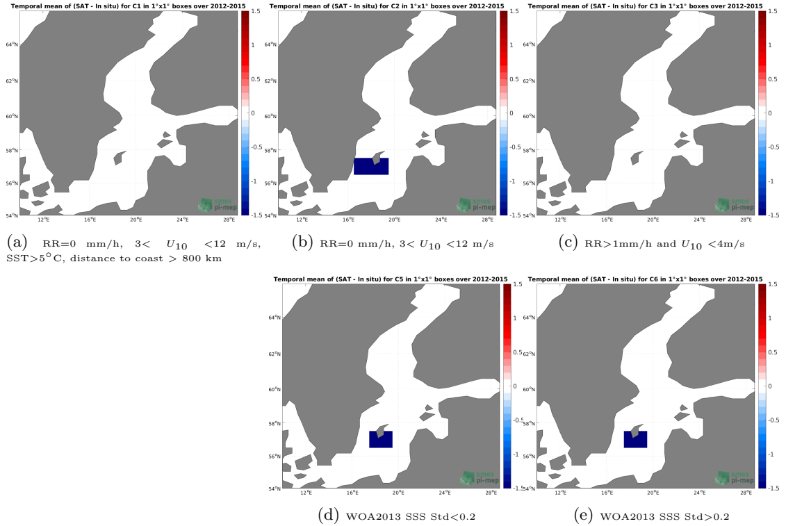
Figure 12: Temporal mean gridded over spatial boxes of size 1^{\circ}\times 1^{\circ} of \Delta\text{SSS} (Aquarius SSS L3 OR v5 - Monthly - Rain mask (NASA-GSFC) - TSG (LEGOS-DM)) for 5 different subdatasets corresponding to:RR=0 mm/h, 3 < U_{10} < 12 m/s, SST >5^{\circ}\text{C} , distance to coast > 800 km (a), RR=0 mm/h, 3 < U_{10} < 12 m/s (b), RR >1 mm/h and U_{10} < 4 m/s (c), WOA2013 SSS Std <0.2 (d), WOA2013 SSS Std >0.2 (e).
