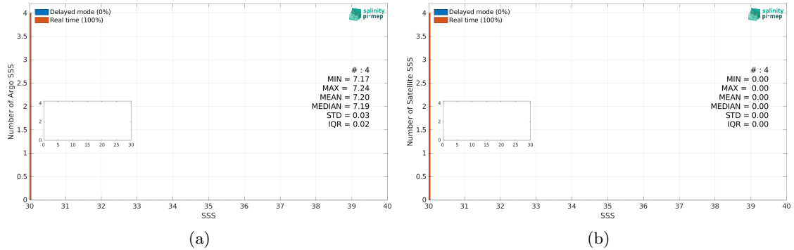
Figure 3: Histograms of SSS from Argo (a) and Aquarius SSS L3 OR v5 - Monthly - Rain mask (NASA-GSFC) (b) considering all match-up pairs per bins of 0.1 over the Baltic Sea Pi-MEP region and for the full satellite product period.
