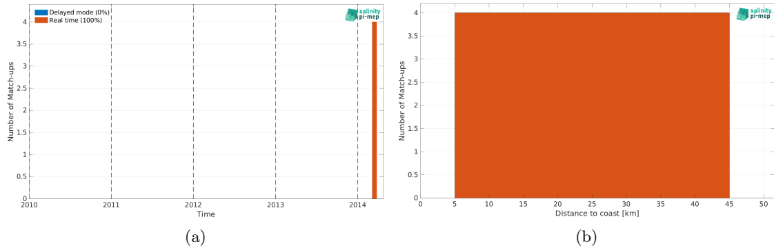
Figure 2: Number of match-ups between Argo and Aquarius SSS L3 OR v5 - Monthly - Rain mask (NASA-GSFC) SSS as a function of time (a) and as function of the distance to coast (b) over the Baltic Sea Pi-MEP region and for the full satellite product period.
