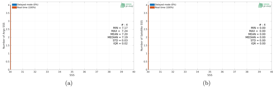
Figure 2: Histograms of SSS from Argo (a) and Aquarius SSS L3 OR v5 - Monthly - Rain mask (NASA-GSFC) (b) considering all match-up pairs per bins of 0.1 over the Baltic Sea Pi-MEP region and for the full satellite product period.
