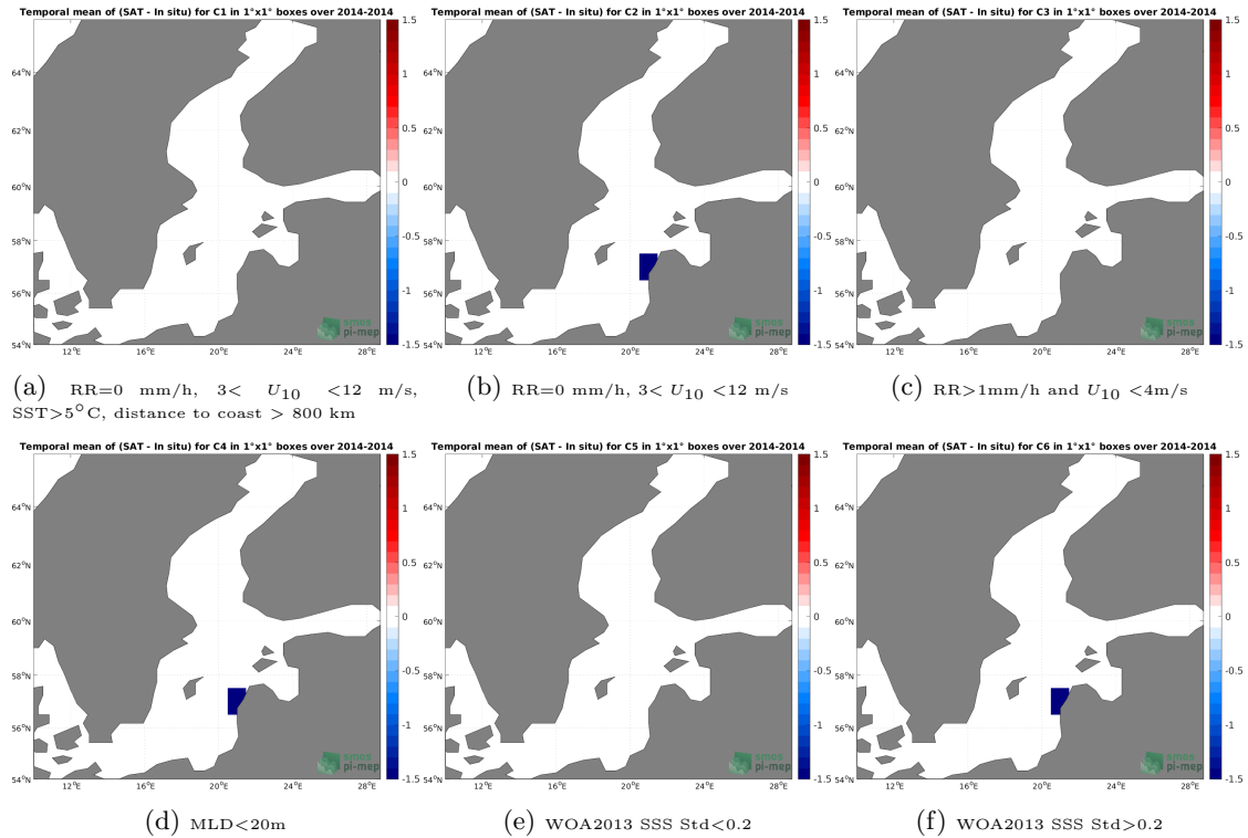
Figure 12: Temporal mean gridded over spatial boxes of size 1^{\circ}\times 1^{\circ} of \Delta\text{SSS} (Aquarius SSS L3 OR v5 - Monthly - Rain mask (NASA-GSFC) - Argo) for 6 different subdatasets corresponding to:RR=0 mm/h, 3 < U_{10} < 12 m/s, SST >5^{\circ}\text{C} , distance to coast > 800 km (a), RR=0 mm/h, 3 < U_{10} < 12 m/s (b), RR >1\text{mm/h} and U_{10} < 4\text{m/s} (c),MLD <20\text{m} (d),WOA2013 SSS Std <0.2 (e),WOA2013 SSS Std >0.2 (f).
