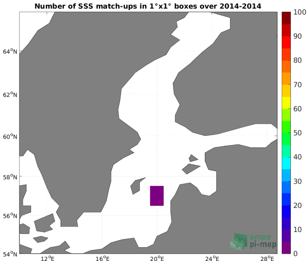
Figure 4: Number of SSS match-ups between Argo SSS and the Aquarius SSS L3 OR v5 - Monthly - Rain mask (NASA-GSFC) SSS product for the Baltic Sea Pi-MEP region over 1°×1° boxes and for the full satellite product period.
