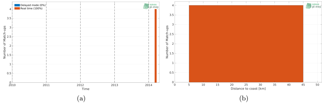
Figure 1: Number of match-ups between Argo and Aquarius SSS L3 OR v5 - Monthly - Rain mask (NASA-GSFC) SSS as a function of time (a) and as function of the distance to coast (b) over the Baltic Sea Pi-MEP region and for the full satellite product period.
