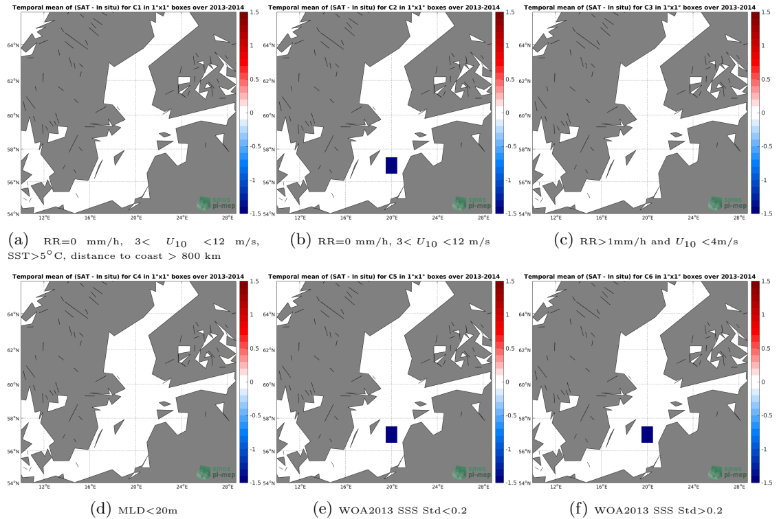
Figure 12: Temporal mean gridded over spatial boxes of size 1^{\circ}\times 1^{\circ} of \Delta\text{SSS} (Aquarius SSS L2-AVERAGED OR v5 (NASA-GSFC) - Argo) for 6 different subdatasets corresponding to:RR=0 mm/h, 3 < U_{10} < 12 m/s, SST >5^{\circ}\text{C} , distance to coast > 800 km (a), RR=0 mm/h, 3 < U_{10} < 12 m/s (b), RR >1\text{mm/h} and U_{10} < 4\text{m/s} (c),MLD <20\text{m} (d),WOA2013 SSS Std <0.2 (e),WOA2013 SSS Std >0.2 (f).
