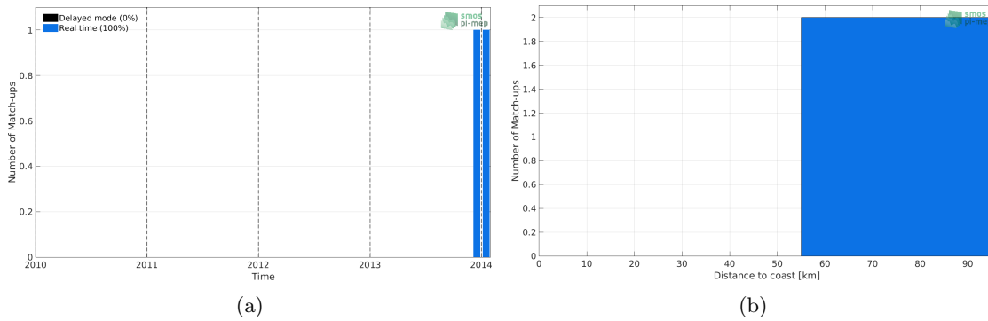
Figure 1: Number of match-ups between Argo and Aquarius SSS L2-AVERAGED OR v5 (NASA-GSFC) SSS as a function of time (a) and as function of the distance to coast (b) over the Baltic Sea Pi-MEP region and for the full satellite product period.
