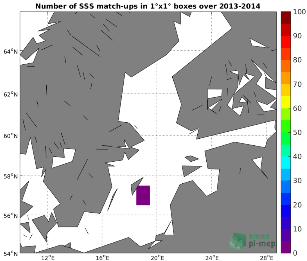
Figure 4: Number of SSS match-ups between Argo SSS and the Aquarius SSS L2-AVERAGED OR v5 (NASA-GSFC) SSS product for the Baltic Sea Pi-MEP region over 1°×1° boxes and for the full satellite product period.
