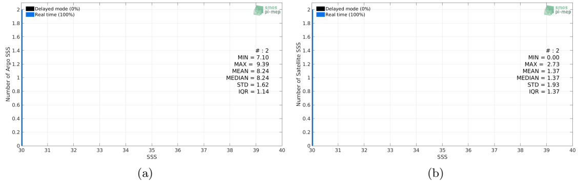
Figure 2: Histograms of SSS from Argo (a) and Aquarius SSS L2-AVERAGED OR v5 (NASA-GSFC) (b) considering all match-up pairs per bins of 0.1 over the Baltic Sea Pi-MEP region and for the full satellite product period.
