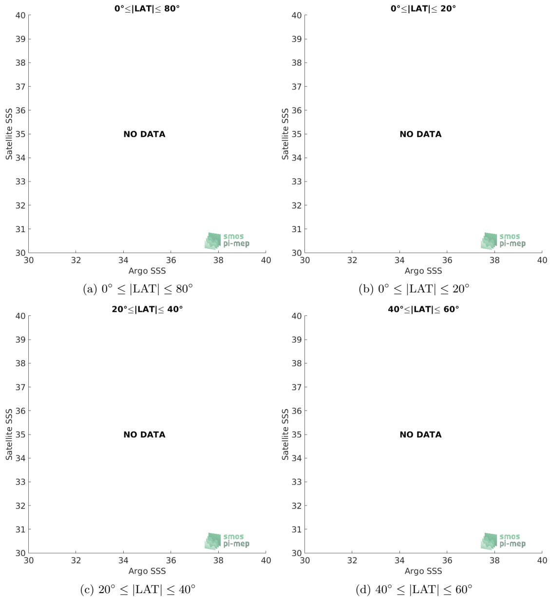
Figure 9: Contour maps of the concentration of Aquarius SSS L2-AVERAGED OR v5 (NASA-GSFC) SSS ( y -axis) versus Argo SSS ( x -axis) at match-up pairs for different latitude bands. For each plot, the red line shows x=y . The black thin and dashed lines indicate a linear fit through the data cloud and the \pm 95\% confidence levels, respectively. The number match-up pairs n , the slope and R^2 coefficient of the linear fit, the root mean square (RMS) and the mean bias between satellite and in situ data are indicated for each latitude band in each plot.
