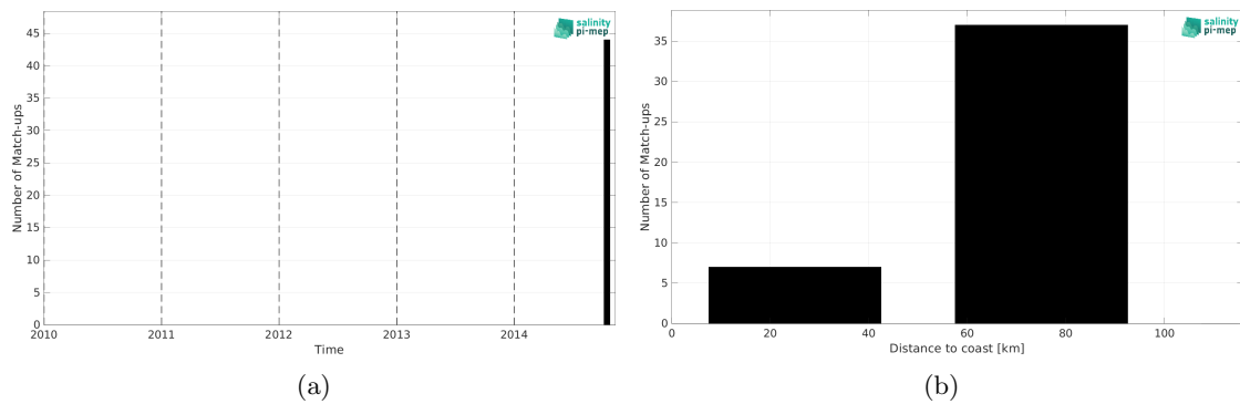
Figure 2: Number of match-ups between TSG (LEGOS-DM) and Aquarius SSS L2 OR v5 (NASA-GSFC) SSS as a function of time (a) and as function of the distance to coast (b) over the Baltic Sea Pi-MEP region and for the full satellite product period.
