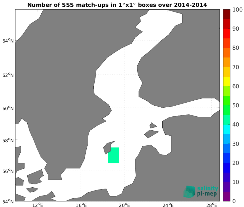
Figure 5: Number of SSS match-ups between TSG (LEGOS-DM) SSS and the Aquarius SSS L2 OR v5 (NASA-GSFC) SSS product for the Baltic Sea Pi-MEP region over 1°×1° boxes and for the full satellite product period.
