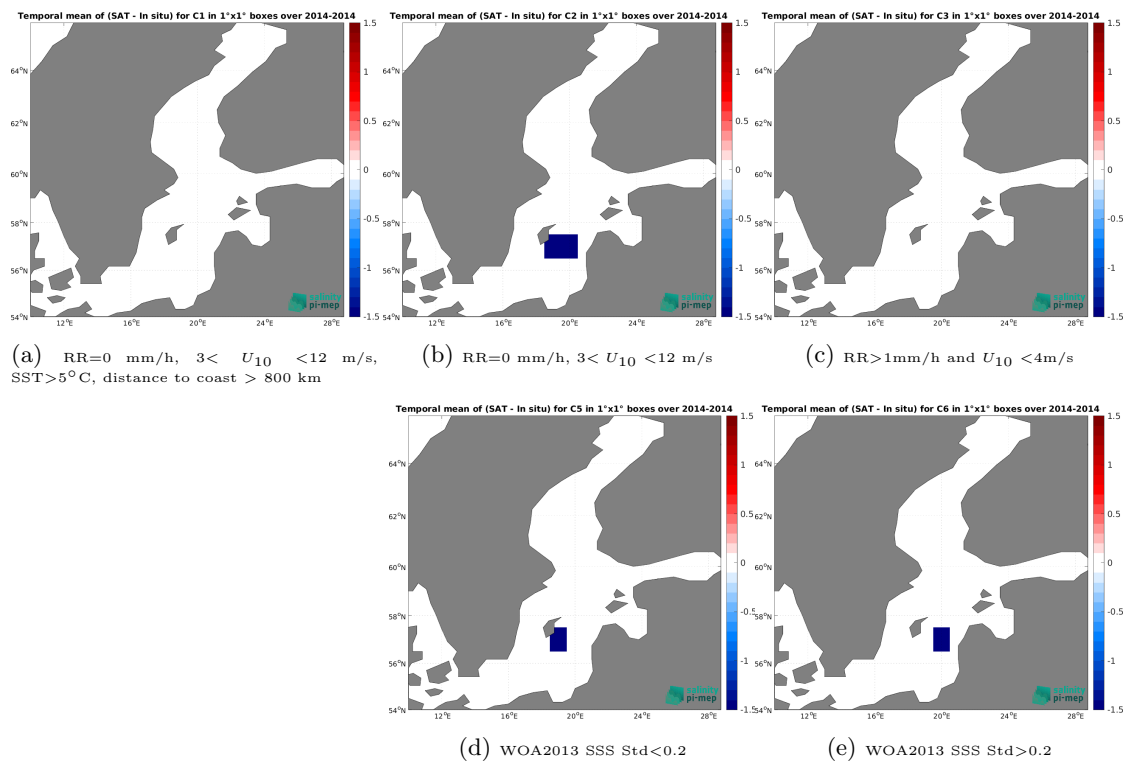
Figure 14: Temporal mean gridded over spatial boxes of size 1^\circ \times 1^\circ of \Delta SSS (Aquarius SSS L2 OR v5 (NASA-GSFC) - TSG (LEGOS-DM)) for 5 different subdatasets corresponding to:RR=0 mm/h, 3 < U_{10} < 12 m/s, SST>5°C, distance to coast > 800 km (a), RR=0 mm/h, 3 < U_{10} < 12 m/s (b), RR>1mm/h and U_{10} < 4 m/s (c), WOA2013 SSS Std<0.2 (d), WOA2013 SSS Std>0.2 (e).
