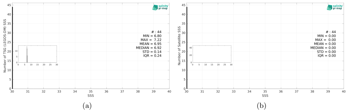
Figure 3: Histograms of SSS from TSG (LEGOS-DM) (a) and Aquarius SSS L2 OR v5 (NASA-GSFC) (b) considering all match-up pairs per bins of 0.1 over the Baltic Sea Pi-MEP region and for the full satellite product period.
