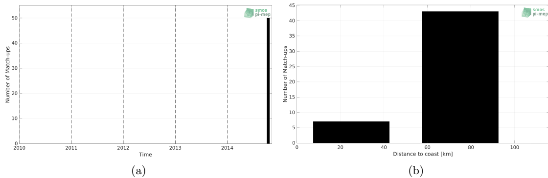
Figure 1: Number of match-ups between TSG (LEGOS-DM) and Aquarius SSS L2 OR v5 (NASA-GSFC) SSS as a function of time (a) and as function of the distance to coast (b) over the Baltic Sea Pi-MEP region and for the full satellite product period.
