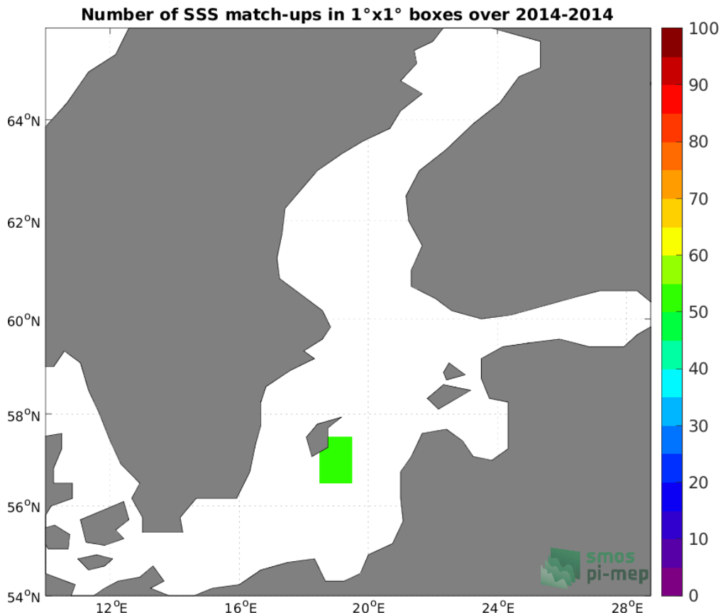
Figure 4: Number of SSS match-ups between TSG (LEGOS-DM) SSS and the Aquarius SSS L2 OR v5 (NASA-GSFC) SSS product for the Baltic Sea Pi-MEP region over 1°×1° boxes and for the full satellite product period.
