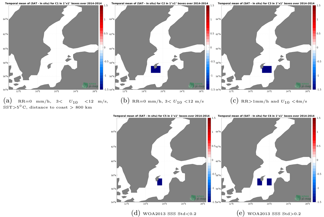
Figure 12: Temporal mean gridded over spatial boxes of size 1^{\circ}\times 1^{\circ} of \Delta\text{SSS} (Aquarius SSS L2 OR v5 (NASA-GSFC) - TSG (LEGOS-DM)) for 5 different subdatasets corresponding to:RR=0 mm/h, 3 < U_{10} < 12 m/s, SST > 5^{\circ}\text{C} , distance to coast > 800 km (a), RR=0 mm/h, 3 < U_{10} < 12 m/s (b), RR > 1 mm/h and U_{10} < 4 m/s (c), WOA2013 SSS Std < 0.2 (d), WOA2013 SSS Std > 0.2 (e).
