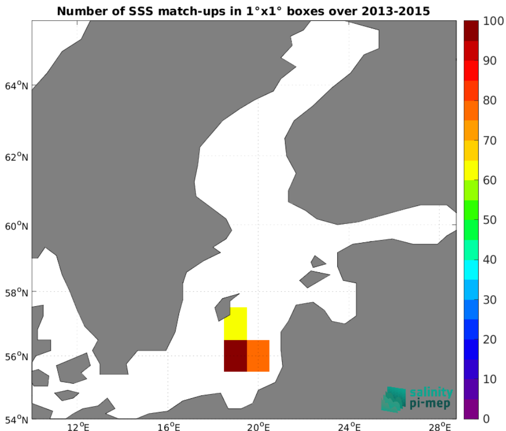
Figure 5: Number of SSS match-ups between ICES SSS and the Aquarius SSS L2 OR v5 (NASA-GSFC) SSS product for the Baltic Sea Pi-MEP region over 1°x1° boxes and for the full satellite product period.
