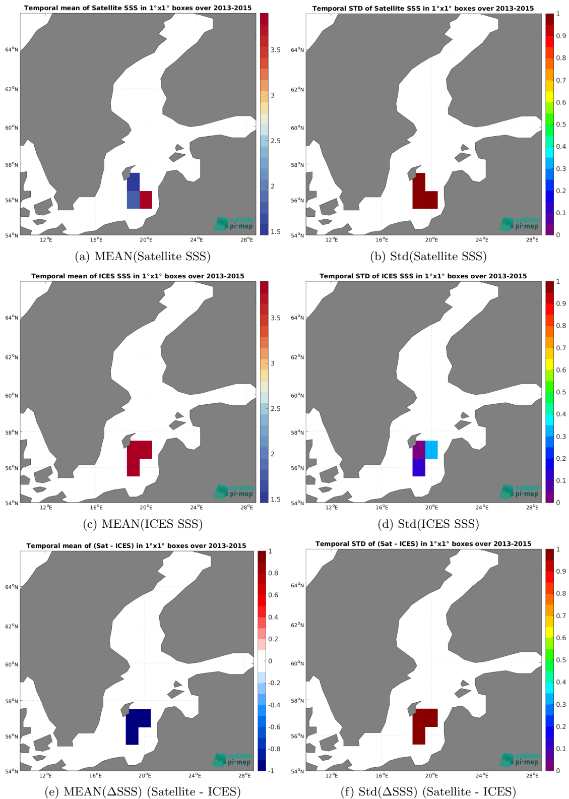
Figure 7: Temporal mean (left) and Std (right) of SSS from Aquarius SSS L2 OR v5 (NASA-GSFC) (top), ICES (middle), and of \Delta SSS (Satellite - ICES). Only match-up pairs are used to generate these maps.
