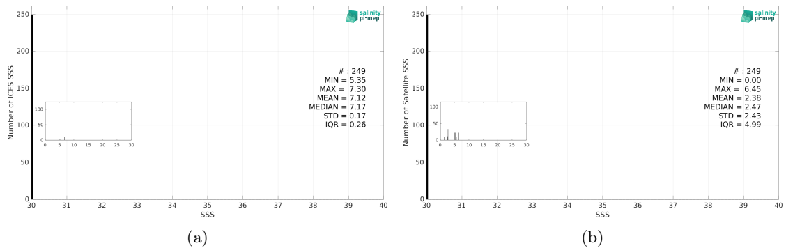
Figure 3: Histograms of SSS from ICES (a) and Aquarius SSS L2 OR v5 (NASA-GSFC) (b) considering all match-up pairs per bins of 0.1 over the Baltic Sea Pi-MEP region and for the full satellite product period.
