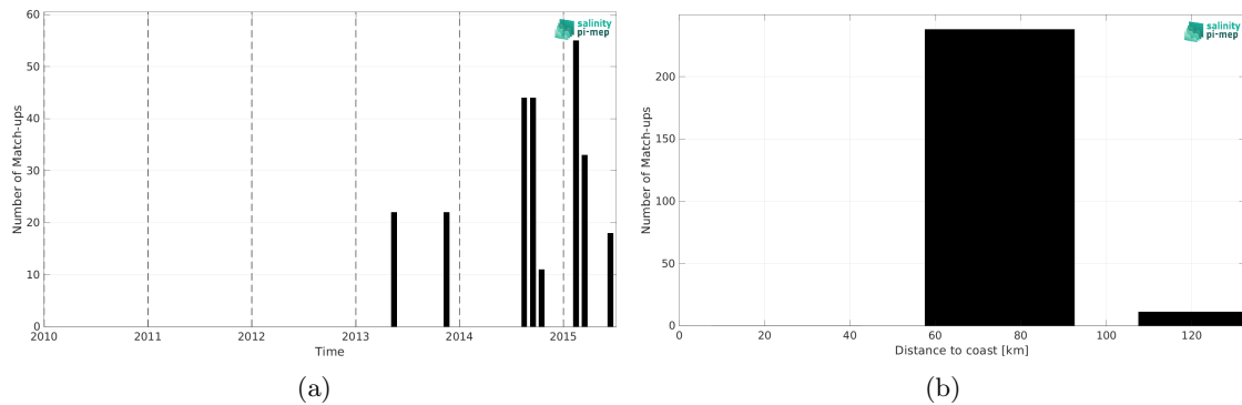
Figure 2: Number of match-ups between ICES and Aquarius SSS L2 OR v5 (NASA-GSFC) SSS as a function of time (a) and as function of the distance to coast (b) over the Baltic Sea Pi-MEP region and for the full satellite product period.
