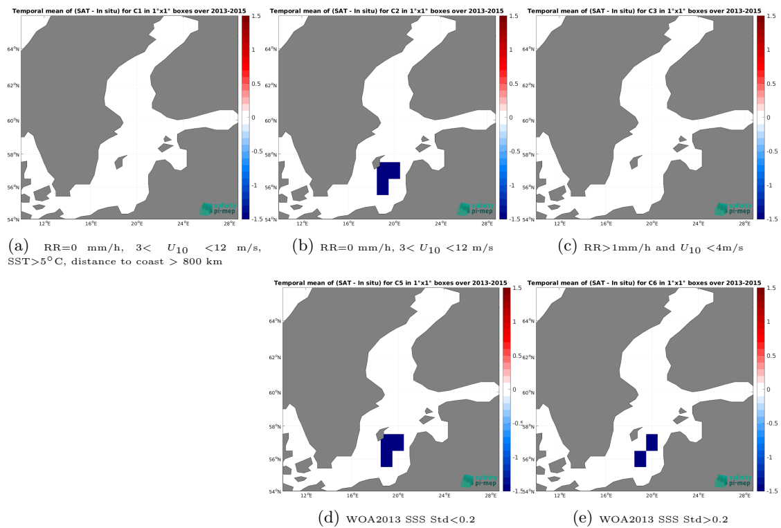
Figure 14: Temporal mean gridded over spatial boxes of size 1^\circ \times 1^\circ of \Delta SSS (Aquarius SSS L2 OR v5 (NASA-GSFC) - ICES) for 5 different subdatasets corresponding to:RR=0 mm/h, 3 < U_{10} < 12 m/s, SST >5^\circ\text{C} , distance to coast > 800 km (a), RR=0 mm/h, 3 < U_{10} < 12 m/s (b), RR >1 mm/h and U_{10} < 4 m/s (c), WOA2013 SSS Std <0.2 (d), WOA2013 SSS Std >0.2 (e).
