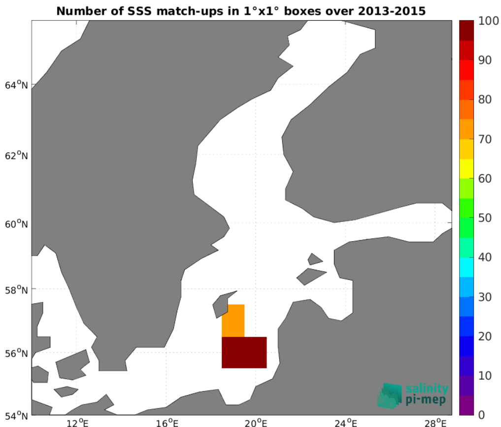
Figure 4: Number of SSS match-ups between ICES SSS and the Aquarius SSS L2 OR v5 (NASA-GSFC) SSS product for the Baltic Sea Pi-MEP region over 1^\circ \times 1^\circ boxes and for the full satellite product period.
