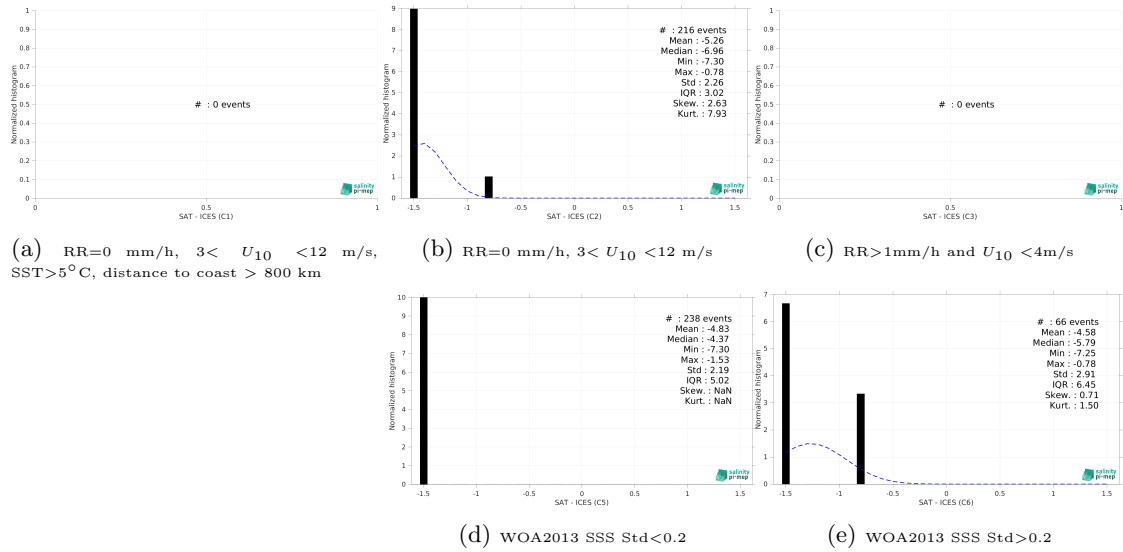
Figure 13: Normalized histogram of \Delta\text{SSS} (Aquarius SSS L2 OR v5 (NASA-GSFC) - ICES) for 5 different subdatasets corresponding to: RR=0 mm/h, 3 < U_{10} < 12 m/s, SST > 5^\circ\text{C} , distance to coast > 800 km (a), RR=0 mm/h, 3 < U_{10} < 12 m/s (b), RR > 1\text{mm/h} and U_{10} < 4\text{m/s} (c), WOA2013 SSS Std < 0.2 (d), WOA2013 SSS Std > 0.2 (e).
