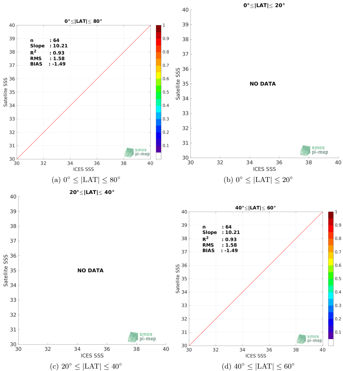
Figure 9: Contour maps of the concentration of Aquarius SSS L2 OR v5 (NASA-GSFC) SSS (y-axis) versus ICES SSS (x-axis) at match-up pairs for different latitude bands. For each plot, the red line shows x=y . The black thin and dashed lines indicate a linear fit through the data cloud and the \pm 95\% confidence levels, respectively. The number match-up pairs n , the slope and R^2 coefficient of the linear fit, the root mean square (RMS) and the mean bias between satellite and in situ data are indicated for each latitude band in each plots.
