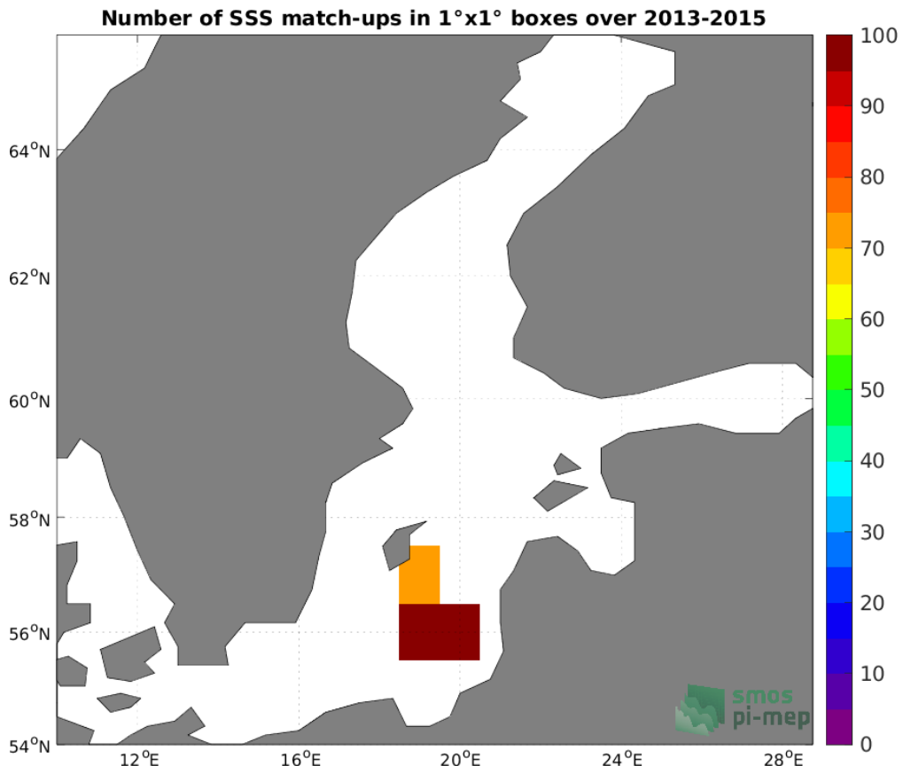
Figure 4: Number of SSS match-ups between ICES SSS and the Aquarius SSS L2 OR v5 (NASA-GSFC) SSS product for the Baltic Sea Pi-MEP region over 1°x1° boxes and for the full satellite product period.
