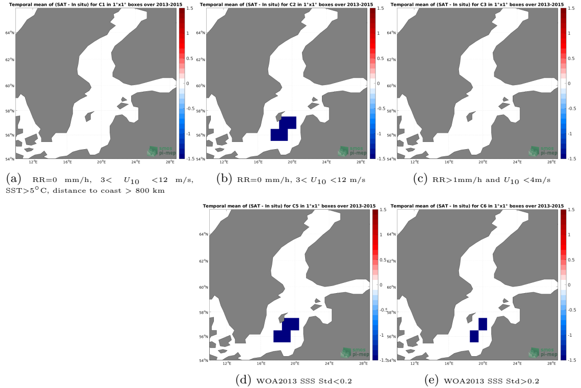
Figure 12: Temporal mean gridded over spatial boxes of size 1^{\circ}\times 1^{\circ} of \Delta\text{SSS} (Aquarius SSS L2 OR v5 (NASA-GSFC) - ICES) for 5 different subdatasets corresponding to: \text{RR}=0 mm/h, 3 < U_{10} < 12 m/s, \text{SST} > 5^{\circ}\text{C} , distance to coast > 800 km (a), \text{RR}=0 mm/h, 3 < U_{10} < 12 m/s (b), \text{RR} > 1\text{mm/h} and U_{10} < 4\text{m/s} (c), WOA2013 SSS Std < 0.2 (d), WOA2013 SSS Std > 0.2 (e).
