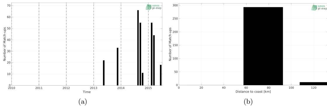
Figure 1: Number of match-ups between ICES and Aquarius SSS L2 OR v5 (NASA-GSFC) SSS as a function of time (a) and as function of the distance to coast (b) over the Baltic Sea Pi-MEP region and for the full satellite product period.
