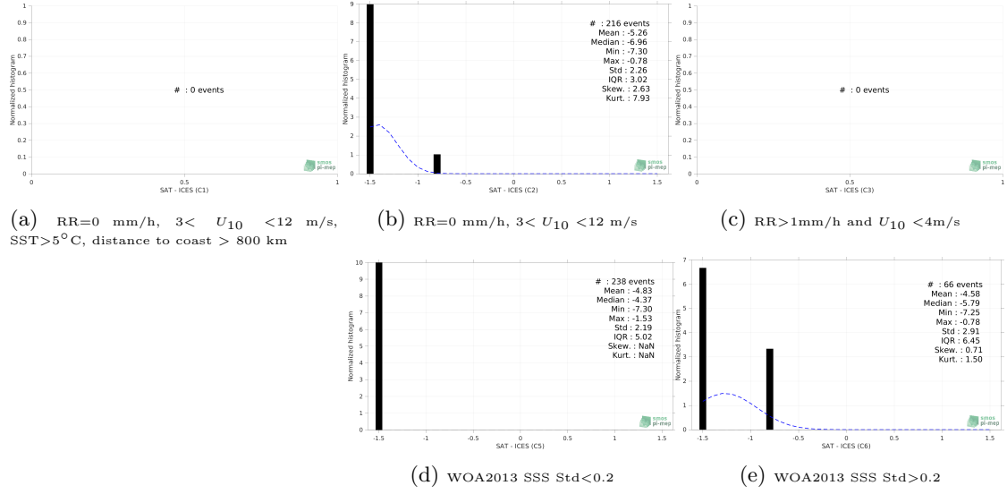
Figure 13: Normalized histogram of \Delta SSS (Aquarius SSS L2 OR v5 (NASA-GSFC) - ICES) for 5 different subdatasets corresponding to: RR=0 mm/h, 3 < U_{10} < 12 m/s, SST>5°C, distance to coast > 800 km (a), RR=0 mm/h, 3 < U_{10} < 12 m/s (b), RR>1mm/h and U_{10} < 4 m/s (c), WOA2013 SSS Std<0.2 (d), WOA2013 SSS Std>0.2 (e).
