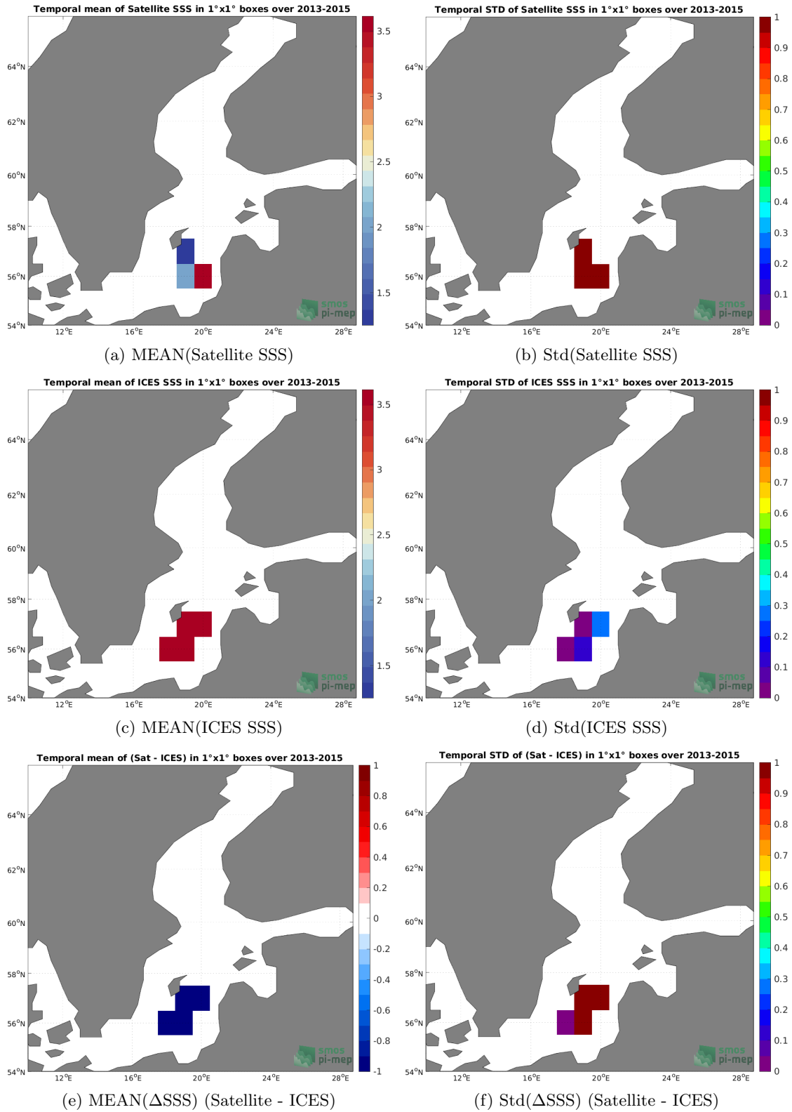
Figure 6: Temporal mean (left) and Std (right) of SSS from Aquarius SSS L2 OR v5 (NASA-GSFC) (top), ICES (middle), and of \Delta SSS (Satellite - ICES). Only match-up pairs are used to generate these maps.
