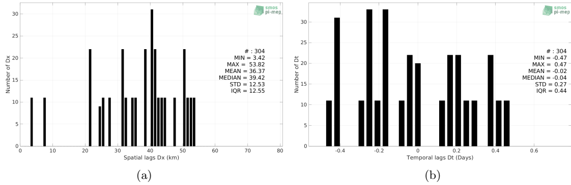
Figure 5: Histograms of the spatial (a) and temporal (b) lags between the location/time of the ICES measurement and the date of the corresponding Aquarius SSS L2 OR v5 (NASA-GSFC) SSS pixel.
