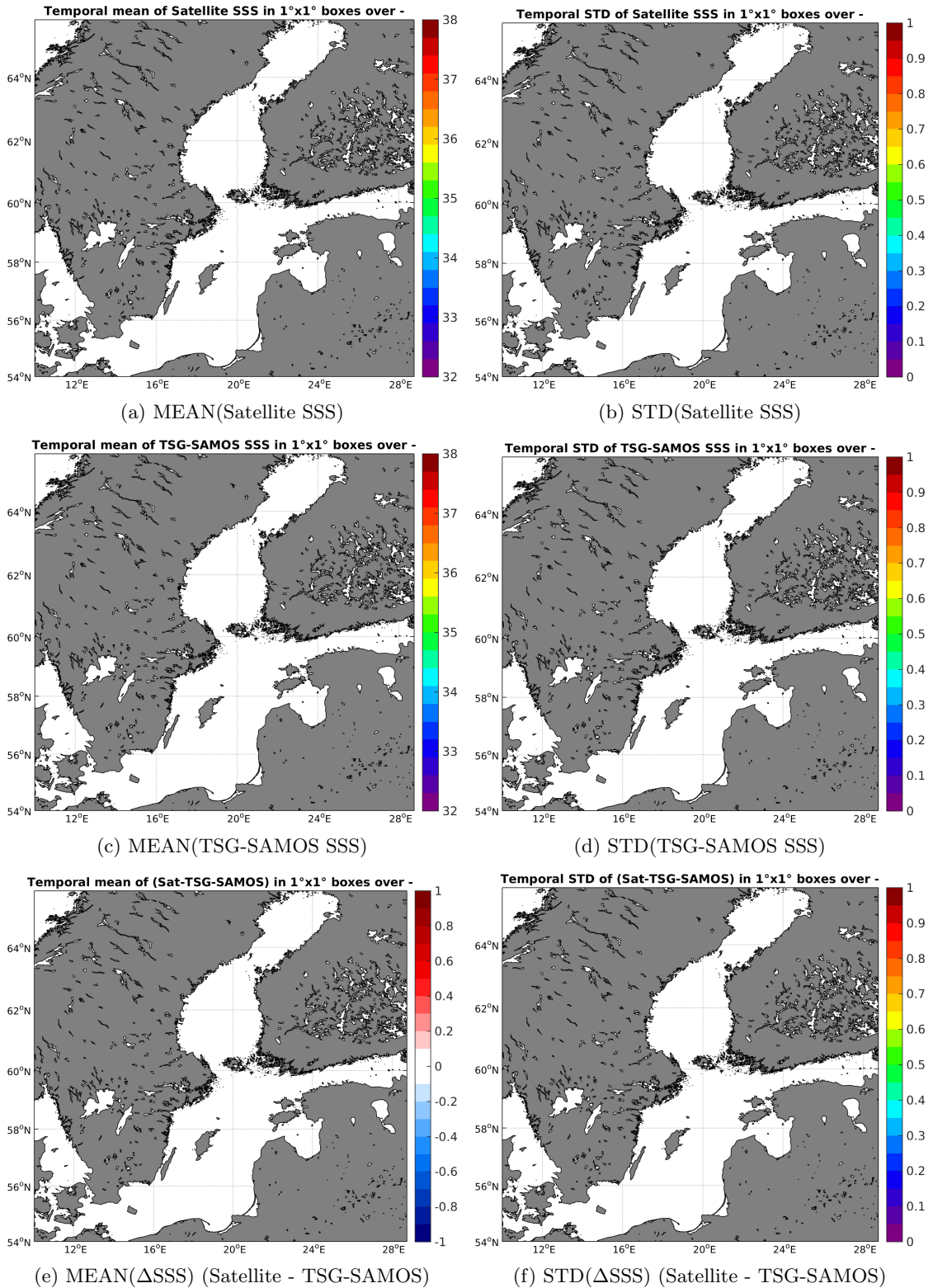
Figure 6: Temporal mean (left) and STD (right) of SSS from AQUARIUS-L2-JPL-V4 (top), TSG-SAMOS (middle), and of \Delta SSS (Satellite - TSG-SAMOS). Only match-up pairs are used to generate these maps.
