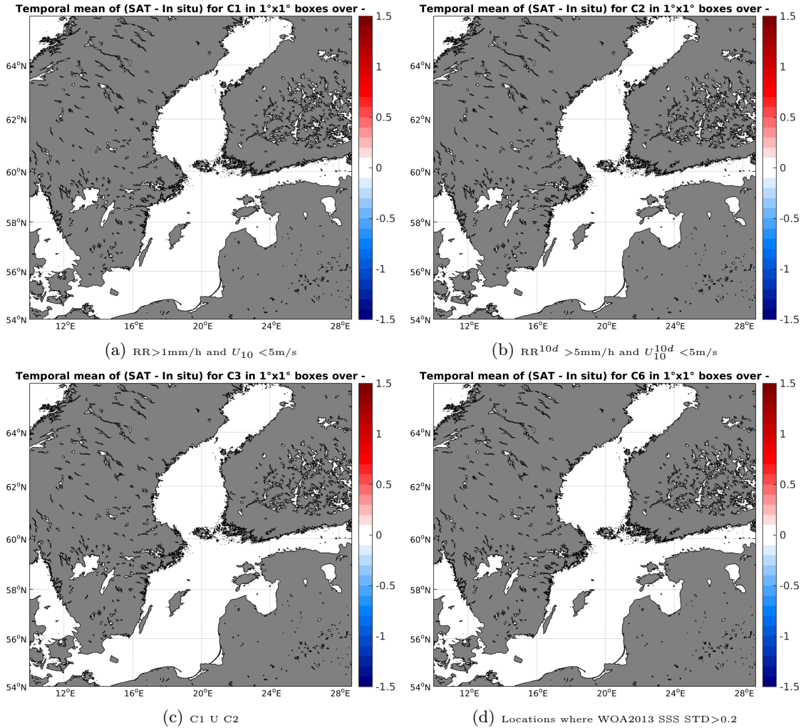
Figure 12: Temporal mean gridded over spatial boxes of size 1^\circ \times 1^\circ of \Delta SSS (AQUARIUS-L2-JPL-V4 - TSG-SAMOS) for 4 different subdatasets corresponding to: RR > 1\text{mm/h} and U_{10} < 5\text{m/s} (a), RR^{10d} > 5\text{mm/h} and U_{10}^{10d} < 5\text{m/s} (b), C1 U C2 (c), Locations where WOA2013 SSS STD > 0.2 (d).
