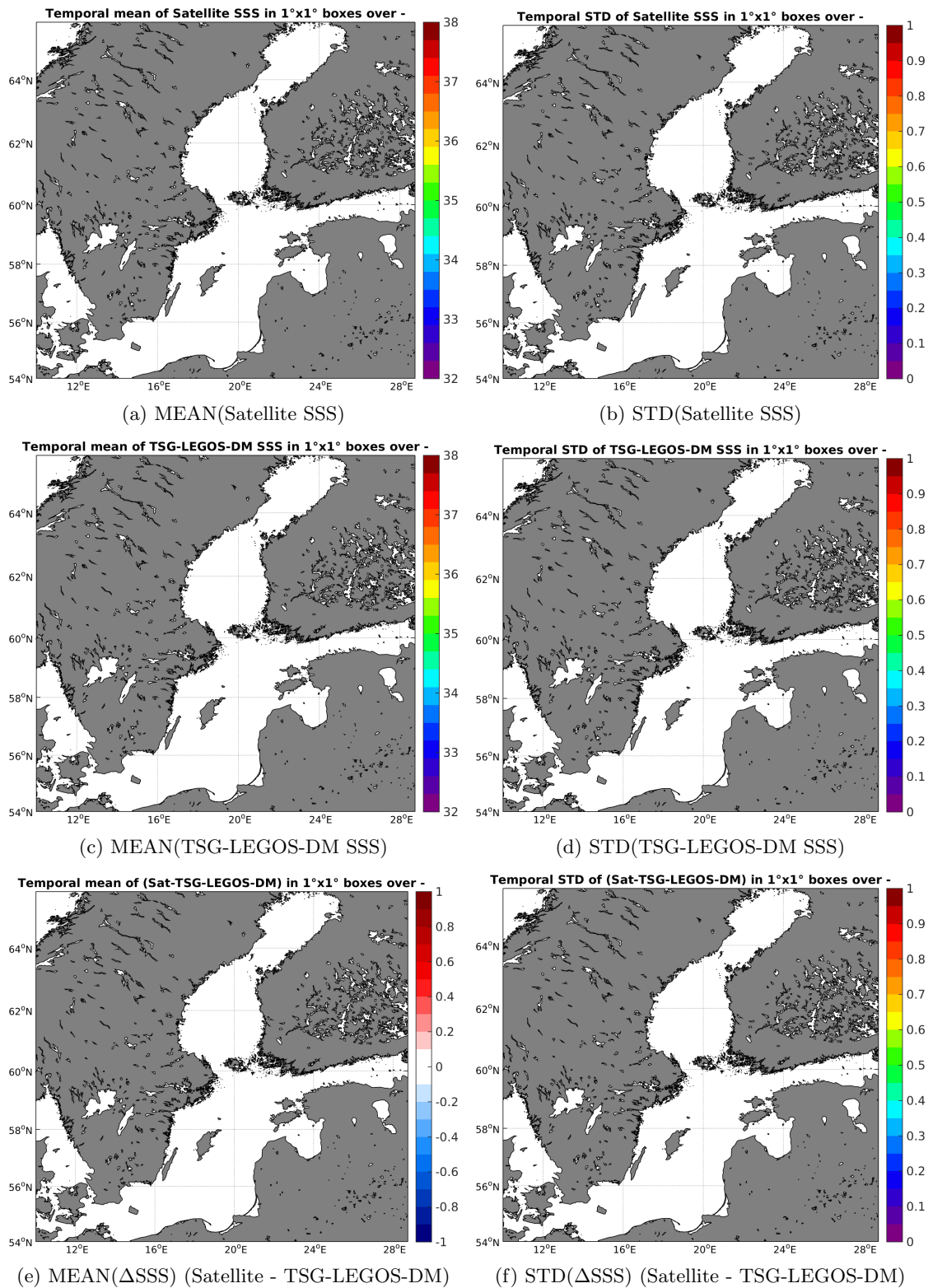
Figure 6: Temporal mean (left) and STD (right) of SSS from AQUARIUS-L2-JPL-V4 (top), TSG-LEGOS-DM (middle), and of \Delta SSS (Satellite - TSG-LEGOS-DM). Only match-up pairs are used to generate these maps.
