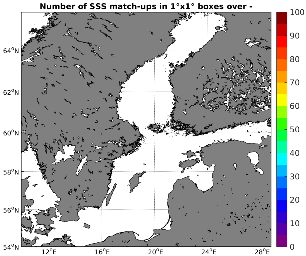
Figure 4: Number of SSS match-ups between TSG-LEGOS-DM SSS and the AQUARIUS-L2-JPL-V4 SSS product for the Baltic Sea Pi-MEP region over 1°x1° boxes and for the full satellite product period.
