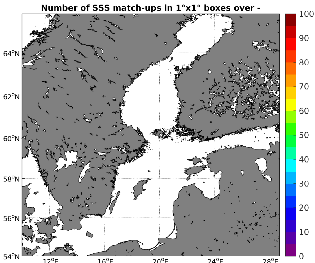
Figure 4: Number of SSS match-ups between TSG-GOSUD-Research-vessel SSS and the AQUARIUS-L2-JPL-V4 SSS product for the Baltic Sea Pi-MEP region over 1°x1° boxes and for the full satellite product period.
