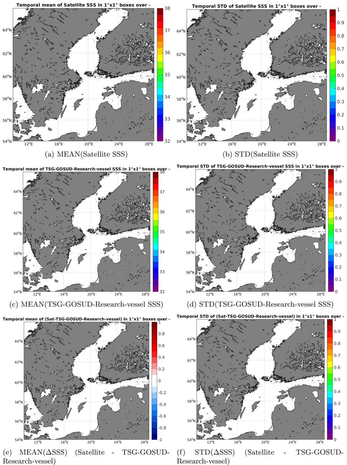
Figure 6: Temporal mean (left) and STD (right) of SSS from AQUARIUS-L2-JPL-V4 (top), TSG-GOSUD-Research-vessel (middle), and of \Delta SSS (Satellite - TSG-GOSUD-Research-vessel). Only match-up pairs are used to generate these maps.
