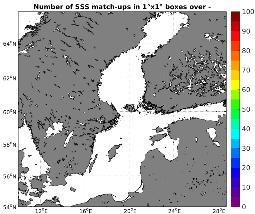
Figure 4: Number of SSS match-ups between Sea mammals SSS and the AQUARIUS-L2-JPL-V4 SSS product for the Baltic Sea Pi-MEP region over 1°x1° boxes and for the full satellite product period.
