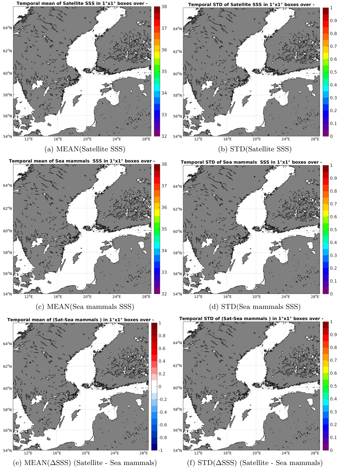
Figure 6: Temporal mean (left) and STD (right) of SSS from AQUARIUS-L2-JPL-V4 (top), Sea mammals (middle), and of \Delta SSS (Satellite - Sea mammals). Only match-up pairs are used to generate these maps.
