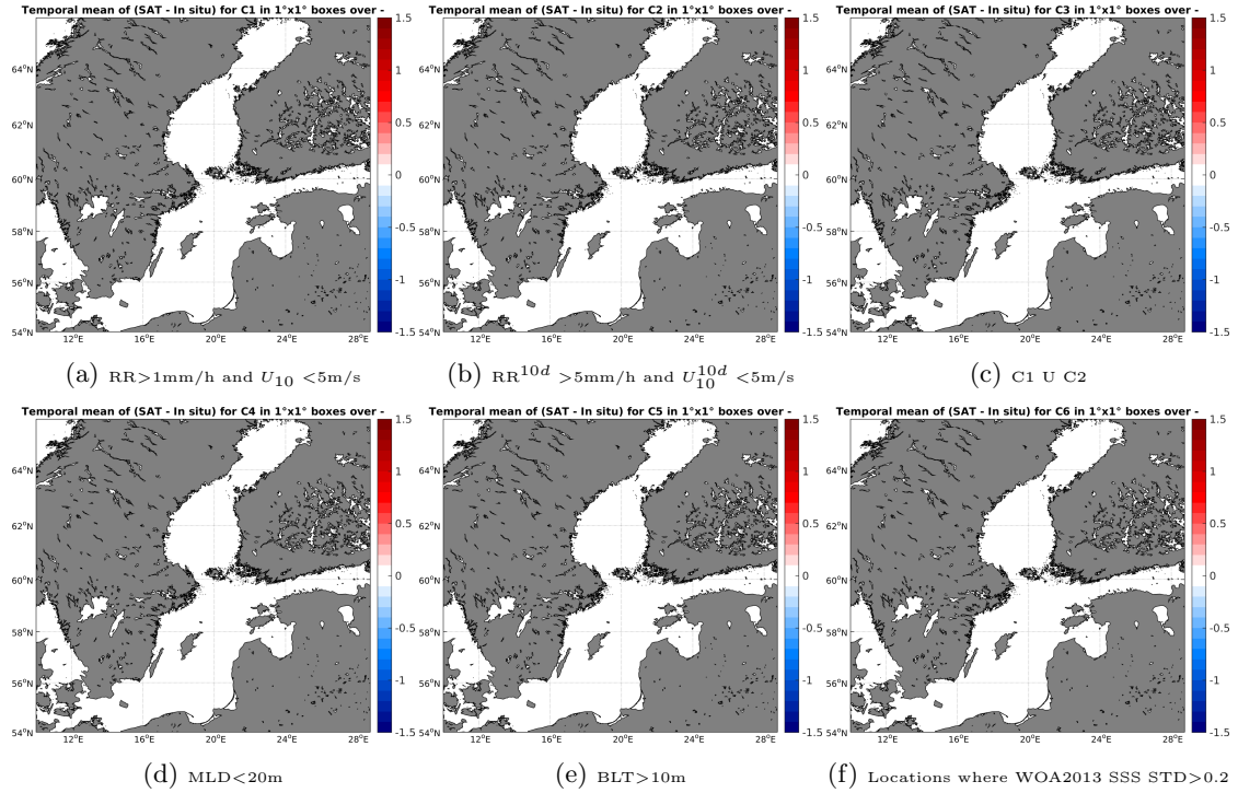
Figure 12: Temporal mean gridded over spatial boxes of size 1^\circ \times 1^\circ of \Delta SSS (AQUARIUS-L2-JPL-V4 - Sea mammals) for 6 different subdatasets corresponding to: RR > 1mm/h and U_{10} < 5 m/s (a), RR^{10d} > 5 mm/h and U_{10}^{10d} < 5 m/s (b), C1 U C2 (c), MLD < 20m (d), BLT > 10m (e), Locations where WOA2013 SSS STD > 0.2 (f).
