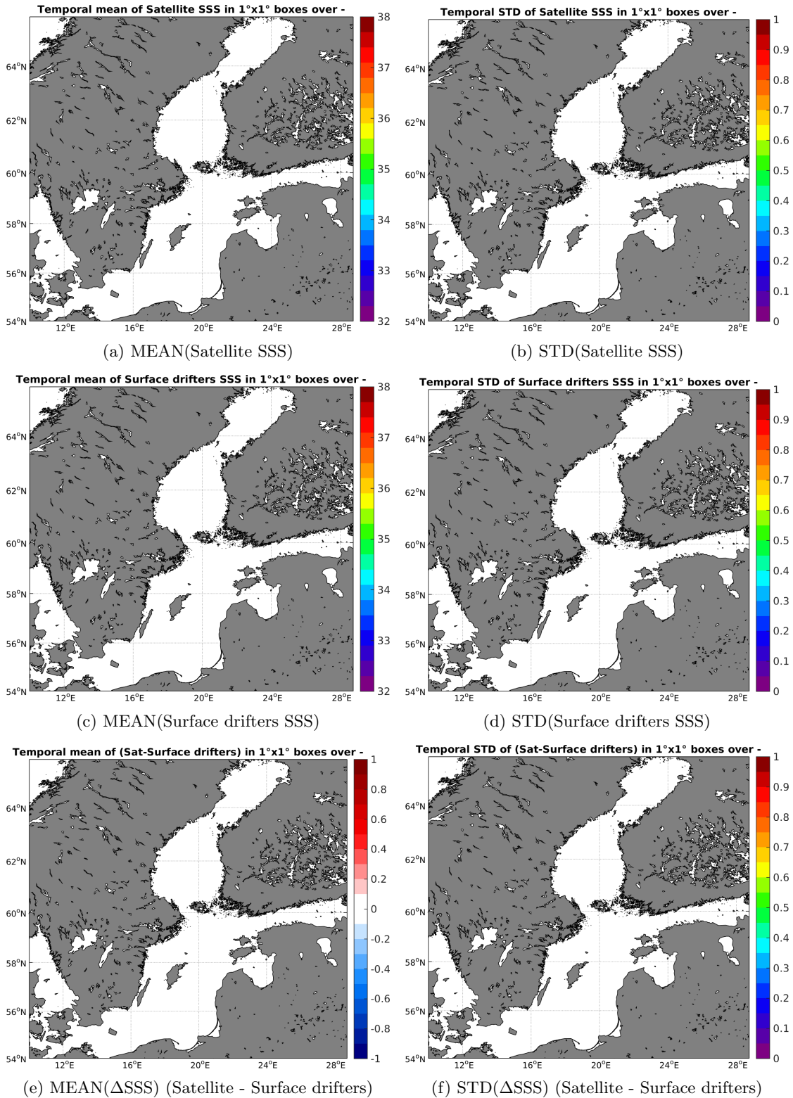
Figure 5: Temporal mean (left) and STD (right) of SSS from AQUARIUS-L2-JPL-V4 (top), Surface drifters (middle), and of \Delta SSS (Satellite - Surface drifters). Only match-up pairs are used to generate these maps.
