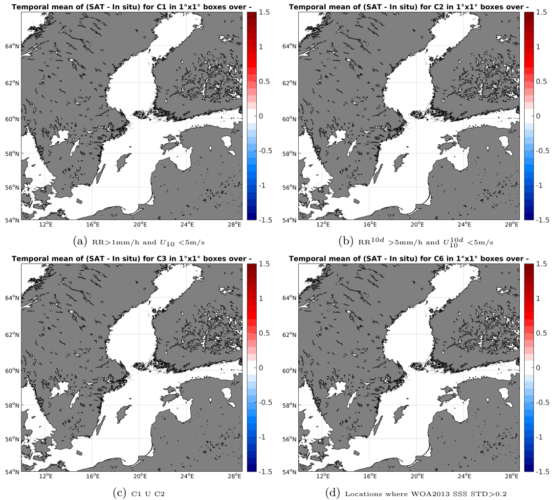
Figure 11: Temporal mean gridded over spatial boxes of size 1^\circ \times 1^\circ of \Delta SSS (AQUARIUS-L2-JPL-V4 - Surface drifters) for 4 different subdatasets corresponding to: RR > 1\text{mm/h} and U_{10} < 5\text{m/s} (a), RR^{10d} > 5\text{mm/h} and U_{10}^{10d} < 5\text{m/s} (b), C1 U C2 (c), Locations where WOA2013 SSS STD > 0.2 (d).
