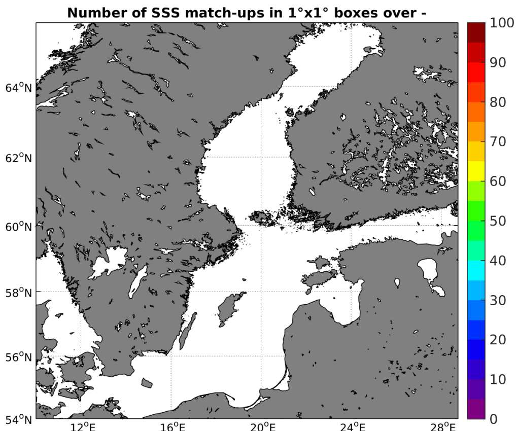
Figure 3: Number of SSS match-ups between Surface drifters SSS and the AQUARIUS-L2-JPL-V4 SSS product for the Baltic Sea Pi-MEP region over 1°x1° boxes and for the full satellite product period.
