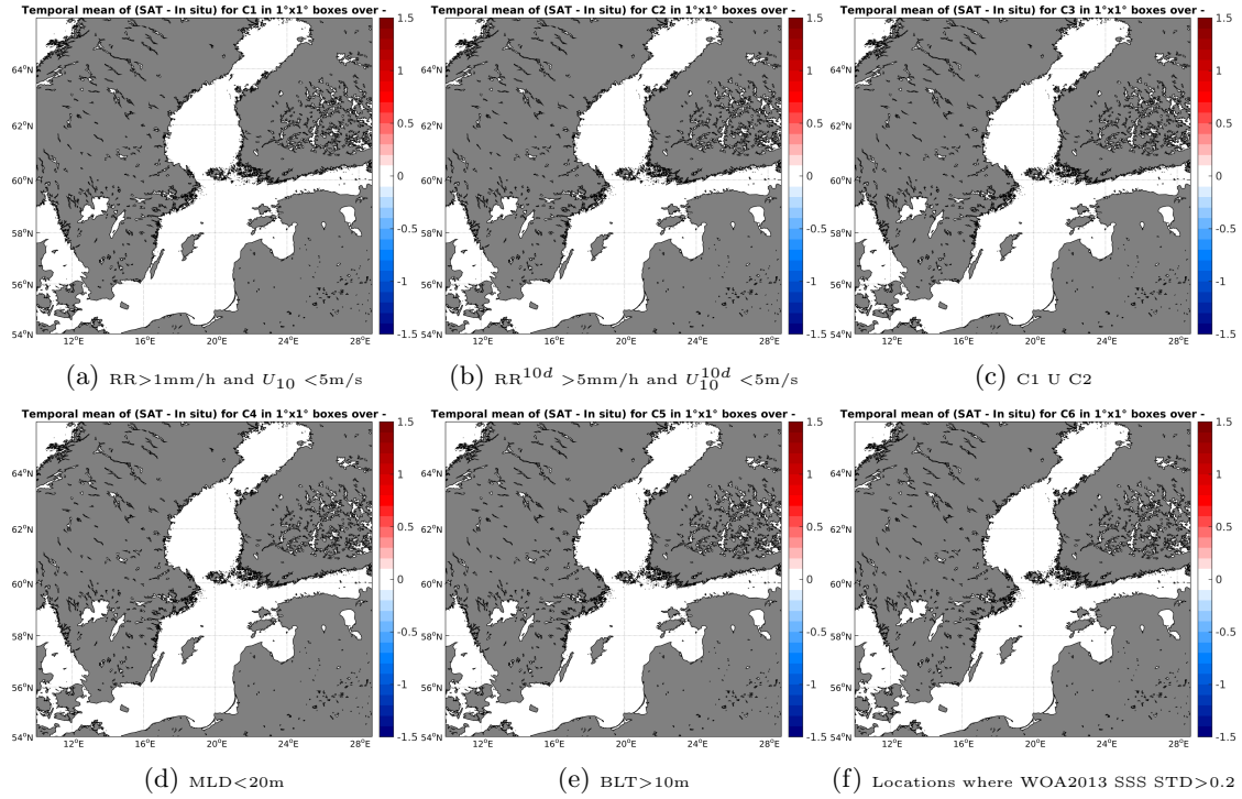
Figure 12: Temporal mean gridded over spatial boxes of size 1^\circ \times 1^\circ of \Delta SSS (AQUARIUS-L2-JPL-V4 - Argo) for 6 different subdatasets corresponding to: RR > 1\text{mm/h} and U_{10} < 5\text{m/s} (a), RR^{10d} > 5\text{mm/h} and U_{10}^{10d} < 5\text{m/s} (b), C1 U C2 (c), MLD < 20\text{m} (d), BLT > 10\text{m} (e), Locations where WOA2013 SSS STD > 0.2 (f).
