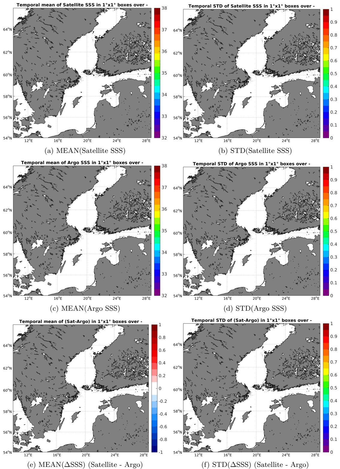
Figure 6: Temporal mean (left) and STD (right) of SSS from AQUARIUS-L2-JPL-V4 (top), Argo (middle), and of \Delta SSS (Satellite - Argo). Only match-up pairs are used to generate these maps.
