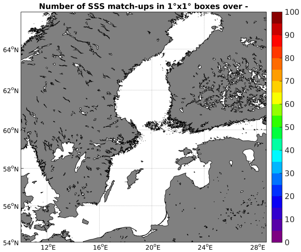
Figure 4: Number of SSS match-ups between Argo SSS and the AQUARIUS-L2-JPL-V4 SSS product for the Baltic Sea Pi-MEP region over 1°x1° boxes and for the full satellite product period.
