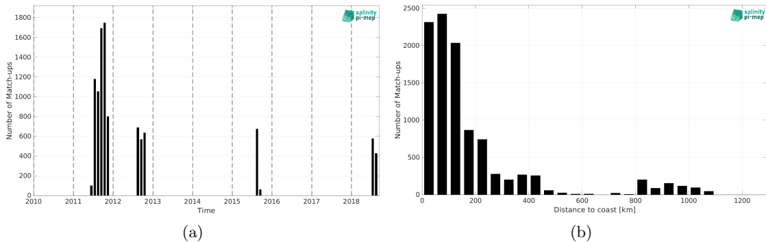
Figure 1: Number of match-ups between TSG (SAMOS) and SMOS and SMAP SSS L4 OI v1 - 7 Days (LOPS) SSS as a function of time (a) and as function of the distance to coast (b) over the Arctic Ocean Pi-MEP region and for the full satellite product period.
