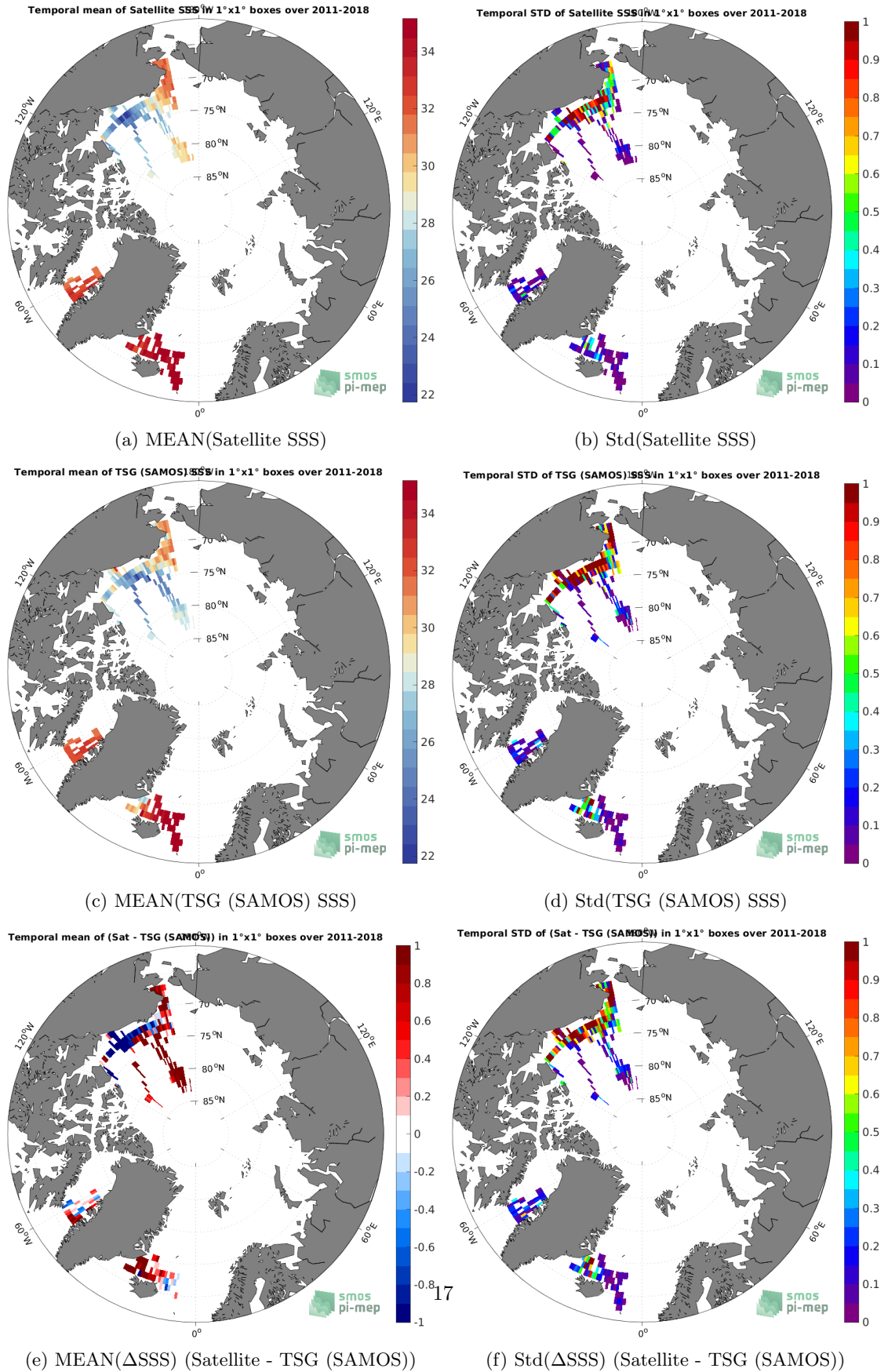
Figure 6: Temporal mean (left) and Std (right) of SSS from SMOS and SMAP SSS L4 OI v1 - 7 Days (LOPS) (top), TSG (SAMOS) (middle), and of \Delta SSS (Satellite - TSG (SAMOS)). Only match-up pairs are used to generate these maps.
