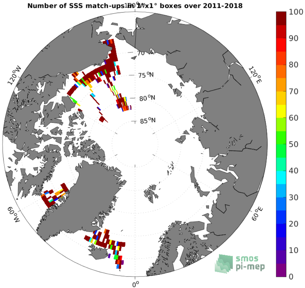
Figure 4: Number of SSS match-ups between TSG (SAMOS) SSS and the SMOS and SMAP SSS L4 OI v1 - 7 Days (LOPS) SSS product for the Arctic Ocean Pi-MEP region over 1^\circ \times 1^\circ boxes and for the full satellite product period.
