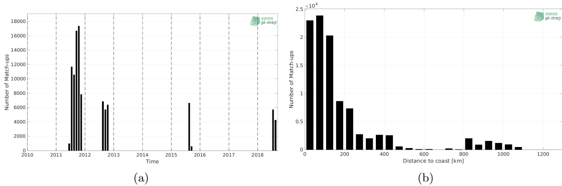
Figure 1: Number of match-ups between TSG (SAMOS) and SMOS and SMAP SSS L4 OI v1 - 7 Days (LOPS) SSS as a function of time (a) and as function of the distance to coast (b) over the Arctic Ocean Pi-MEP region and for the full satellite product period.
