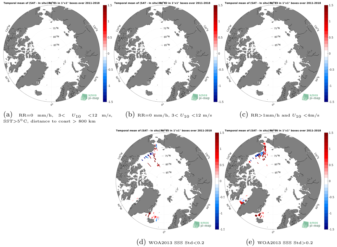
Figure 12: Temporal mean gridded over spatial boxes of size 1^{\circ}\times 1^{\circ} of \Delta\text{SSS} (SMOS and SMAP SSS L4 OI v1 - 7 Days (LOPS) - TSG (SAMOS)) for 5 different subdatasets corresponding to: RR=0 mm/h, 3 < U_{10} < 12 m/s, SST > 5^{\circ}\text{C} , distance to coast > 800 km (a), RR=0 mm/h, 3 < U_{10} < 12 m/s (b), RR > 1 mm/h and U_{10} < 4 m/s (c), WOA2013 SSS Std < 0.2 (d), WOA2013 SSS Std > 0.2 (e).
