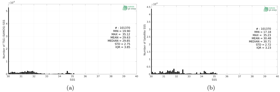
Figure 2: Histograms of SSS from TSG (SAMOS) (a) and SMOS and SMAP SSS L4 OI v1 - 7 Days (LOPS) (b) considering all match-up pairs per bins of 0.1 over the Arctic Ocean Pi-MEP region and for the full satellite product period.
