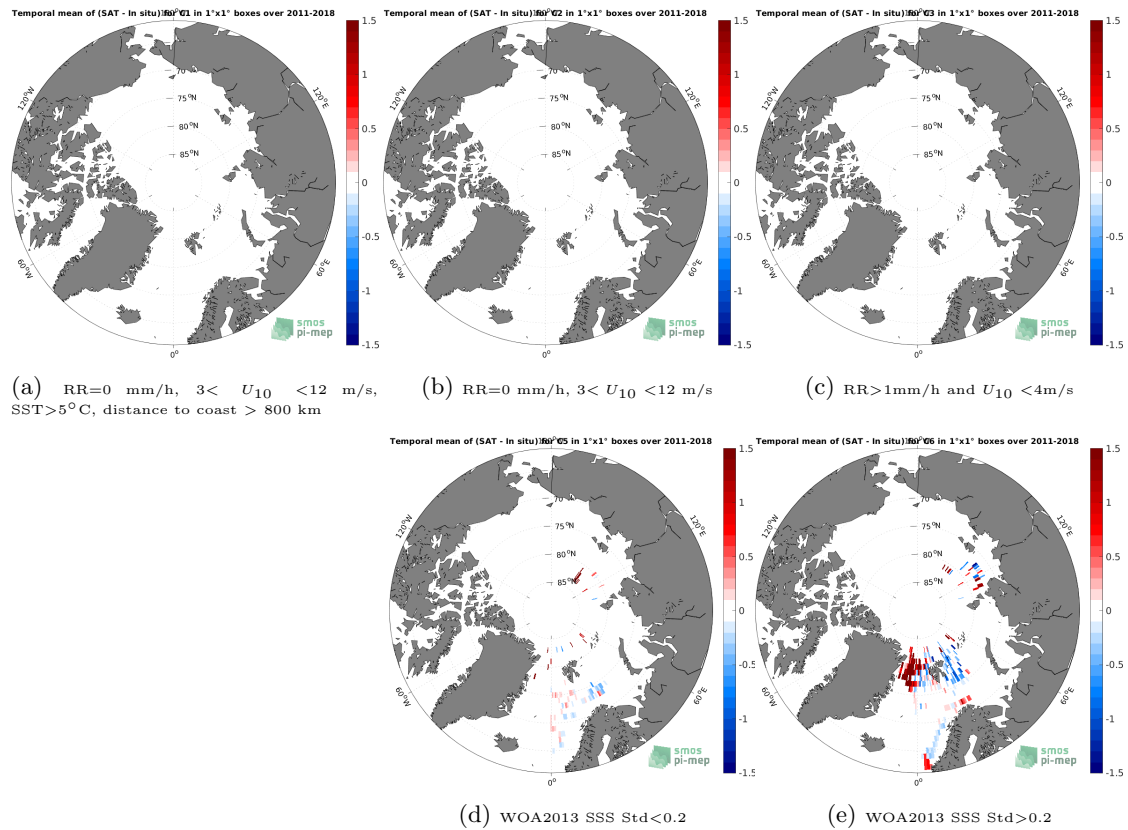
Figure 12: Temporal mean gridded over spatial boxes of size 1^{\circ}\times 1^{\circ} of \Delta\text{SSS} (SMOS and SMAP SSS L4 OI v1 - 7 Days (LOPS) - TSG (Polarstern)) for 5 different subdatasets corresponding to: RR=0 mm/h, 3 < U_{10} < 12 m/s, SST > 5^{\circ}\text{C} , distance to coast > 800 km (a), RR=0 mm/h, 3 < U_{10} < 12 m/s (b), RR > 1 mm/h and U_{10} < 4 m/s (c), WOA2013 SSS Std < 0.2 (d), WOA2013 SSS Std > 0.2 (e).
