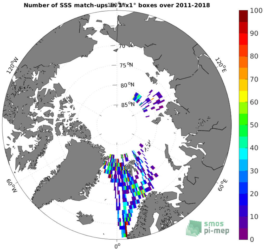
Figure 4: Number of SSS match-ups between TSG (Polarstern) SSS and the SMOS and SMAP SSS L4 OI v1 - 7 Days (LOPS) SSS product for the Arctic Ocean Pi-MEP region over 1^\circ \times 1^\circ boxes and for the full satellite product period.
