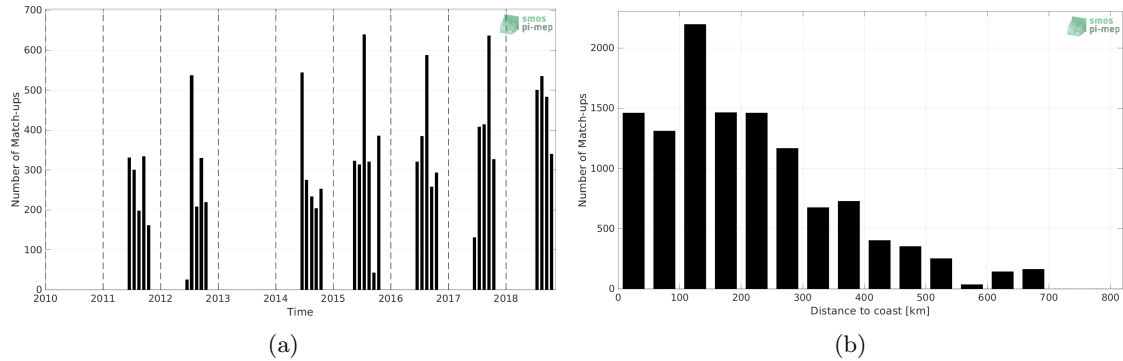
Figure 1: Number of match-ups between TSG (Polarstern) and SMOS and SMAP SSS L4 OI v1 - 7 Days (LOPS) SSS as a function of time (a) and as function of the distance to coast (b) over the Arctic Ocean Pi-MEP region and for the full satellite product period.
