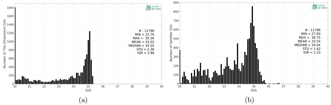
Figure 2: Histograms of SSS from TSG (Polarstern) (a) and SMOS and SMAP SSS L4 OI v1 - 7 Days (LOPS) (b) considering all match-up pairs per bins of 0.1 over the Arctic Ocean Pi-MEP region and for the full satellite product period.
