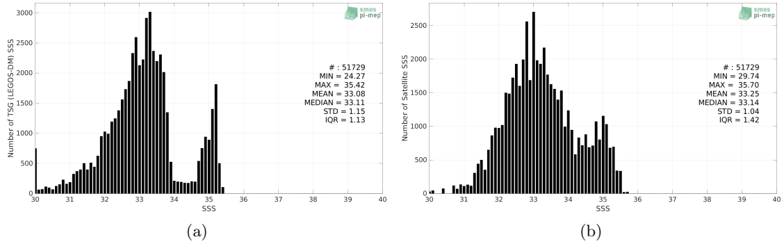
Figure 2: Histograms of SSS from TSG (LEGOS-DM) (a) and SMOS and SMAP SSS L4 OI v1 - 7 Days (LOPS) (b) considering all match-up pairs per bins of 0.1 over the Arctic Ocean Pi-MEP region and for the full satellite product period.
