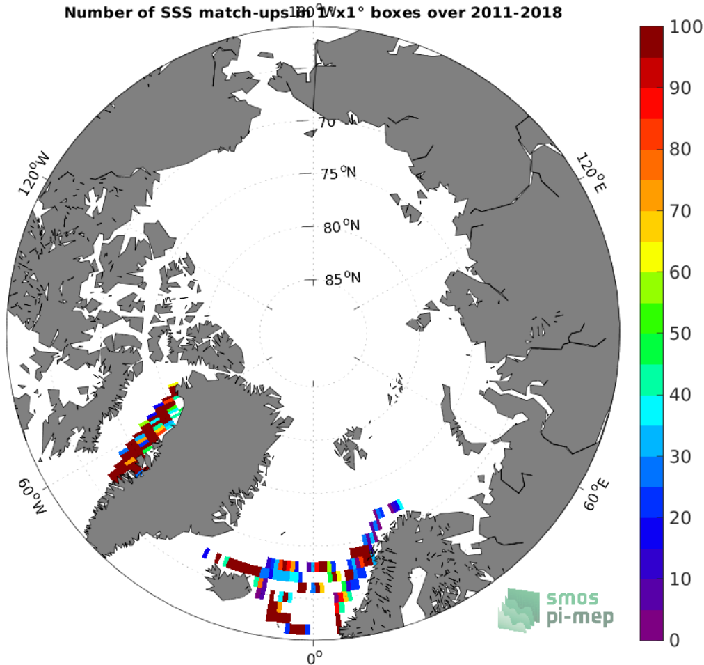
Figure 4: Number of SSS match-ups between TSG (LEGOS-DM) SSS and the SMOS and SMAP SSS L4 OI v1 - 7 Days (LOPS) SSS product for the Arctic Ocean Pi-MEP region over 1^\circ \times 1^\circ boxes and for the full satellite product period.
