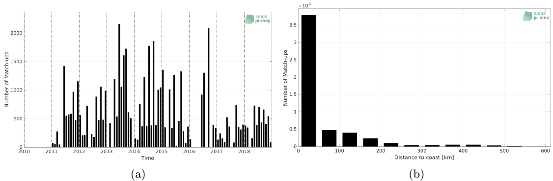
Figure 1: Number of match-ups between TSG (LEGOS-DM) and SMOS and SMAP SSS L4 OI v1 - 7 Days (LOPS) SSS as a function of time (a) and as function of the distance to coast (b) over the Arctic Ocean Pi-MEP region and for the full satellite product period.
