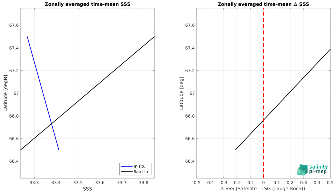
Figure 8: Left panel: Zonal mean SSS from SMOS and SMAP SSS L4 OI v1 - 7 Days (LOPS) satellite product (black) and from TSG (Lauge-Koch) (blue). Right panel: Zonal mean of \Delta SSS (Satellite - TSG (Lauge-Koch)) for all the collected Pi-MEP match-up pairs estimated over the full satellite product period.
