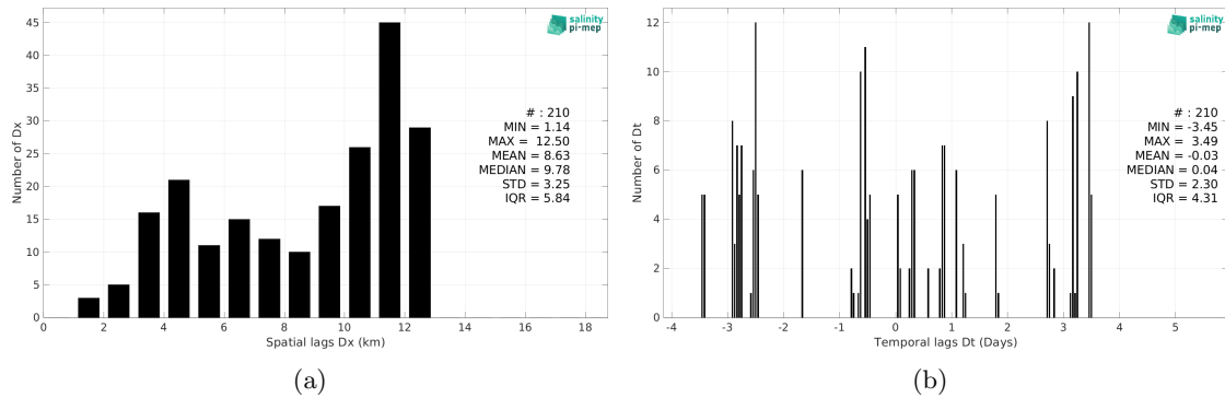
Figure 5: Histograms of the spatial (a) and temporal (b) lags between the location/time of the TSG (Lauge-Koch) measurement and the date of the corresponding SMOS and SMAP SSS L4 OI v1 - 7 Days (LOPS) SSS pixel.
