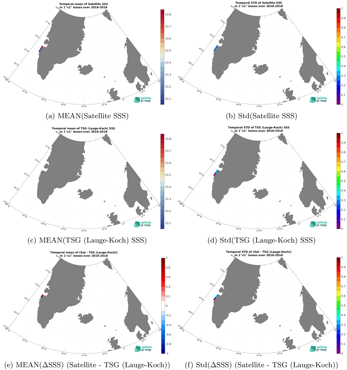
Figure 6: Temporal mean (left) and Std (right) of SSS from SMOS and SMAP SSS L4 OI v1 - 7 Days (LOPS) (top), TSG (Lauge-Koch) (middle), and of \Delta SSS (Satellite - TSG (Lauge-Koch)). Only match-up pairs are used to generate these maps.
