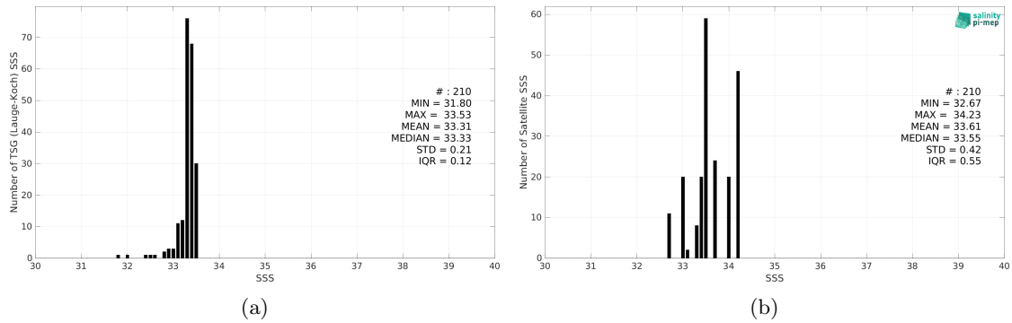
Figure 2: Histograms of SSS from TSG (Lauge-Koch) (a) and SMOS and SMAP SSS L4 OI v1 - 7 Days (LOPS) (b) considering all match-up pairs per bins of 0.1 over the Arctic Ocean Pi-MEP region and for the full satellite product period.
