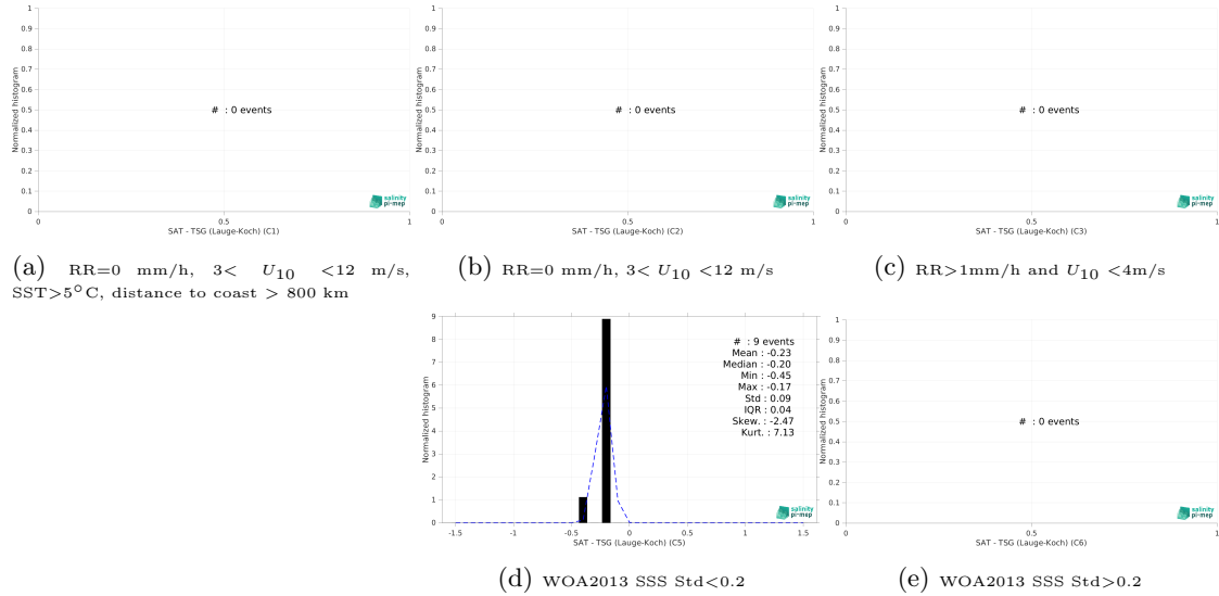
Figure 13: Normalized histogram of \Delta SSS (SMOS and SMAP SSS L4 OI v1 - 7 Days (LOPS) - TSG (Lauge-Koch)) for 5 different subdatasets corresponding to: RR=0 mm/h, 3 < U_{10} < 12 m/s, SST>5°C, distance to coast > 800 km (a), RR=0 mm/h, 3 < U_{10} < 12 m/s (b), RR>1mm/h and U_{10} < 4 m/s (c), WOA2013 SSS Std<0.2 (d), WOA2013 SSS Std>0.2 (e).
