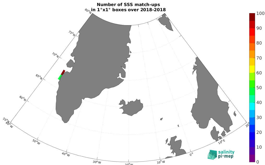
Figure 4: Number of SSS match-ups between TSG (Lauge-Koch) SSS and the SMOS and SMAP SSS L4 OI v1 - 7 Days (LOPS) SSS product for the Arctic Ocean Pi-MEP region over 1^\circ \times 1^\circ boxes and for the full satellite product period.
