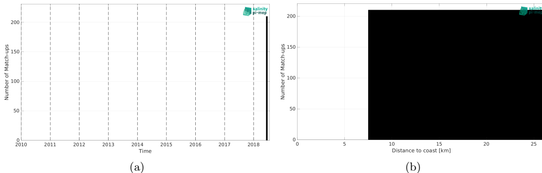
Figure 1: Number of match-ups between TSG (Lauge-Koch) and SMOS and SMAP SSS L4 OI v1 - 7 Days (LOPS) SSS as a function of time (a) and as function of the distance to coast (b) over the Arctic Ocean Pi-MEP region and for the full satellite product period.
