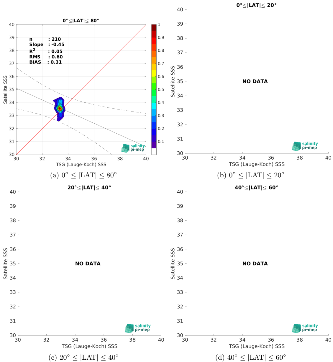
Figure 9: Contour maps of the concentration of SMOS and SMAP SSS L4 OI v1 - 7 Days (LOPS) SSS (y-axis) versus TSG (Lauge-Koch) SSS (x-axis) at match-up pairs for different latitude bands. For each plot, the red line shows x=y . The black thin and dashed lines indicate a linear fit through the data cloud and the \pm 95\% confidence levels, respectively. The number match-up pairs n , the slope and R^2 coefficient of the linear fit, the root mean square (RMS) and the mean bias between satellite and in situ data are indicated for each latitude band in each plots.
