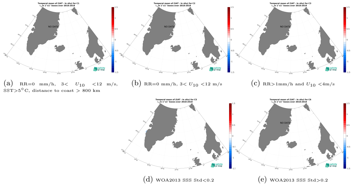
Figure 12: Temporal mean gridded over spatial boxes of size 1^{\circ}\times 1^{\circ} of \Delta\text{SSS} (SMOS and SMAP SSS L4 OI v1 - 7 Days (LOPS) - TSG (Lauge-Koch)) for 5 different subdatasets corresponding to:RR=0 mm/h, 3 < U_{10} < 12 m/s, SST >5^{\circ}\text{C} , distance to coast > 800 km (a), RR=0 mm/h, 3 < U_{10} < 12 m/s (b), RR >1 mm/h and U_{10} < 4 m/s (c), WOA2013 SSS Std <0.2 (d), WOA2013 SSS Std >0.2 (e).
