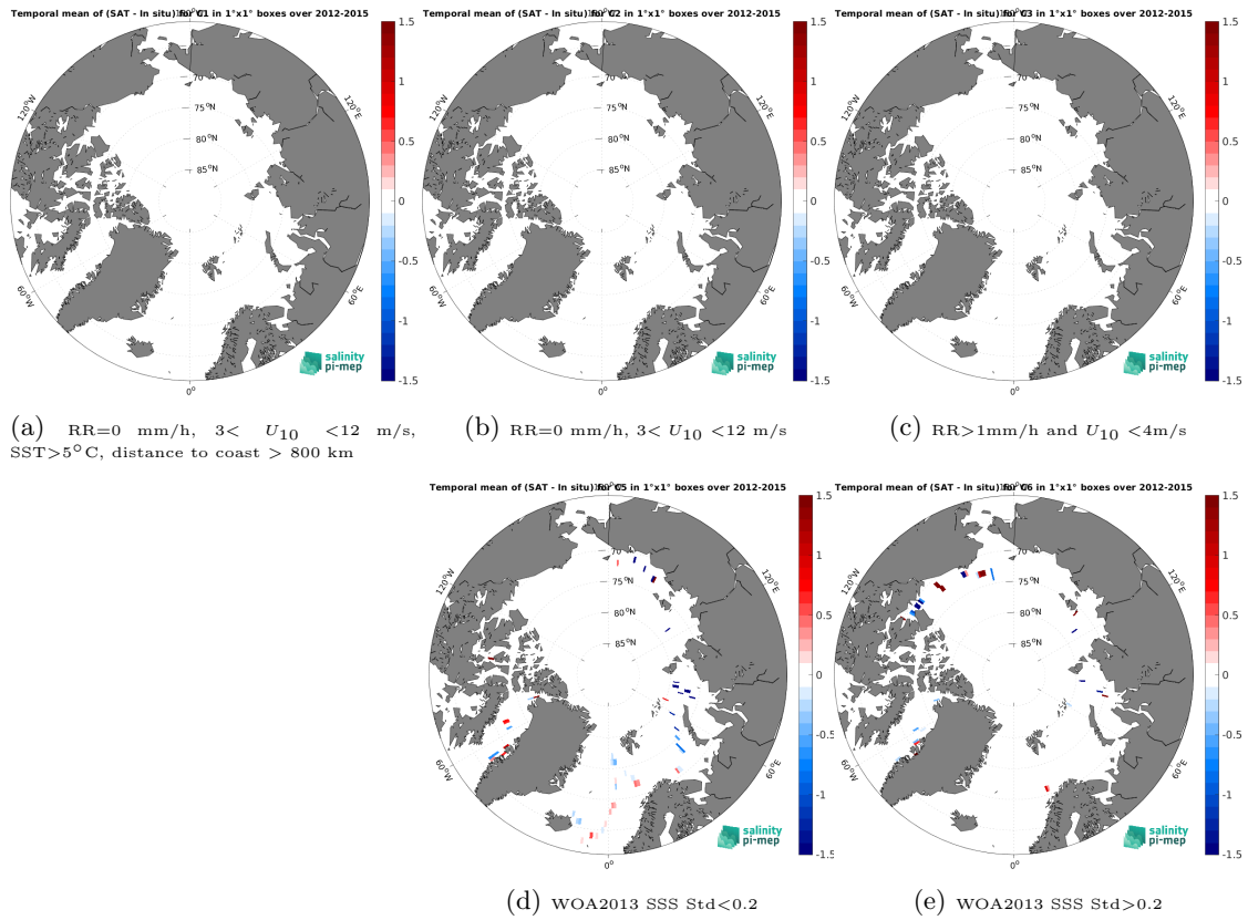
Figure 12: Temporal mean gridded over spatial boxes of size 1^\circ \times 1^\circ of \Delta\text{SSS} (SMOS and SMAP SSS L4 OI v1 - 7 Days (LOPS) - TSG (GOSUD-Sailing-ship)) for 5 different subdatasets corresponding to: RR=0 mm/h, 3 < U_{10} < 12 m/s, SST > 5^\circ\text{C} , distance to coast > 800 km (a), RR=0 mm/h, 3 < U_{10} < 12 m/s (b), RR > 1 mm/h and U_{10} < 4 m/s (c), WOA2013 SSS Std < 0.2 (d), WOA2013 SSS Std > 0.2 (e).
