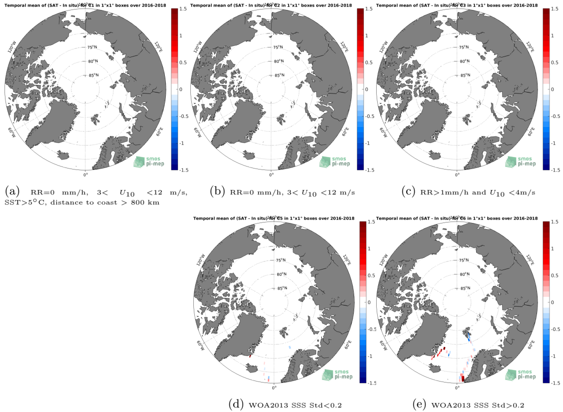
Figure 12: Temporal mean gridded over spatial boxes of size 1^\circ \times 1^\circ of \Delta SSS (SMOS and SMAP SSS L4 OI v1 - 7 Days (LOPS) - TSG (GOSUD-Research-vessel)) for 5 different subdatasets corresponding to: RR=0 mm/h, 3 < U_{10} < 12 m/s, SST > 5°C, distance to coast > 800 km (a), RR=0 mm/h, 3 < U_{10} < 12 m/s (b), RR > 1mm/h and U_{10} < 4 m/s (c), WOA2013 SSS Std < 0.2 (d), WOA2013 SSS Std > 0.2 (e).
