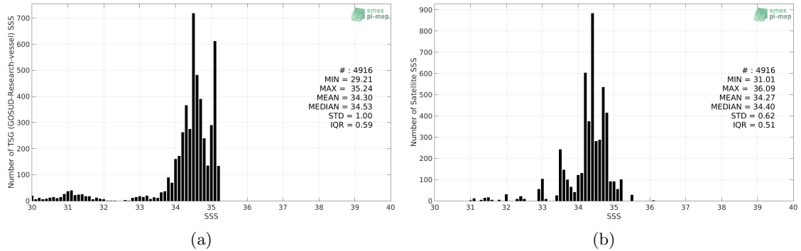
Figure 2: Histograms of SSS from TSG (GOSUD-Research-vessel) (a) and SMOS and SMAP SSS L4 OI v1 - 7 Days (LOPS) (b) considering all match-up pairs per bins of 0.1 over the Arctic Ocean Pi-MEP region and for the full satellite product period.
