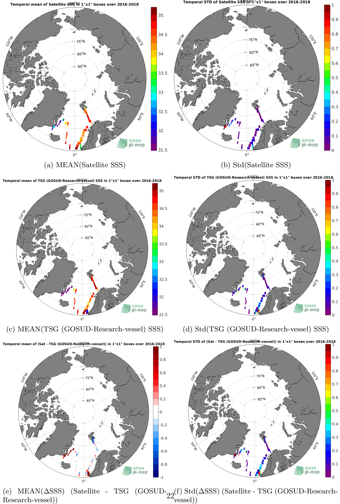
Figure 6: Temporal mean (left) and Std (right) of SSS from SMOS and SMAP SSS L4 OI v1 - 7 Days (LOPS) (top), TSG (GOSUD-Research-vessel) (middle), and of \Delta SSS (Satellite - TSG (GOSUD-Research-vessel)). Only match-up pairs are used to generate these maps.
