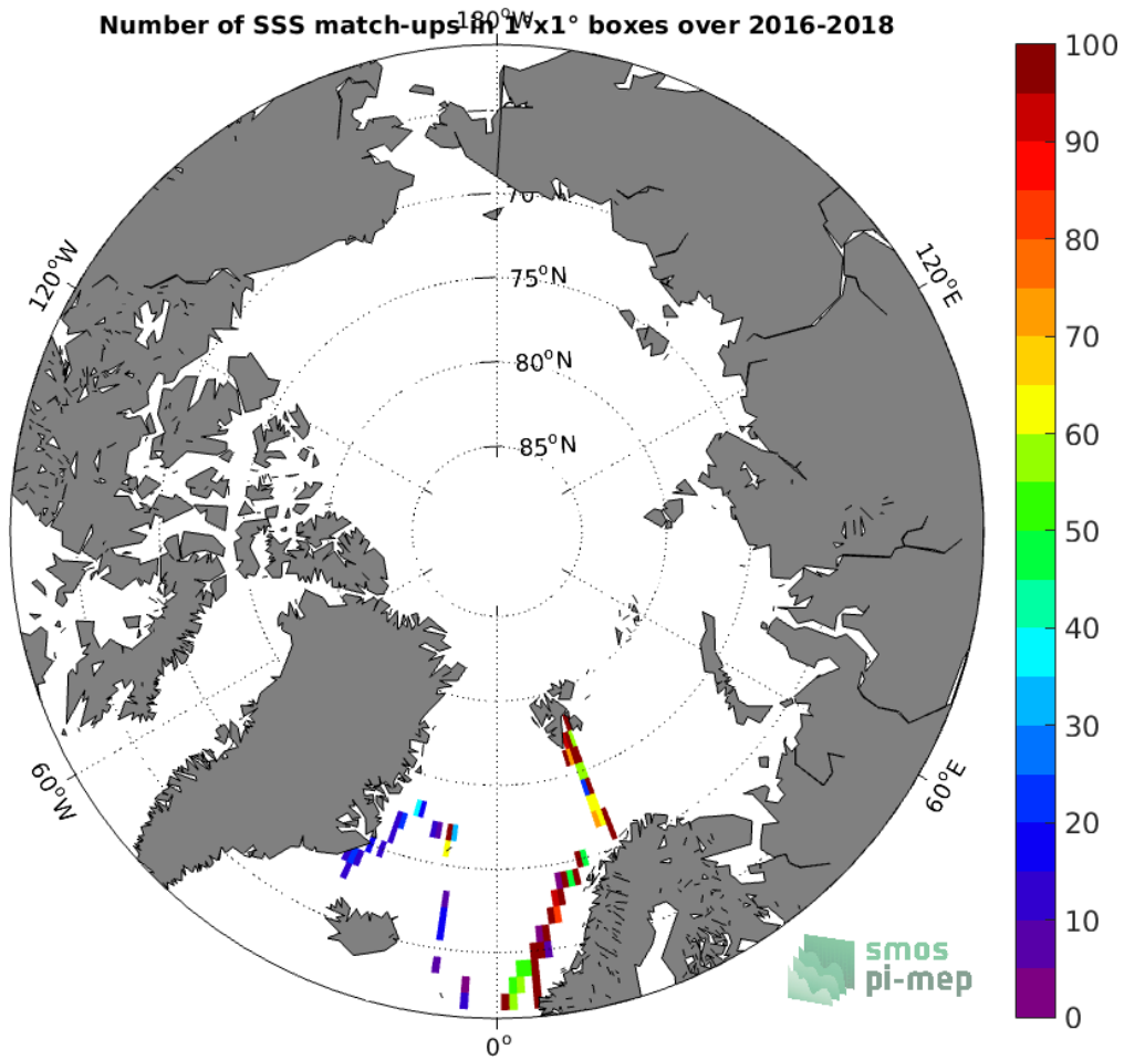
Figure 4: Number of SSS match-ups between TSG (GOSUD-Research-vessel) SSS and the SMOS and SMAP SSS L4 OI v1 - 7 Days (LOPS) SSS product for the Arctic Ocean Pi-MEP region over 1^\circ \times 1^\circ boxes and for the full satellite product period.
