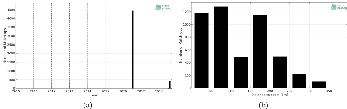
Figure 1: Number of match-ups between TSG (GOSUD-Research-vessel) and SMOS and SMAP SSS L4 OI v1 - 7 Days (LOPS) SSS as a function of time (a) and as function of the distance to coast (b) over the Arctic Ocean Pi-MEP region and for the full satellite product period.
