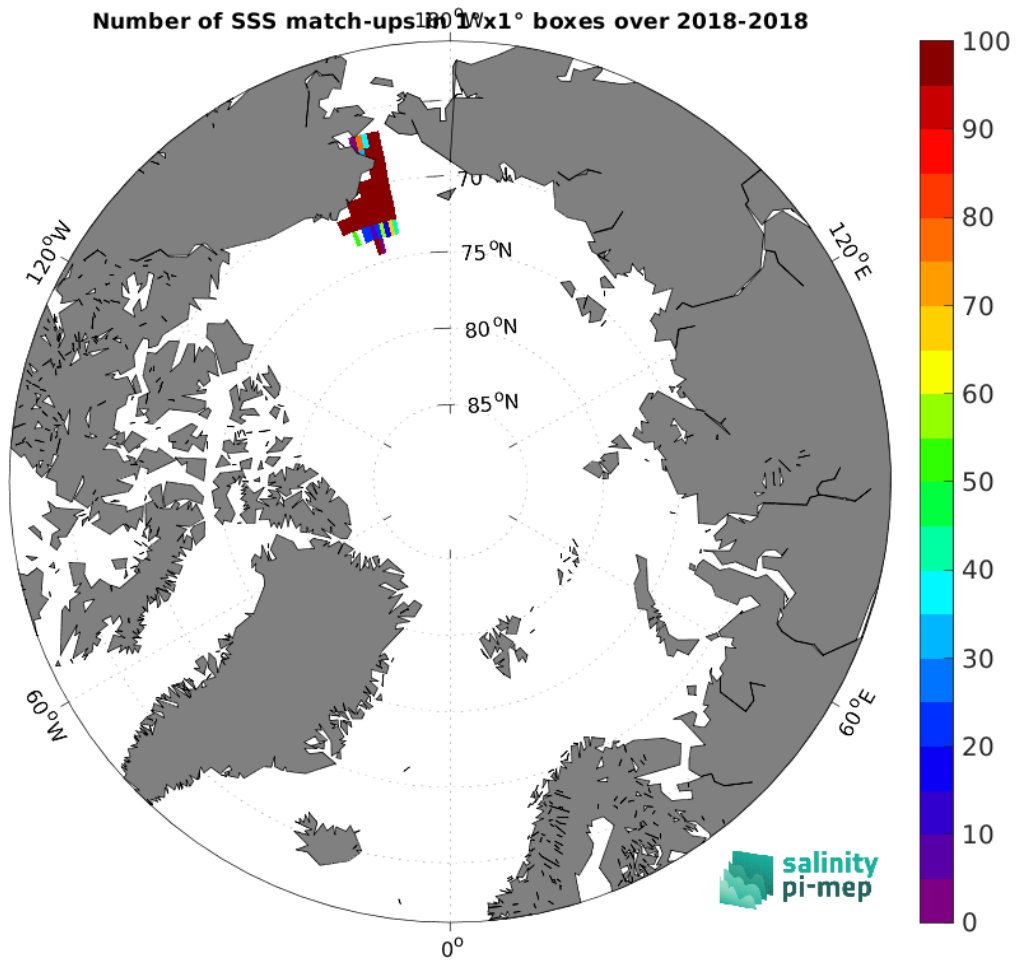
Figure 4: Number of SSS match-ups between Saildrone SSS and the SMOS and SMAP SSS L4 OI v1 - 7 Days (LOPS) SSS product for the Arctic Ocean Pi-MEP region over 1^\circ \times 1^\circ boxes and for the full satellite product period.
