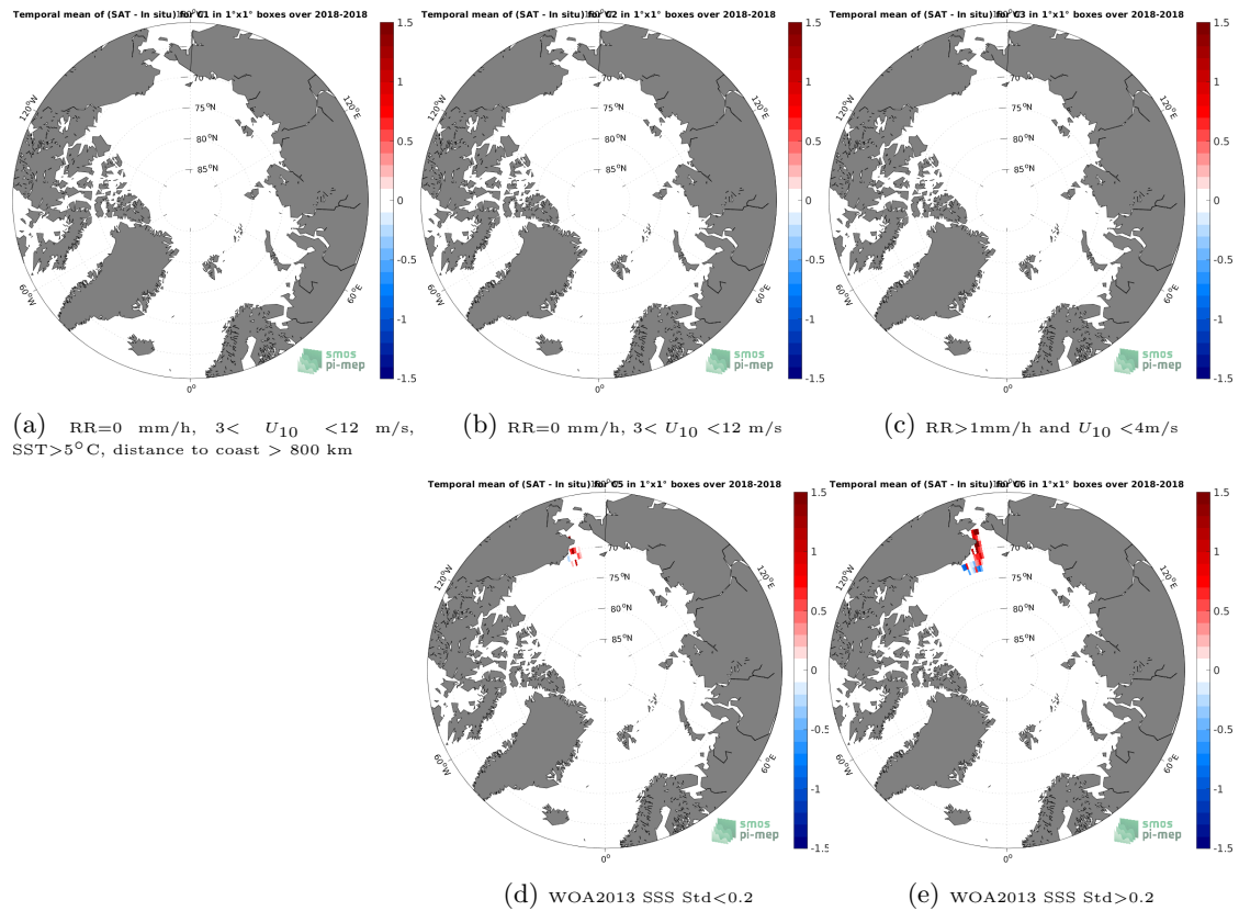
Figure 12: Temporal mean gridded over spatial boxes of size 1^{\circ}\times 1^{\circ} of \Delta\text{SSS} (SMOS and SMAP SSS L4 OI v1 - 7 Days (LOPS) - Sairdrone) for 5 different subdatasets corresponding to:RR=0 mm/h, 3 < U_{10} < 12 m/s, SST > 5^{\circ}\text{C} , distance to coast > 800 km (a), RR=0 mm/h, 3 < U_{10} < 12 m/s (b), RR > 1 mm/h and U_{10} < 4 m/s (c), WOA2013 SSS Std < 0.2 (d), WOA2013 SSS Std > 0.2 (e).
