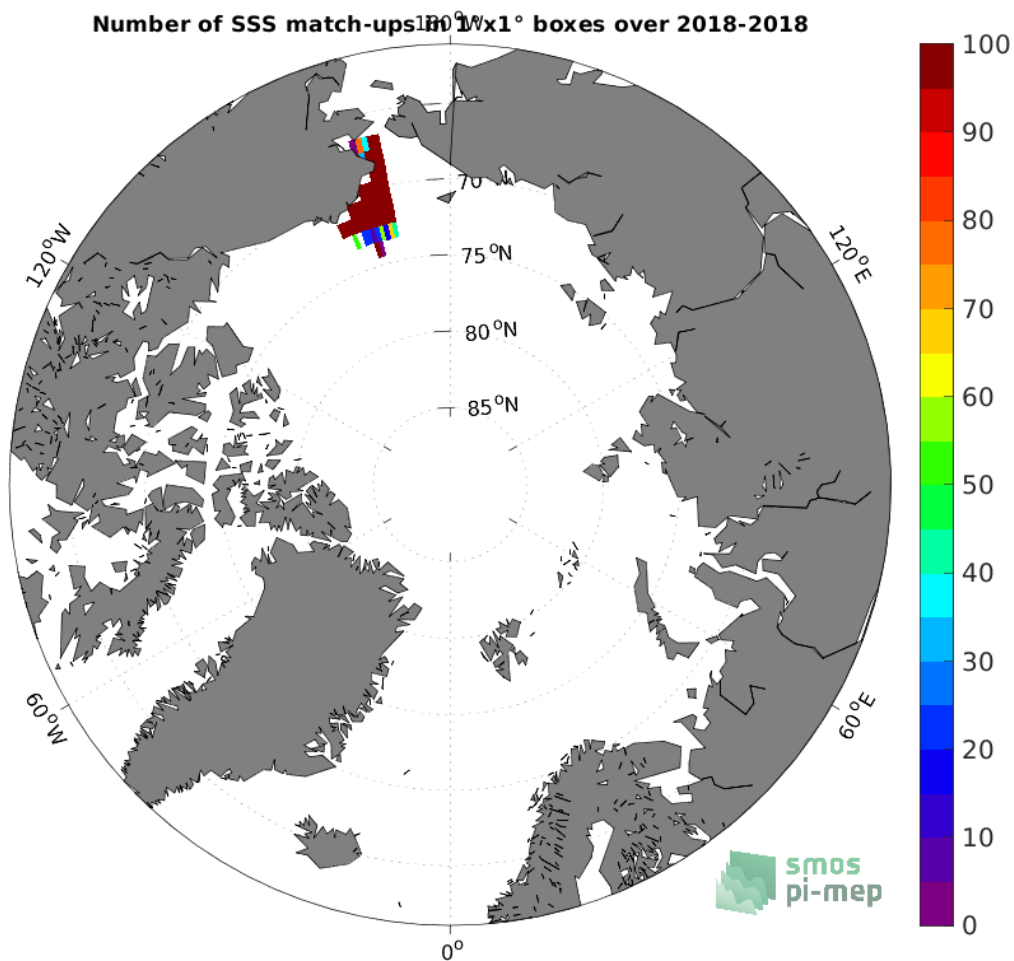
Figure 4: Number of SSS match-ups between Sailldrone SSS and the SMOS and SMAP SSS L4 OI v1 - 7 Days (LOPS) SSS product for the Arctic Ocean Pi-MEP region over 1^\circ \times 1^\circ boxes and for the full satellite product period.
