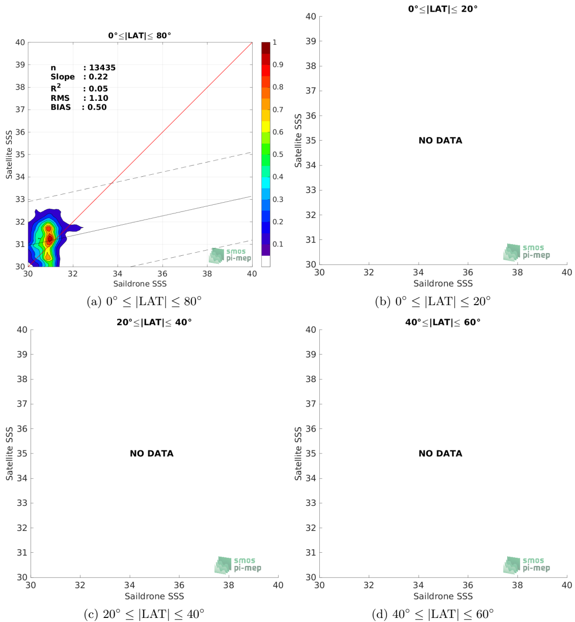
Figure 9: Contour maps of the concentration of SMOS and SMAP SSS L4 OI v1 - 7 Days (LOPS) SSS (y-axis) versus Saildrone SSS (x-axis) at match-up pairs for different latitude bands. For each plot, the red line shows x=y . The black thin and dashed lines indicate a linear fit through the data cloud and the \pm 95\% confidence levels, respectively. The number match-up pairs n , the slope and R^2 coefficient of the linear fit, the root mean square (RMS) and the mean bias between satellite and in situ data are indicated for each latitude band in each plots.
