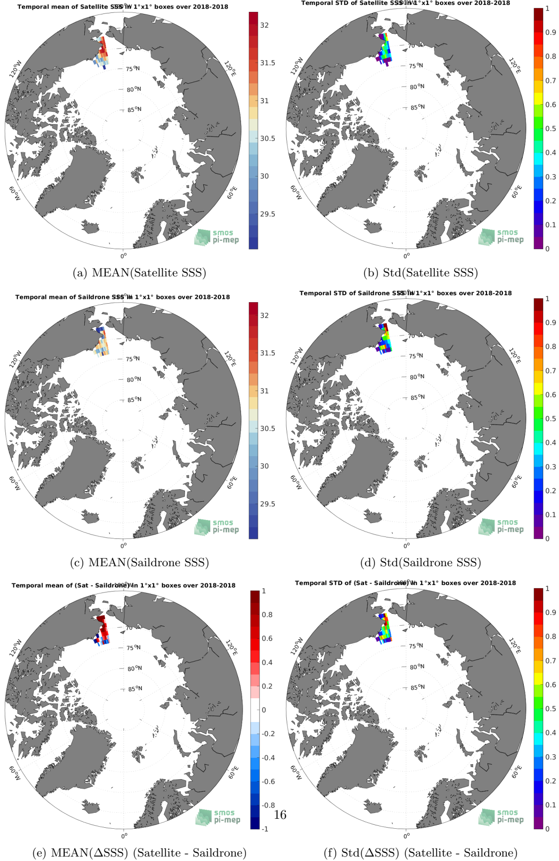
Figure 6: Temporal mean (left) and Std (right) of SSS from SMOS and SMAP SSS L4 OI v1 - 7 Days (LOPS) (top), Saildrone (middle), and of \Delta SSS (Satellite - Saildrone). Only match-up pairs are used to generate these maps.
