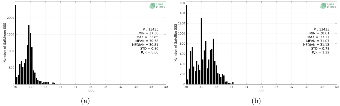
Figure 2: Histograms of SSS from Sairdrone (a) and SMOS and SMAP SSS L4 OI v1 - 7 Days (LOPS) (b) considering all match-up pairs per bins of 0.1 over the Arctic Ocean Pi-MEP region and for the full satellite product period.
