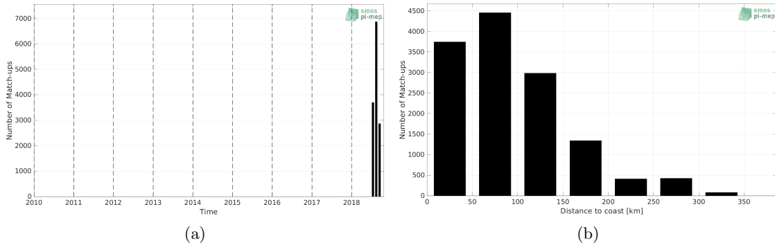
Figure 1: Number of match-ups between Saildrone and SMOS and SMAP SSS L4 OI v1 - 7 Days (LOPS) SSS as a function of time (a) and as function of the distance to coast (b) over the Arctic Ocean Pi-MEP region and for the full satellite product period.
