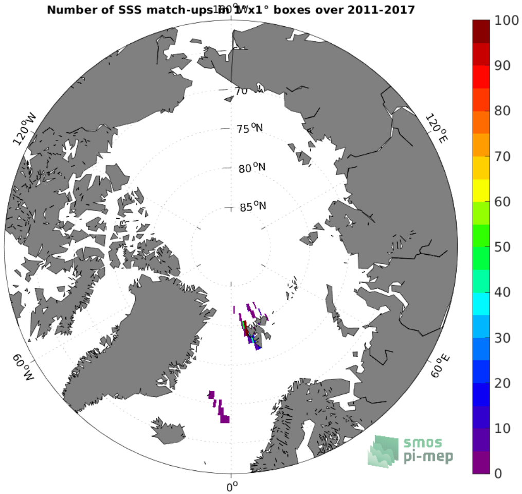
Figure 4: Number of SSS match-ups between Marine mammals SSS and the SMOS and SMAP SSS L4 OI v1 - 7 Days (LOPS) SSS product for the Arctic Ocean Pi-MEP region over 1^{\circ} \times 1^{\circ} boxes and for the full satellite product period.
