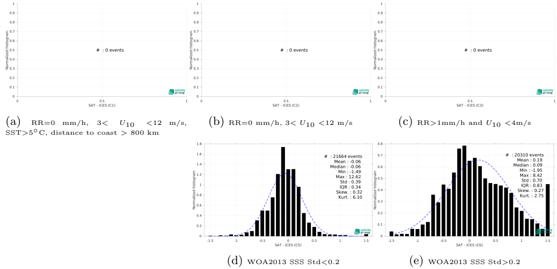
Figure 13: Normalized histogram of \Delta SSS (SMOS and SMAP SSS L4 OI v1 - 7 Days (LOPS) - ICES) for 5 different subdatasets corresponding to: RR=0 mm/h, 3 < U_{10} < 12 m/s, SST>5°C, distance to coast > 800 km (a), RR=0 mm/h, 3 < U_{10} < 12 m/s (b), RR>1mm/h and U_{10} < 4 m/s (c), WOA2013 SSS Std<0.2 (d), WOA2013 SSS Std>0.2 (e).
