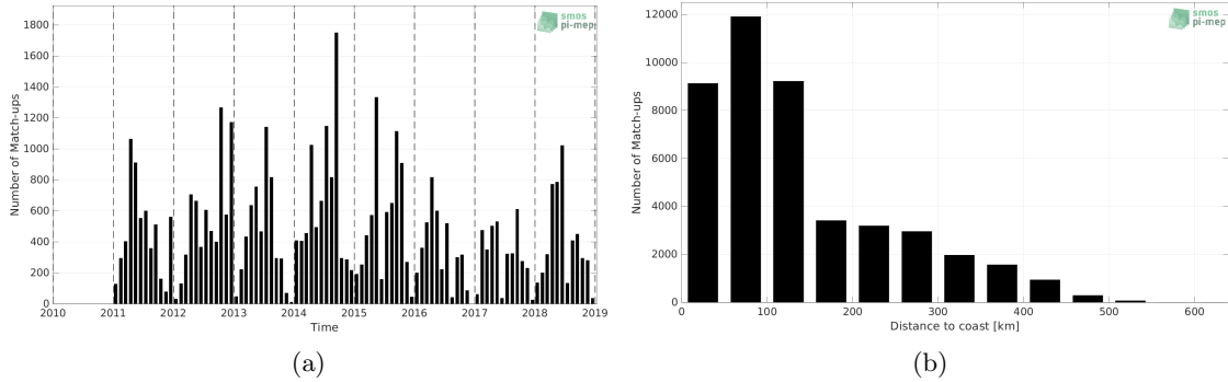
Figure 1: Number of match-ups between ICES and SMOS and SMAP SSS L4 OI v1 - 7 Days (LOPS) SSS as a function of time (a) and as function of the distance to coast (b) over the Arctic Ocean Pi-MEP region and for the full satellite product period.
