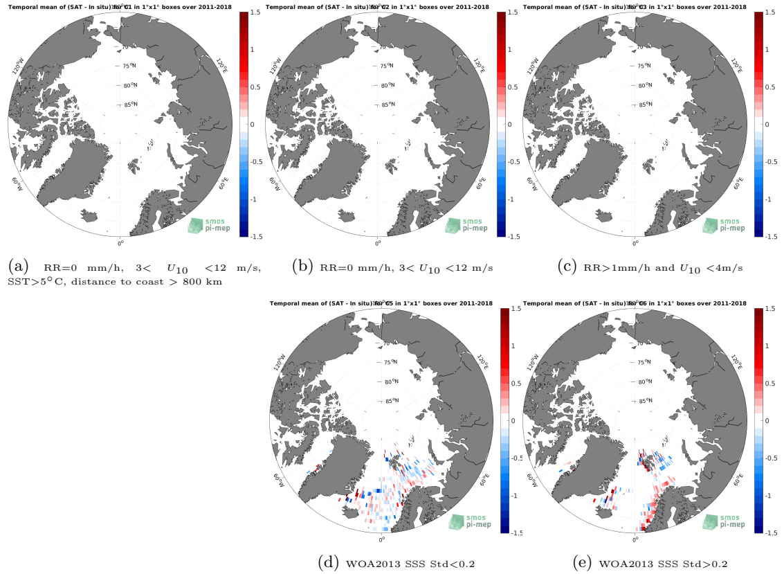
Figure 12: Temporal mean gridded over spatial boxes of size 1^{\circ}\times 1^{\circ} of \Delta\text{SSS} (SMOS and SMAP SSS L4 OI v1 - 7 Days (LOPS) - ICES) for 5 different subdatasets corresponding to:RR=0 mm/h, 3 < U_{10} < 12 m/s, SST > 5^{\circ}\text{C} , distance to coast > 800 km (a), RR=0 mm/h, 3 < U_{10} < 12 m/s (b), RR > 1 mm/h and U_{10} < 4 m/s (c), WOA2013 SSS Std < 0.2 (d), WOA2013 SSS Std > 0.2 (e).
