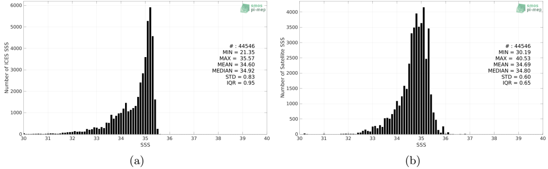
Figure 2: Histograms of SSS from ICES (a) and SMOS and SMAP SSS L4 OI v1 - 7 Days (LOPS) (b) considering all match-up pairs per bins of 0.1 over the Arctic Ocean Pi-MEP region and for the full satellite product period.
