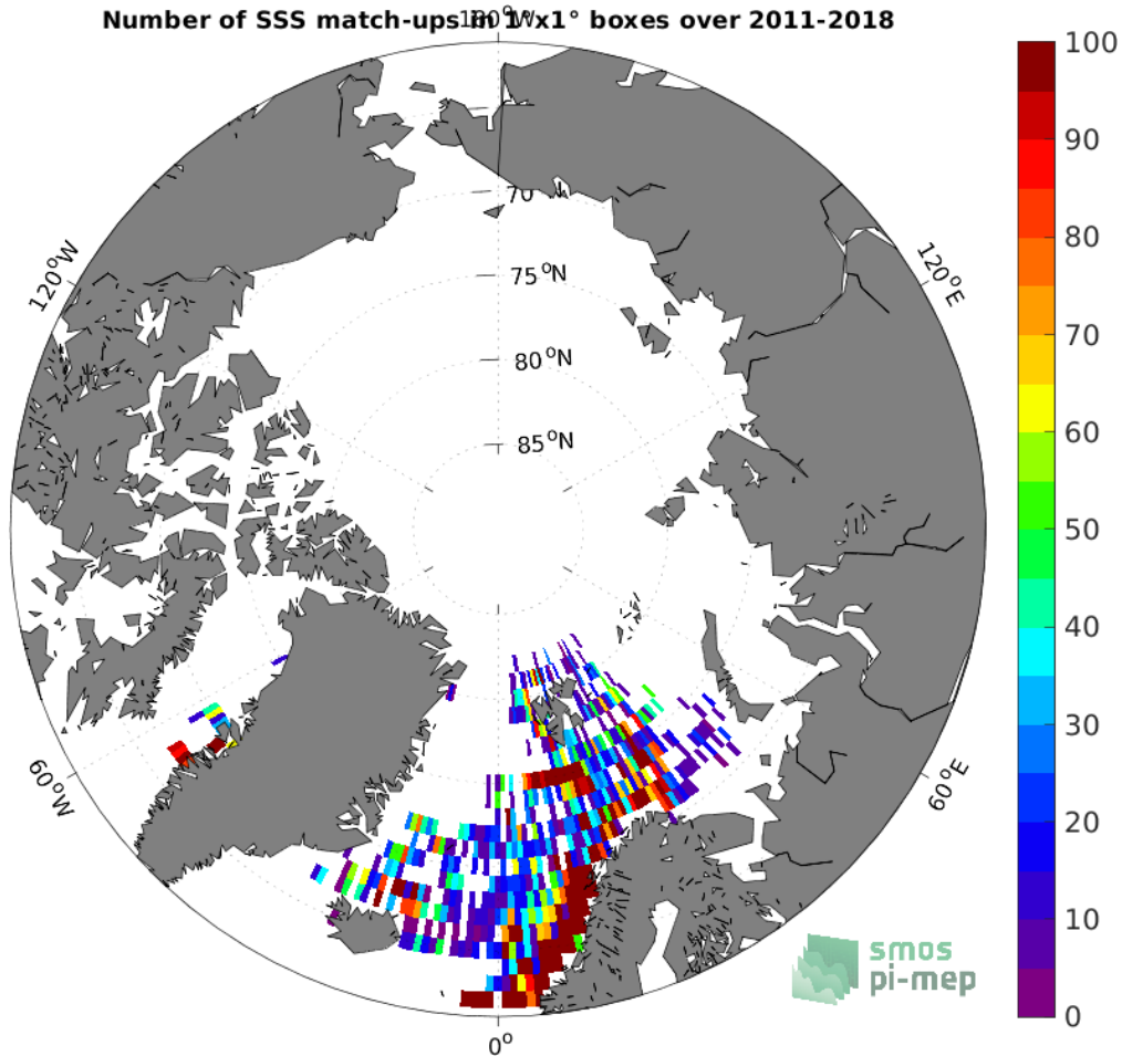
Figure 4: Number of SSS match-ups between ICES SSS and the SMOS and SMAP SSS L4 OI v1 - 7 Days (LOPS) SSS product for the Arctic Ocean Pi-MEP region over 1^\circ \times 1^\circ boxes and for the full satellite product period.
