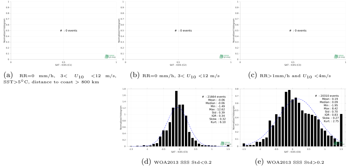
Figure 13: Normalized histogram of \Delta SSS (SMOS and SMAP SSS L4 OI v1 - 7 Days (LOPS) - ICES) for 5 different subdatasets corresponding to: RR=0 mm/h, 3 < U_{10} < 12 m/s, SST>5°C, distance to coast > 800 km (a), RR=0 mm/h, 3 < U_{10} < 12 m/s (b), RR>1mm/h and U_{10} < 4 m/s (c), WOA2013 SSS Std<0.2 (d), WOA2013 SSS Std>0.2 (e).
