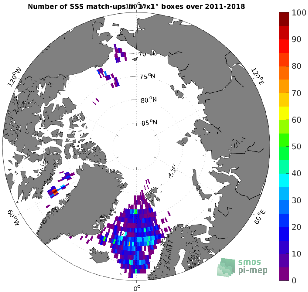
Figure 4: Number of SSS match-ups between Argo SSS and the SMOS and SMAP SSS L4 OI v1 - 7 Days (LOPS) SSS product for the Arctic Ocean Pi-MEP region over 1^{\circ} \times 1^{\circ} boxes and for the full satellite product period.
