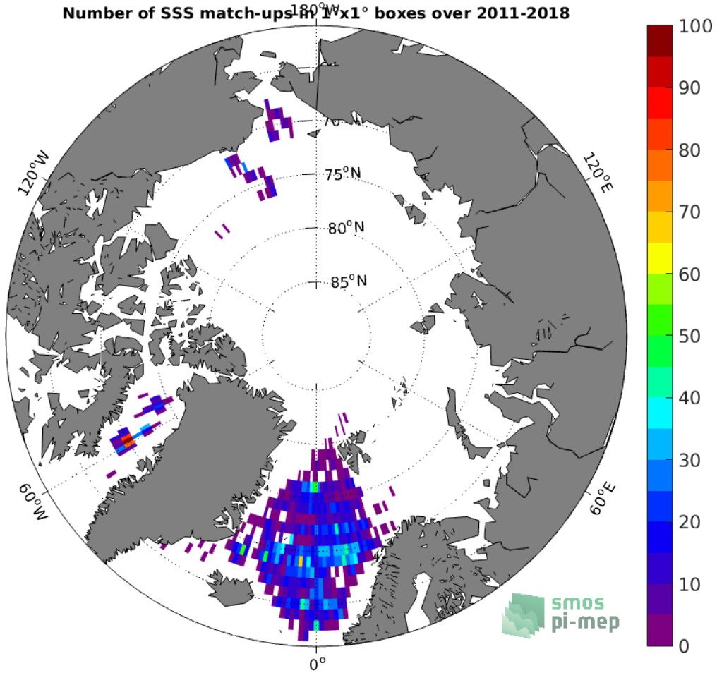
Figure 4: Number of SSS match-ups between Argo SSS and the SMOS and SMAP SSS L4 OI v1 - 7 Days (LOPS) SSS product for the Arctic Ocean Pi-MEP region over 1^\circ \times 1^\circ boxes and for the full satellite product period.
