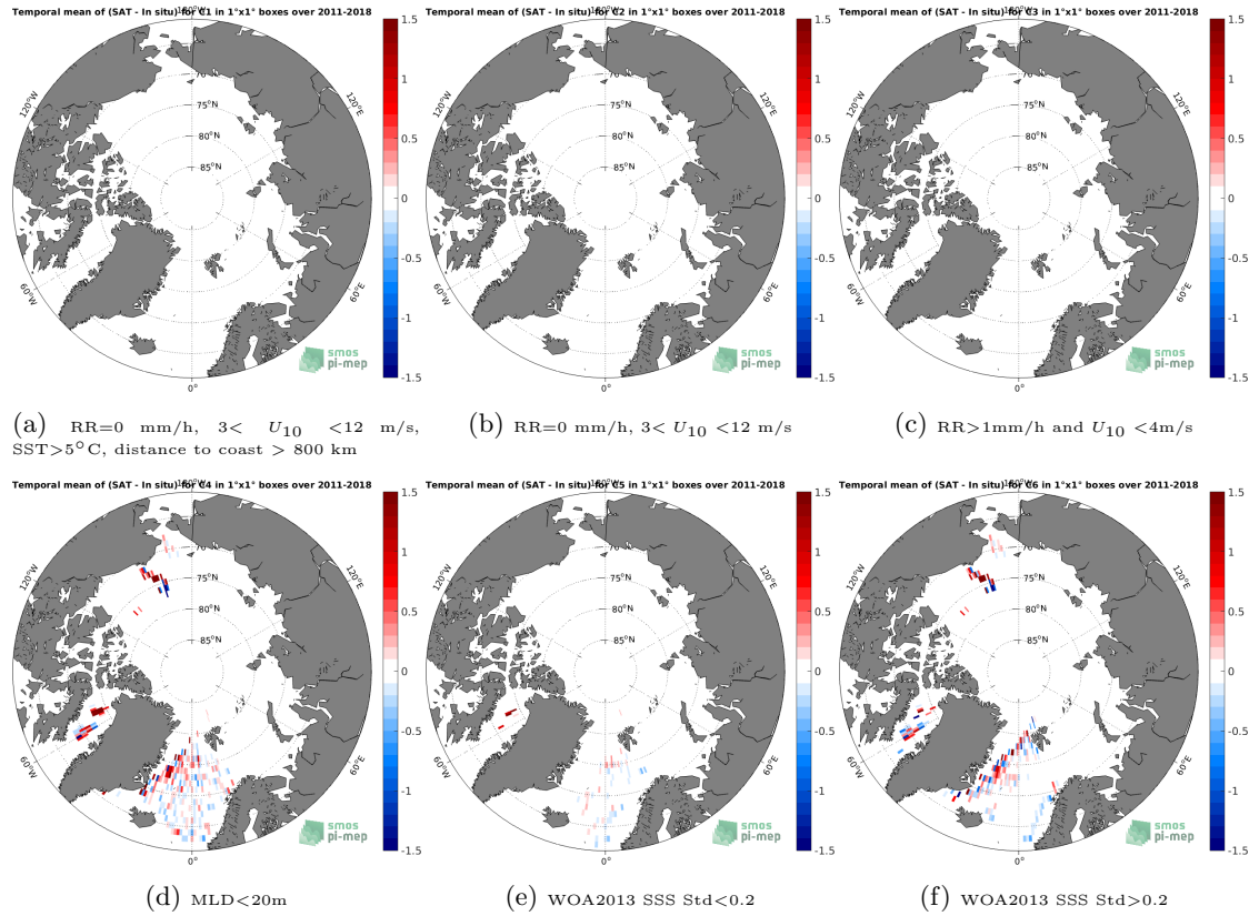
Figure 12: Temporal mean gridded over spatial boxes of size 1^{\circ} \times 1^{\circ} of \Delta\text{SSS} (SMOS and SMAP SSS L4 OI v1 - 7 Days (LOPS) - Argo) for 6 different subdatasets corresponding to: RR=0 mm/h, 3 < U_{10} < 12 m/s, SST > 5^{\circ}\text{C} , distance to coast > 800 km (a), RR=0 mm/h, 3 < U_{10} < 12 m/s (b), RR > 1 mm/h and U_{10} < 4 m/s (c), MLD < 20\text{m} (d), WOA2013 SSS Std < 0.2 (e), WOA2013 SSS Std > 0.2 (f).
