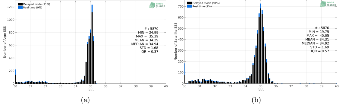
Figure 2: Histograms of SSS from Argo (a) and SMOS and SMAP SSS L4 OI v1 - 7 Days (LOPS) (b) considering all match-up pairs per bins of 0.1 over the Arctic Ocean Pi-MEP region and for the full satellite product period.
