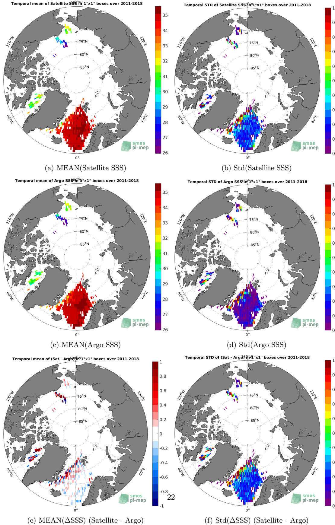
Figure 6: Temporal mean (left) and Std (right) of SSS from SMOS and SMAP SSS L4 OI v1 - 7 Days (LOPS) (top), Argo (middle), and of \Delta SSS (Satellite - Argo). Only match-up pairs are used to generate these maps.
