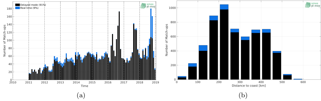
Figure 1: Number of match-ups between Argo and SMOS and SMAP SSS L4 OI v1 - 7 Days (LOPS) SSS as a function of time (a) and as function of the distance to coast (b) over the Arctic Ocean Pi-MEP region and for the full satellite product period.
