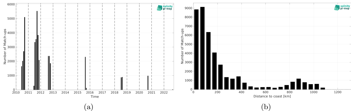
Figure 1: Number of match-ups between TSG (SAMOS) and SMOS SSS L4 v1 - Weekly (CMEMS-CNR) SSS as a function of time (a) and as function of the distance to coast (b) over the Arctic Ocean Pi-MEP region and for the full satellite product period.
