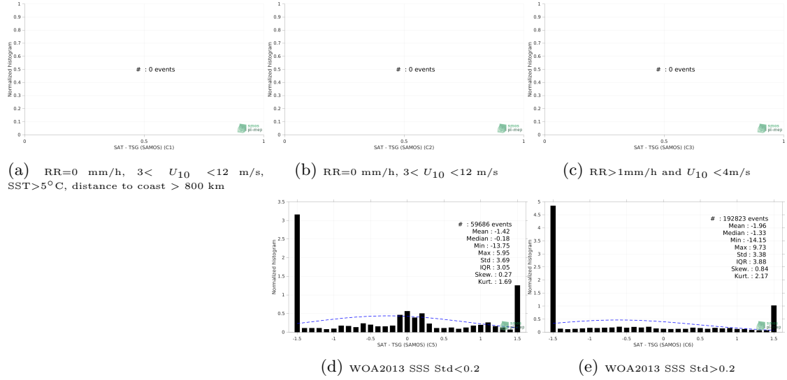
Figure 13: Normalized histogram of \Delta SSS (SMOS SSS L4 v1 - Weekly (CMEMS-CNR) - TSG (SAMOS)) for 5 different subdatasets corresponding to: RR=0 mm/h, 3 < U_{10} < 12 m/s, SST > 5°C, distance to coast > 800 km (a), RR=0 mm/h, 3 < U_{10} < 12 m/s (b), RR > 1mm/h and U_{10} < 4 m/s (c), WOA2013 SSS Std < 0.2 (d), WOA2013 SSS Std > 0.2 (e).
