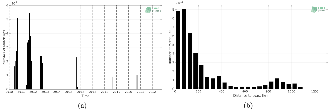
Figure 1: Number of match-ups between TSG (SAMOS) and SMOS SSS L4 v1 - Weekly (CMEMS-CNR) SSS as a function of time (a) and as function of the distance to coast (b) over the Arctic Ocean Pi-MEP region and for the full satellite product period.
