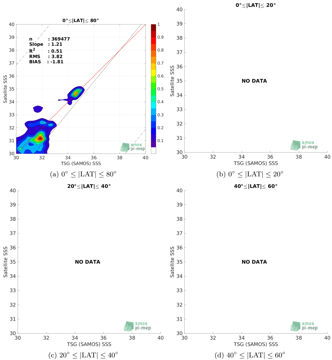
Figure 9: Contour maps of the concentration of SMOS SSS L4 v1 - Weekly (CMEMS-CNR) SSS (y-axis) versus TSG (SAMOS) SSS (x-axis) at match-up pairs for different latitude bands. For each plot, the red line shows x=y . The black thin and dashed lines indicate a linear fit through the data cloud and the \pm 95\% confidence levels, respectively. The number match-up pairs n , the slope and R^2 coefficient of the linear fit, the root mean square (RMS) and the mean bias between satellite and in situ data are indicated for each latitude band in each plots.
