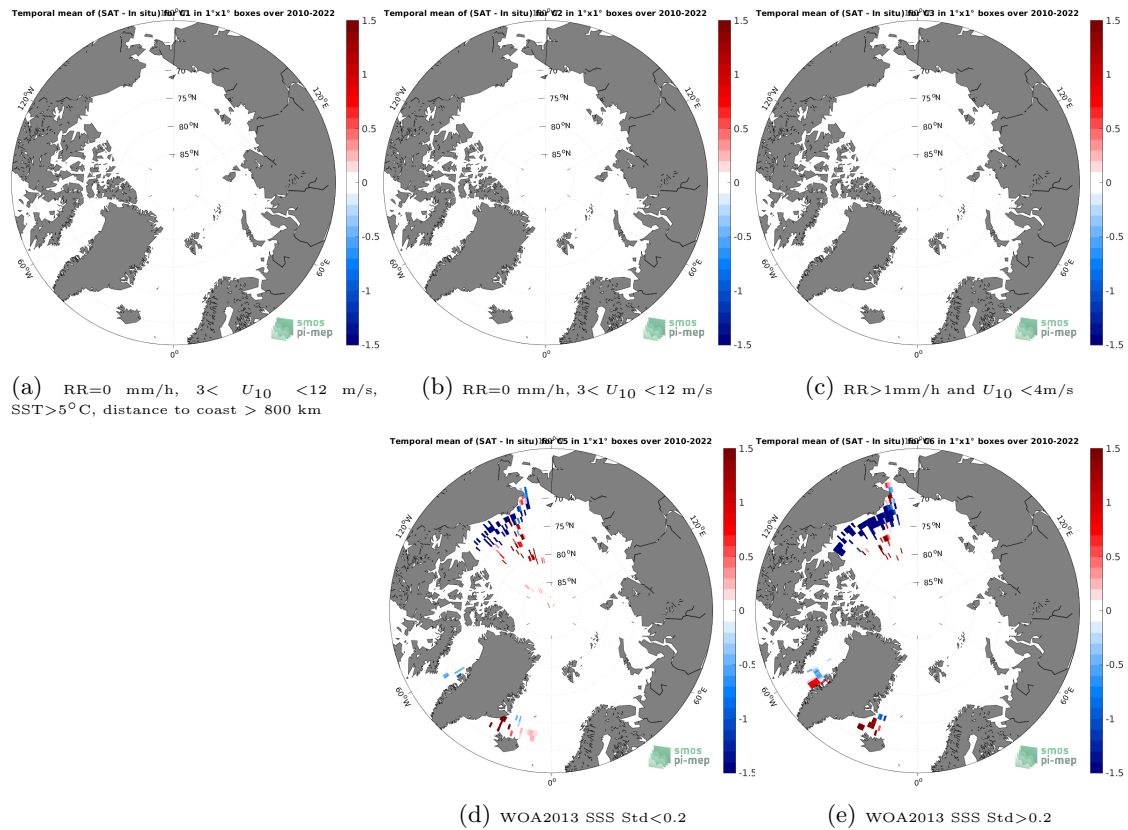
Figure 12: Temporal mean gridded over spatial boxes of size 1^{\circ}\times 1^{\circ} of \Delta\text{SSS} (SMOS SSS L4 v1 - Weekly (CMEMS-CNR) - TSG (SAMOS)) for 5 different subdatasets corresponding to:RR=0 mm/h, 3 < U_{10} < 12 m/s, SST >5^{\circ}\text{C} , distance to coast > 800 km (a), RR=0 mm/h, 3 < U_{10} < 12 m/s (b), RR >1 mm/h and U_{10} < 4 m/s (c), WOA2013 SSS Std <0.2 (d), WOA2013 SSS Std >0.2 (e).
