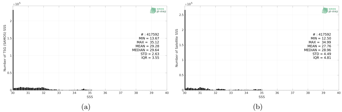
Figure 2: Histograms of SSS from TSG (SAMOS) (a) and SMOS SSS L4 v1 - Weekly (CMEMS-CNR) (b) considering all match-up pairs per bins of 0.1 over the Arctic Ocean Pi-MEP region and for the full satellite product period.
