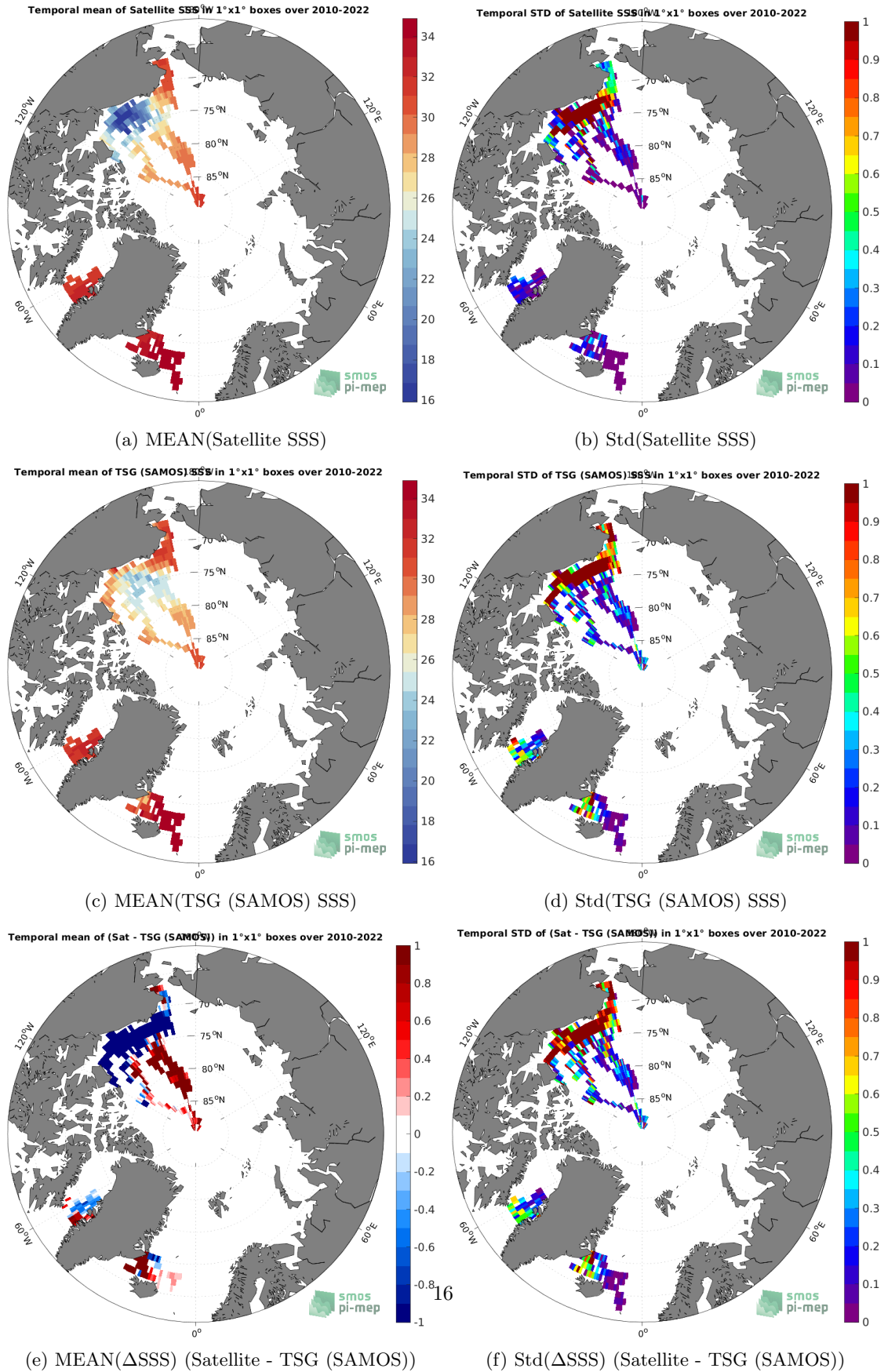
Figure 6: Temporal mean (left) and Std (right) of SSS from SMOS SSS L4 v1 - Weekly (CMEMS-CNR) (top), TSG (SAMOS) (middle), and of \Delta SSS (Satellite - TSG (SAMOS)). Only match-up pairs are used to generate these maps.
