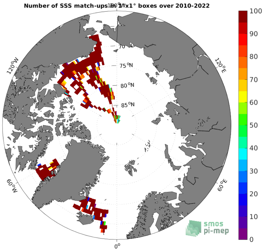
Figure 4: Number of SSS match-ups between TSG (SAMOS) SSS and the SMOS SSS L4 v1 - Weekly (CMEMS-CNR) SSS product for the Arctic Ocean Pi-MEP region over 1^\circ \times 1^\circ boxes and for the full satellite product period.
