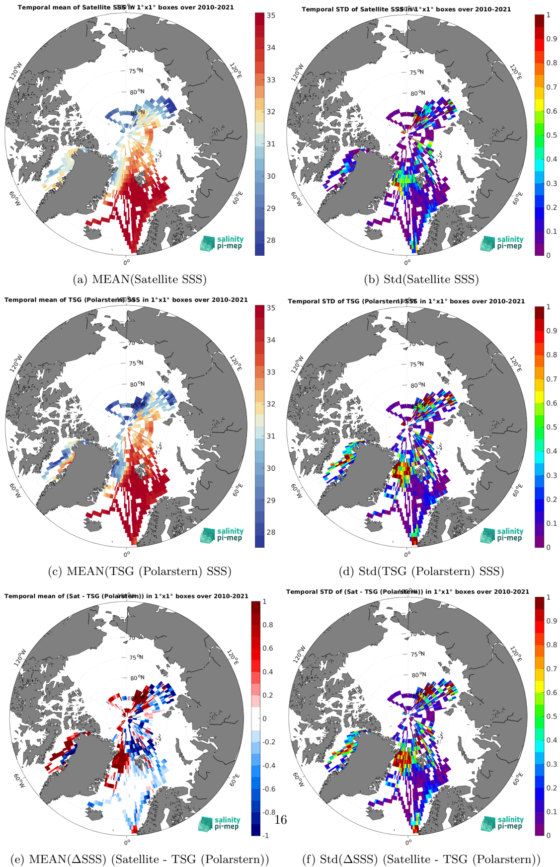
Figure 6: Temporal mean (left) and Std (right) of SSS from SMOS SSS L4 v1 - Weekly (CMEMS-CNR) (top), TSG (Polarstern) (middle), and of \Delta SSS (Satellite - TSG (Polarstern)). Only match-up pairs are used to generate these maps.
