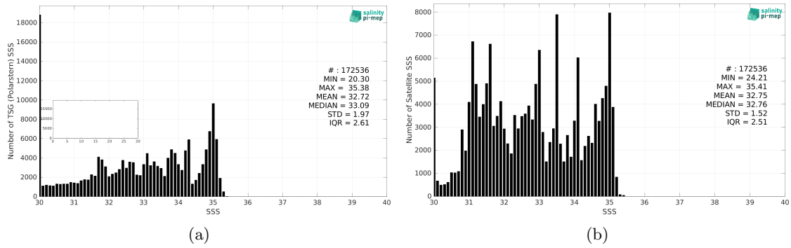
Figure 2: Histograms of SSS from TSG (Polarstern) (a) and SMOS SSS L4 v1 - Weekly (CMEMS-CNR) (b) considering all match-up pairs per bins of 0.1 over the Arctic Ocean Pi-MEP region and for the full satellite product period.
