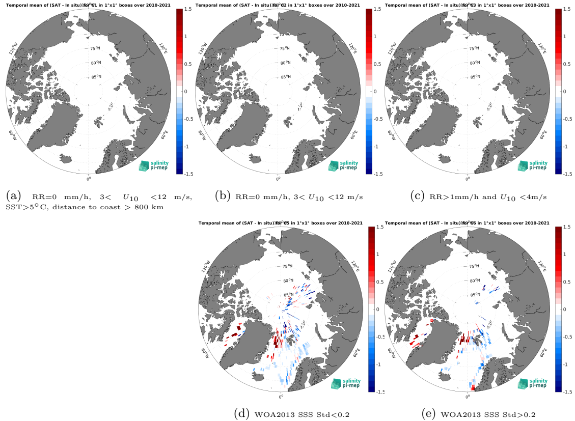
Figure 12: Temporal mean gridded over spatial boxes of size 1^{\circ}\times 1^{\circ} of \Delta\text{SSS} (SMOS SSS L4 v1 - Weekly (CMEMS-CNR) - TSG (Polarstern)) for 5 different subdatasets corresponding to:RR=0 mm/h, 3 < U_{10} < 12 m/s, SST > 5^{\circ}\text{C} , distance to coast > 800 km (a), RR=0 mm/h, 3 < U_{10} < 12 m/s (b), RR > 1 mm/h and U_{10} < 4 m/s (c), WOA2013 SSS Std < 0.2 (d), WOA2013 SSS Std > 0.2 (e).
