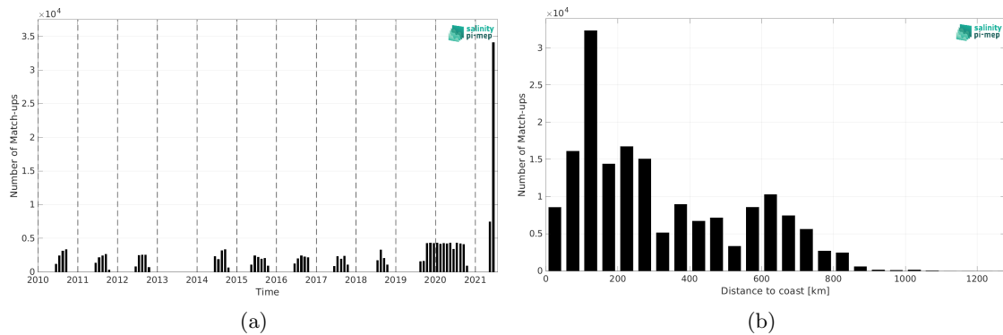
Figure 1: Number of match-ups between TSG (Polarstern) and SMOS SSS L4 v1 - Weekly (CMEMS-CNR) SSS as a function of time (a) and as function of the distance to coast (b) over the Arctic Ocean Pi-MEP region and for the full satellite product period.
