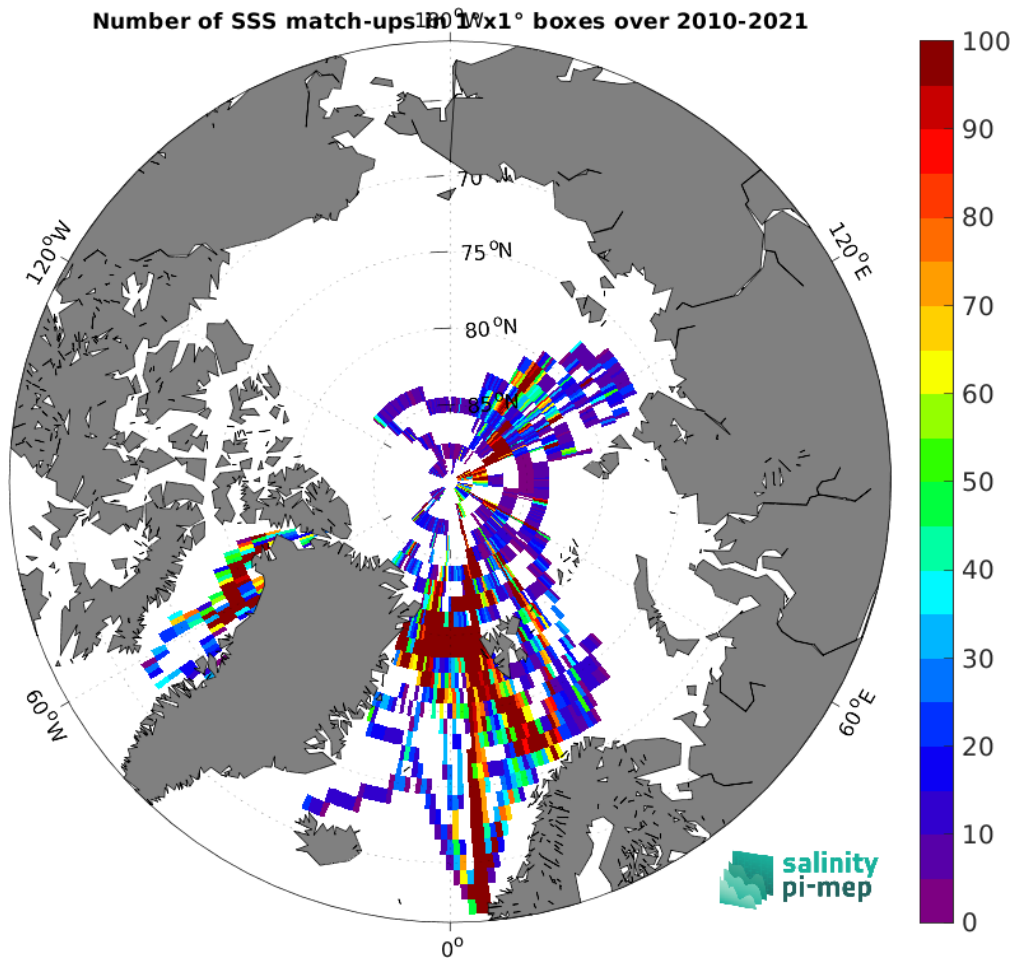
Figure 4: Number of SSS match-ups between TSG (Polarstern) SSS and the SMOS SSS L4 v1 - Weekly (CMEMS-CNR) SSS product for the Arctic Ocean Pi-MEP region over 1^\circ \times 1^\circ boxes and for the full satellite product period.
