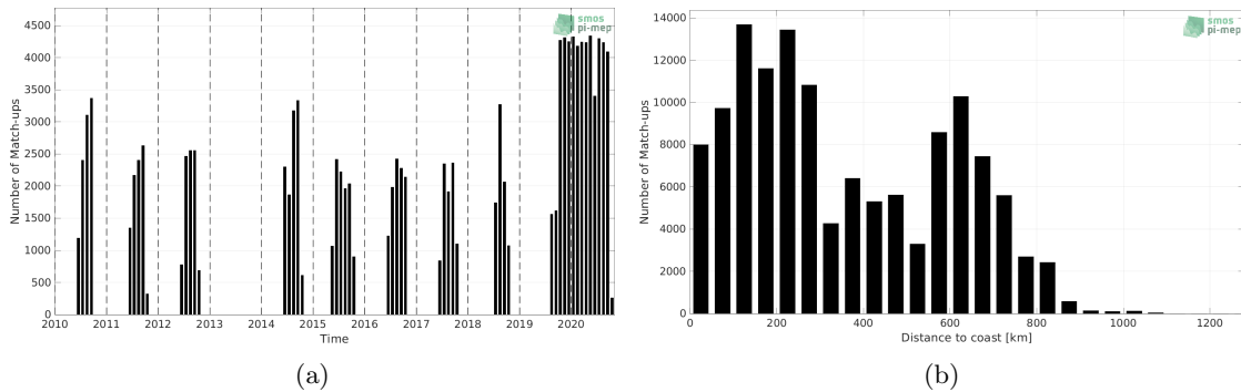
Figure 1: Number of match-ups between TSG (Polarstern) and SMOS SSS L4 v1 - Weekly (CMEMS-CNR) SSS as a function of time (a) and as function of the distance to coast (b) over the Arctic Ocean Pi-MEP region and for the full satellite product period.
