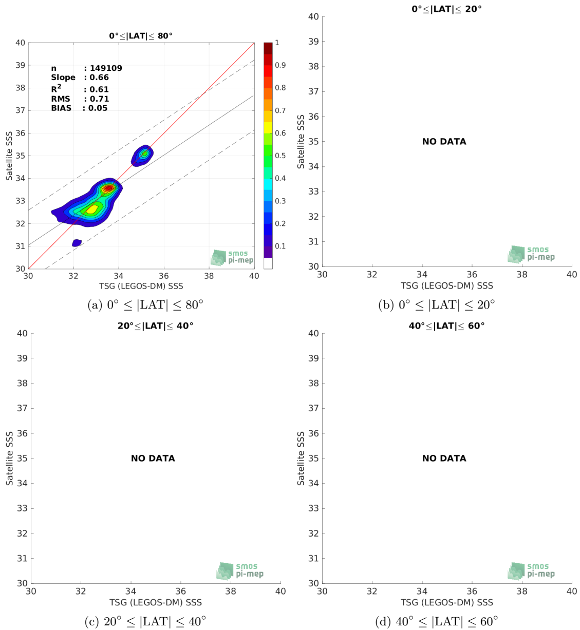
Figure 9: Contour maps of the concentration of SMOS SSS L4 v1 - Weekly (CMEMS-CNR) SSS (y-axis) versus TSG (LEGOS-DM) SSS (x-axis) at match-up pairs for different latitude bands. For each plot, the red line shows x=y . The black thin and dashed lines indicate a linear fit through the data cloud and the \pm 95\% confidence levels, respectively. The number match-up pairs n , the slope and R^2 coefficient of the linear fit, the root mean square (RMS) and the mean bias between satellite and in situ data are indicated for each latitude band in each plots.
