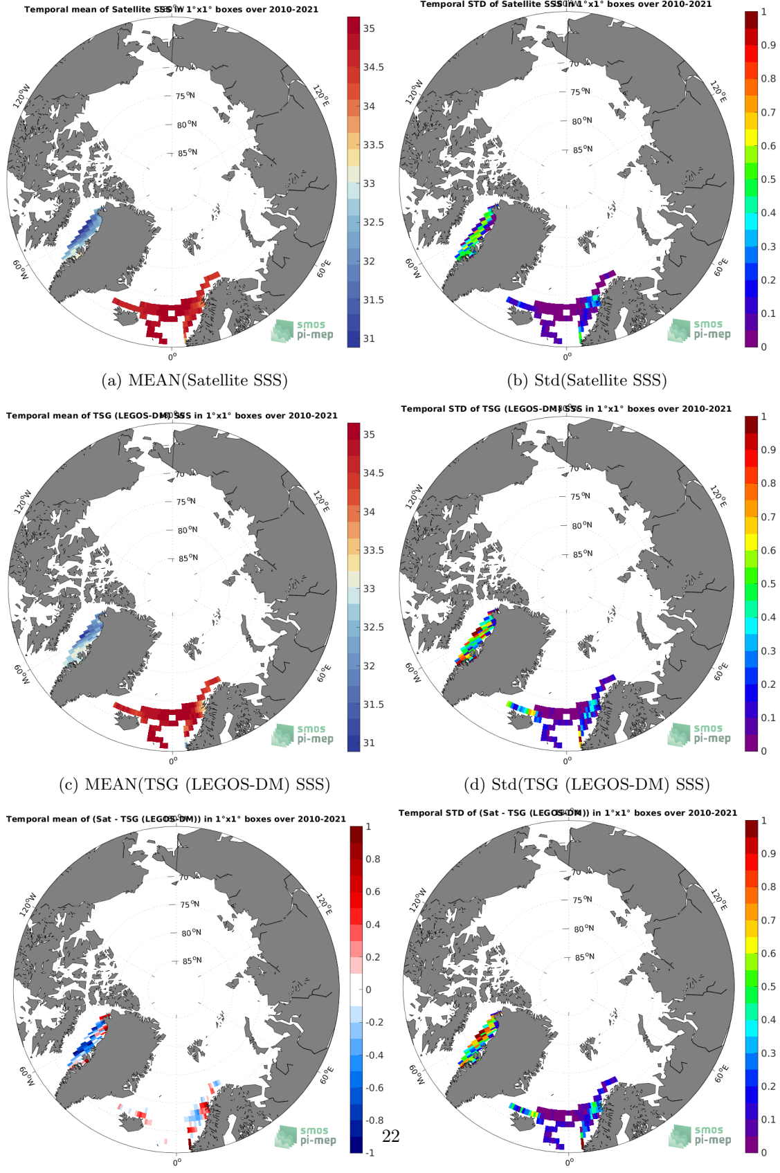
Figure 6: Temporal mean (left) and Std (right) of SSS from SMOS SSS L4 v1 - Weekly (CMEMS-CNR) (top), TSG (LEGOS-DM) (middle), and of \Delta SSS (Satellite - TSG (LEGOS-DM)). Only match-up pairs are used to generate these maps.
