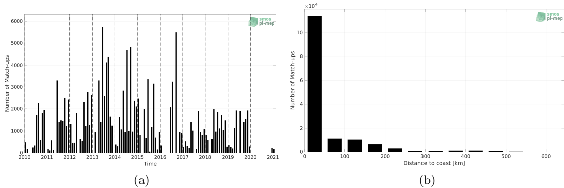
Figure 1: Number of match-ups between TSG (LEGOS-DM) and SMOS SSS L4 v1 - Weekly (CMEMS-CNR) SSS as a function of time (a) and as function of the distance to coast (b) over the Arctic Ocean Pi-MEP region and for the full satellite product period.
