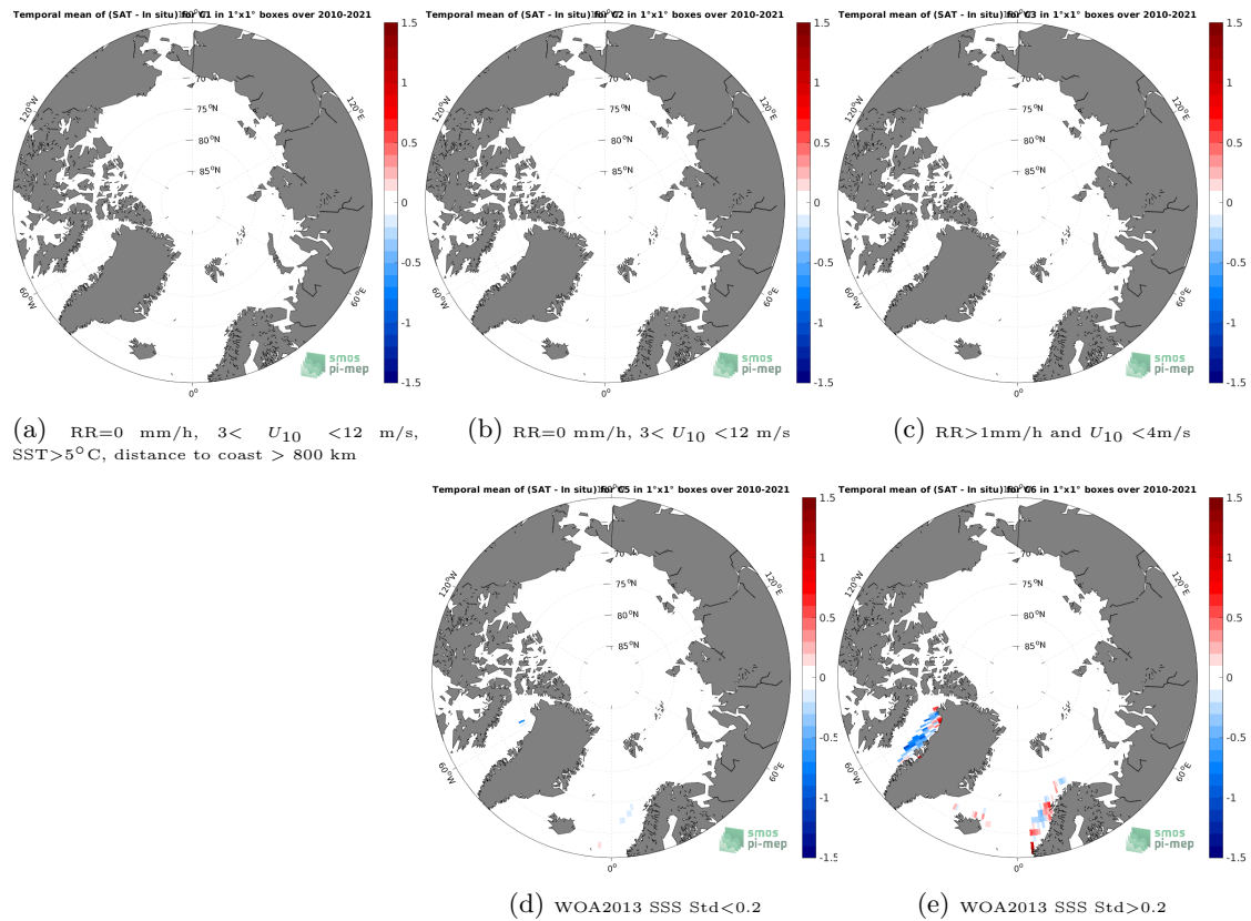
Figure 12: Temporal mean gridded over spatial boxes of size 1^{\circ}\times 1^{\circ} of \Delta\text{SSS} (SMOS SSS L4 v1 - Weekly (CMEMS-CNR) - TSG (LEGOS-DM)) for 5 different subdatasets corresponding to: RR=0 mm/h, 3 < U_{10} < 12 m/s, SST > 5^{\circ}\text{C} , distance to coast > 800 km (a), RR=0 mm/h, 3 < U_{10} < 12 m/s (b), RR > 1 mm/h and U_{10} < 4 m/s (c), WOA2013 SSS Std < 0.2 (d), WOA2013 SSS Std > 0.2 (e).
