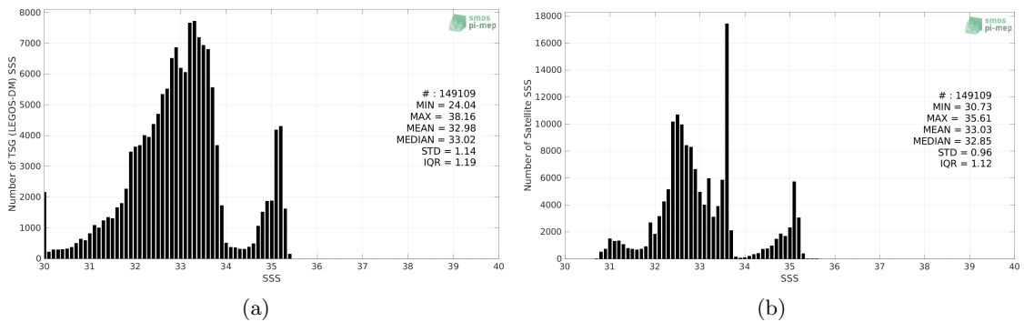
Figure 2: Histograms of SSS from TSG (LEGOS-DM) (a) and SMOS SSS L4 v1 - Weekly (CMEMS-CNR) (b) considering all match-up pairs per bins of 0.1 over the Arctic Ocean Pi-MEP region and for the full satellite product period.
