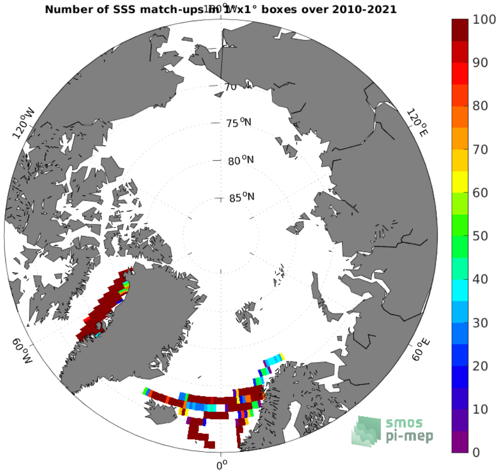
Figure 4: Number of SSS match-ups between TSG (LEGOS-DM) SSS and the SMOS SSS L4 v1 - Weekly (CMEMS-CNR) SSS product for the Arctic Ocean Pi-MEP region over 1^\circ \times 1^\circ boxes and for the full satellite product period.
