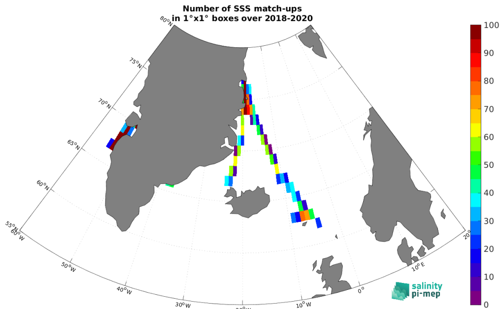
Figure 4: Number of SSS match-ups between TSG (Lauge-Koch) SSS and the SMOS SSS L4 v1 - Weekly (CMEMS-CNR) SSS product for the Arctic Ocean Pi-MEP region over 1^\circ \times 1^\circ boxes and for the full satellite product period.
