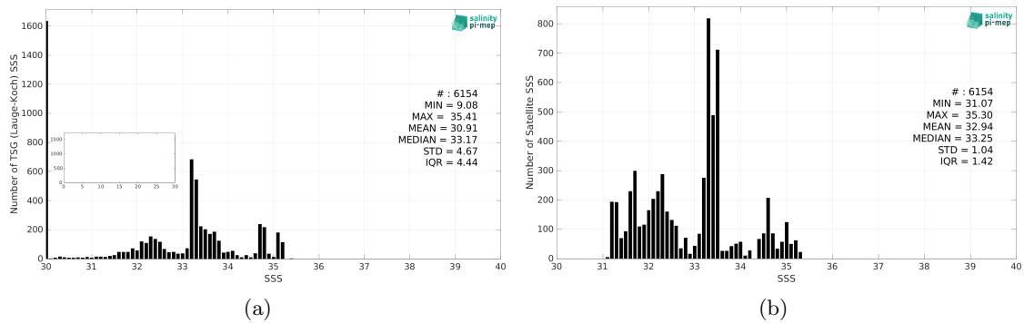
Figure 2: Histograms of SSS from TSG (Lauge-Koch) (a) and SMOS SSS L4 v1 - Weekly (CMEMS-CNR) (b) considering all match-up pairs per bins of 0.1 over the Arctic Ocean Pi-MEP region and for the full satellite product period.
