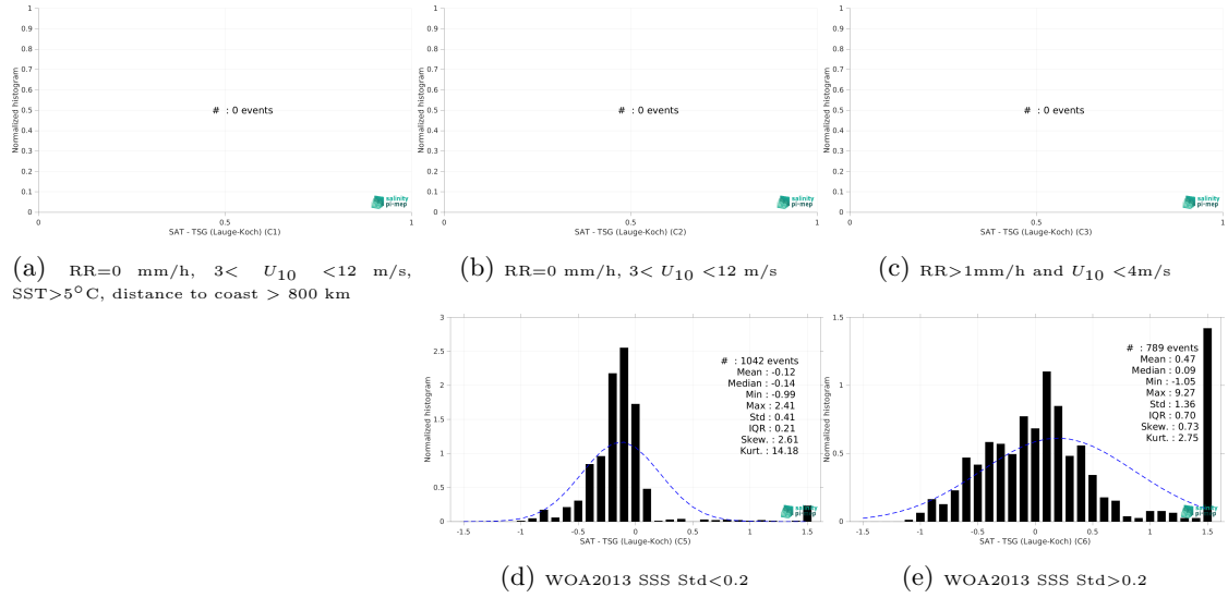
Figure 13: Normalized histogram of \Delta SSS (SMOS SSS L4 v1 - Weekly (CMEMS-CNR) - TSG (Laue-Koch)) for 5 different subdatasets corresponding to: RR=0 mm/h, 3 < U_{10} < 12 m/s, SST > 5°C, distance to coast > 800 km (a), RR=0 mm/h, 3 < U_{10} < 12 m/s (b), RR > 1mm/h and U_{10} < 4 m/s (c), WOA2013 SSS Std < 0.2 (d), WOA2013 SSS Std > 0.2 (e).
