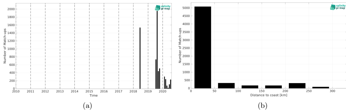
Figure 1: Number of match-ups between TSG (Lauge-Koch) and SMOS SSS L4 v1 - Weekly (CMEMS-CNR) SSS as a function of time (a) and as function of the distance to coast (b) over the Arctic Ocean Pi-MEP region and for the full satellite product period.
